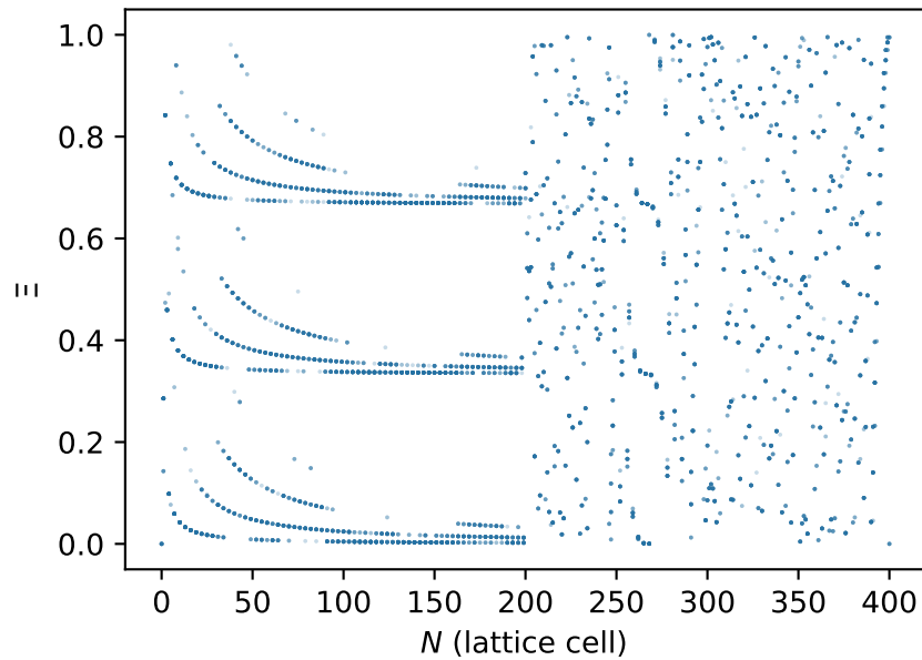
Cubic kernel: lattice at thirds
