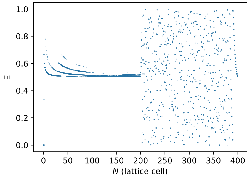
Quadratic kernel: atoms lie on smooth curves
