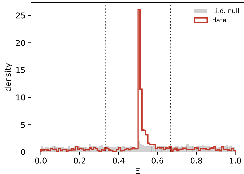
Tent map, quadratic kernel S_2 , K = 400
