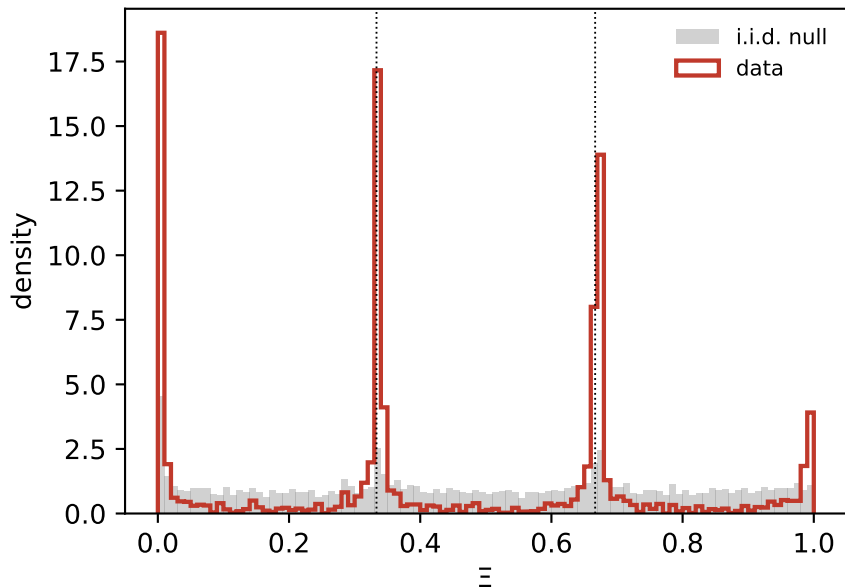
Lorenz x, cubic kernel S_3 , K = 100
