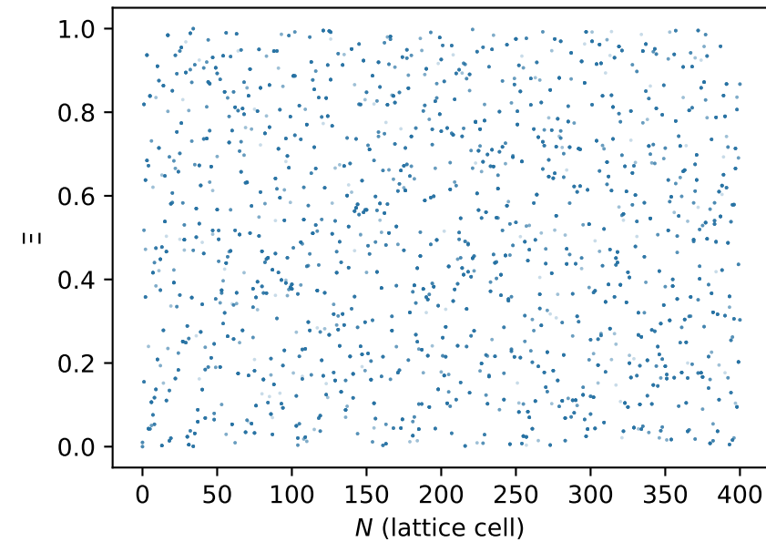
Hash kernel: arithmetic structure destroyed
