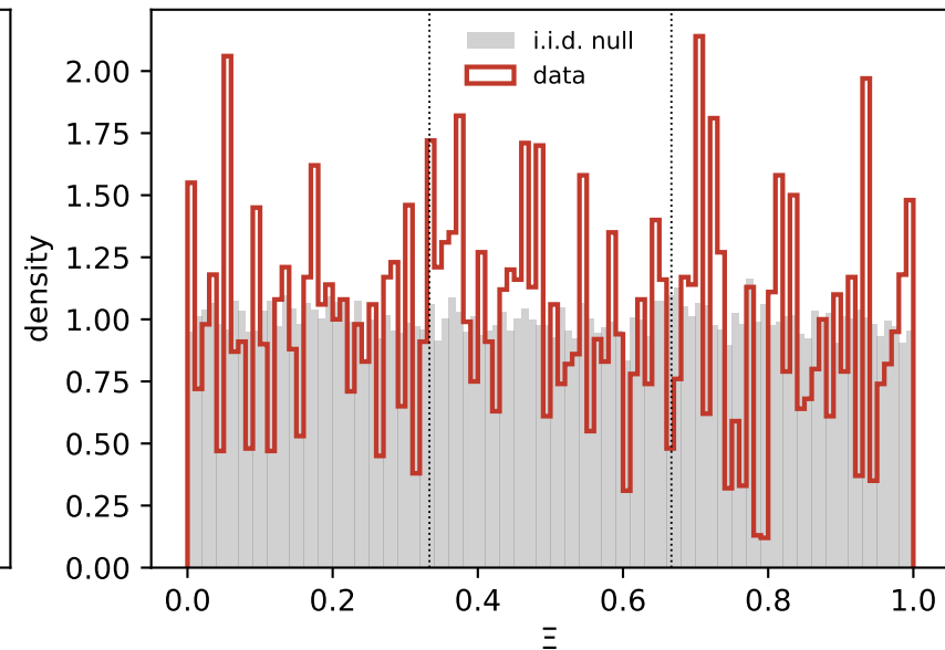
Tent map, pseudorandom hash, K = 200
