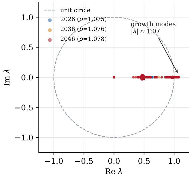
(a) Spectrum of the one-year map
