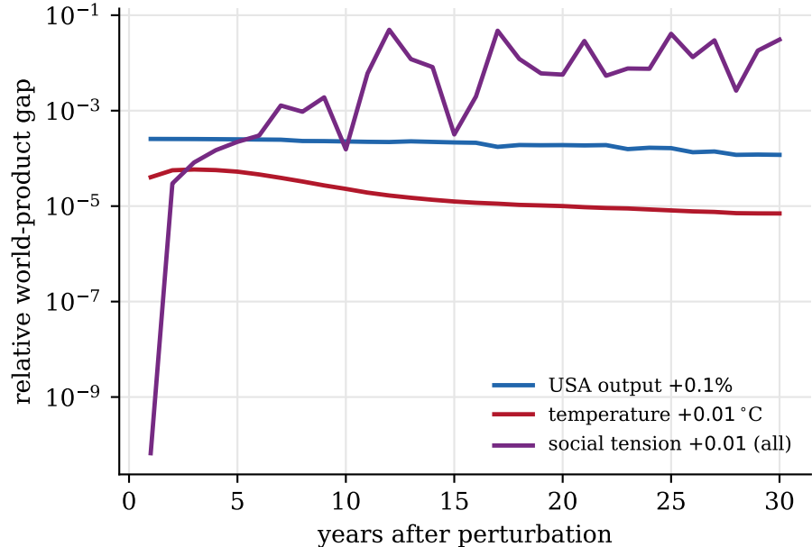
(b) Perturbations: contraction vs. slow social memory
