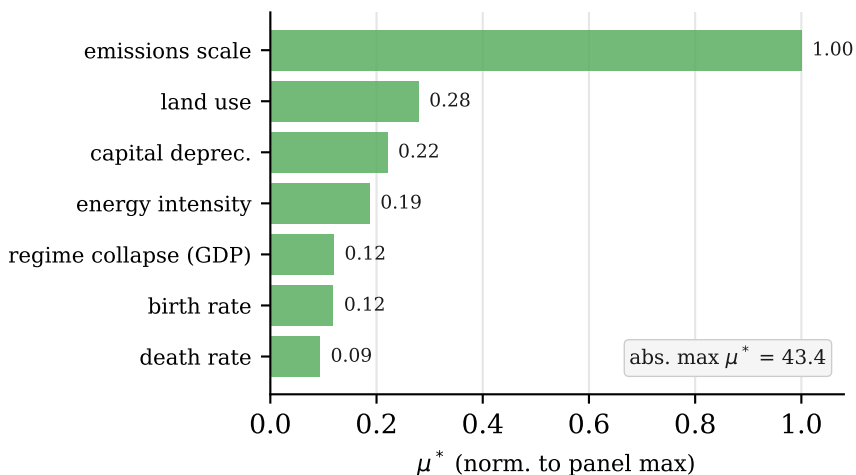
CO 2 emissions
