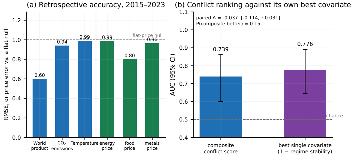
Figure 4: Retrospective anchor. (a) In-sample error 2015–2023 in two different units on one axis, as labelled: world product (trillion USD), emissions (Gt) and temperature (in units of 0.1^\circ\text{C} , so the plotted 0.99 is 0.099^\circ\text{C} ) at left; the three resource prices at right, scored as the ratio to the error a no-skill flat price makes, so the dashed line at unity is that null and below it is better. (b) Conflict ranking against the benchmark that decides it — not chance, but the composite’s own best single input. Bars are AUC with 95% bootstrap intervals; the paired difference and the probability that the composite is the better ranker are inset (score inputs at 2023 base-year values; the vintage-clean variant is given in the text).
