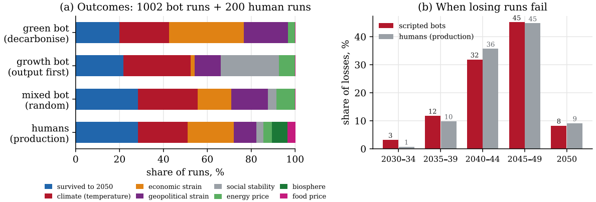
Figure 6: The tail census: 1,002 scripted playthroughs and 200 completed human runs (of 401 started; completer statistics shown, an upper bound under the stated attrition assumption), 2023–2050. (a) Outcome composition by archetype and for human players: no doctrine dominates, each dies of its characteristic cause, and the human loss spectrum is broader (biosphere and food-price tails the bots rarely hit). (b) Timing of failures, bots vs. humans: both distributions peak in 2040–2049 as slow accumulators come due.
