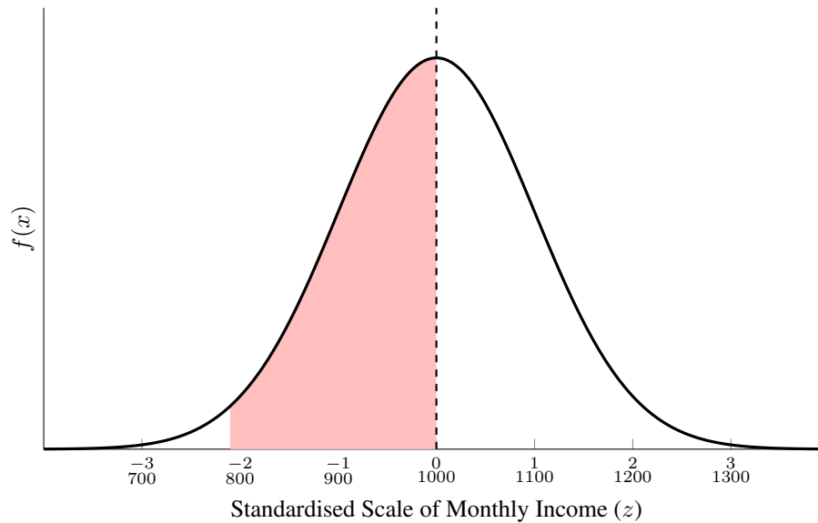
Figure 7.17: Standard Normal Distribution of Income
