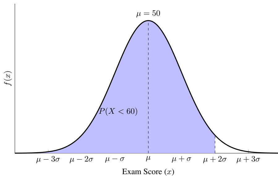
Figure 7.8: The Normal Distribution
