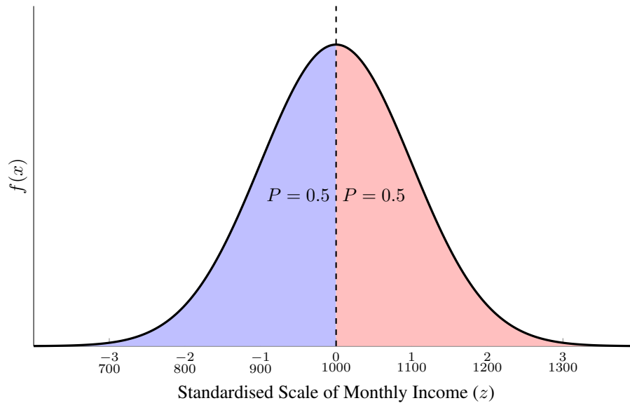
Figure 7.12: Standard Normal Distribution of Income
