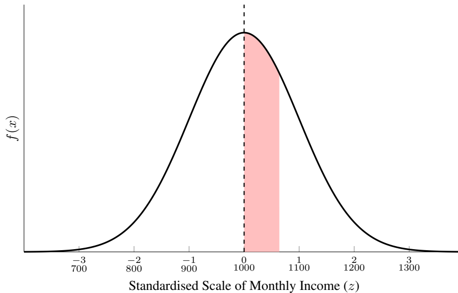
Figure 7.14: Standard Normal Distribution of Income
