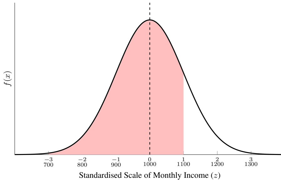
Figure 7.15: Standard Normal Distribution of Income
