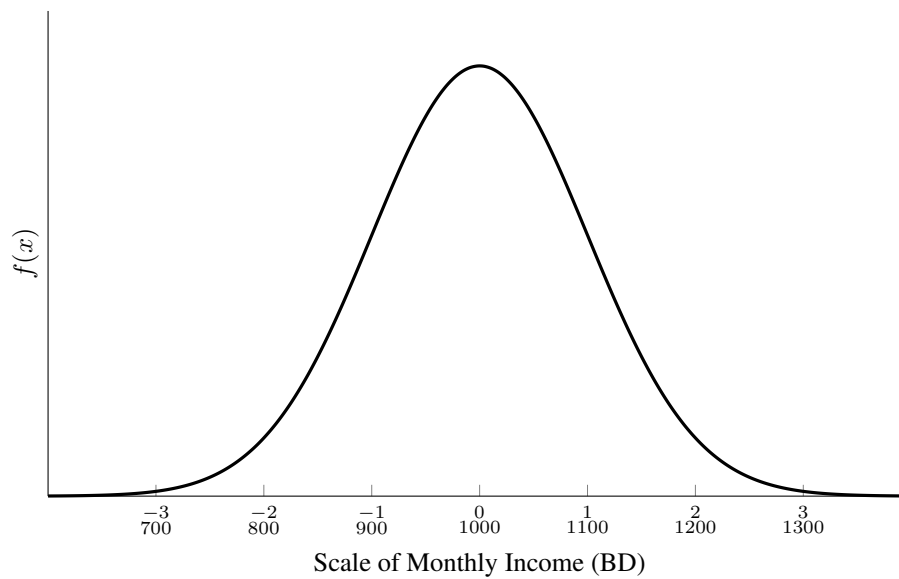
Figure 7.11: Standard Normal Distribution of Income
