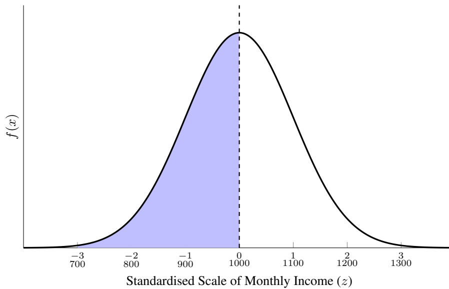
Figure 7.18: Standard Normal Distribution of Income
