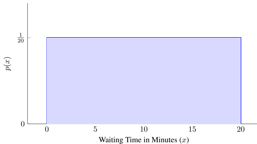
Figure 7.5: Uniform Distribution of Passenger Waiting Time
