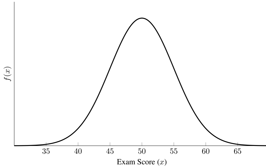
Figure 7.7: The Normal Distribution
