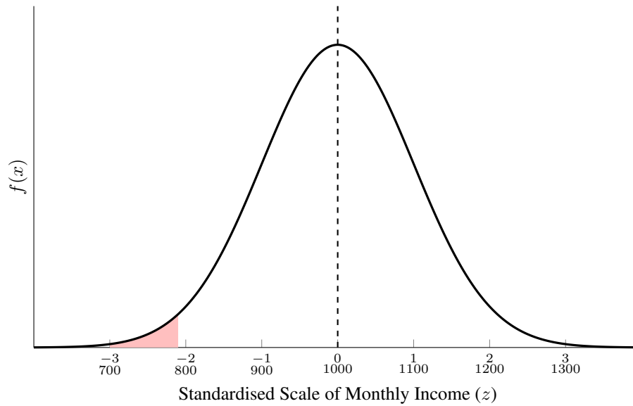
Figure 7.19: Standard Normal Distribution of Income
