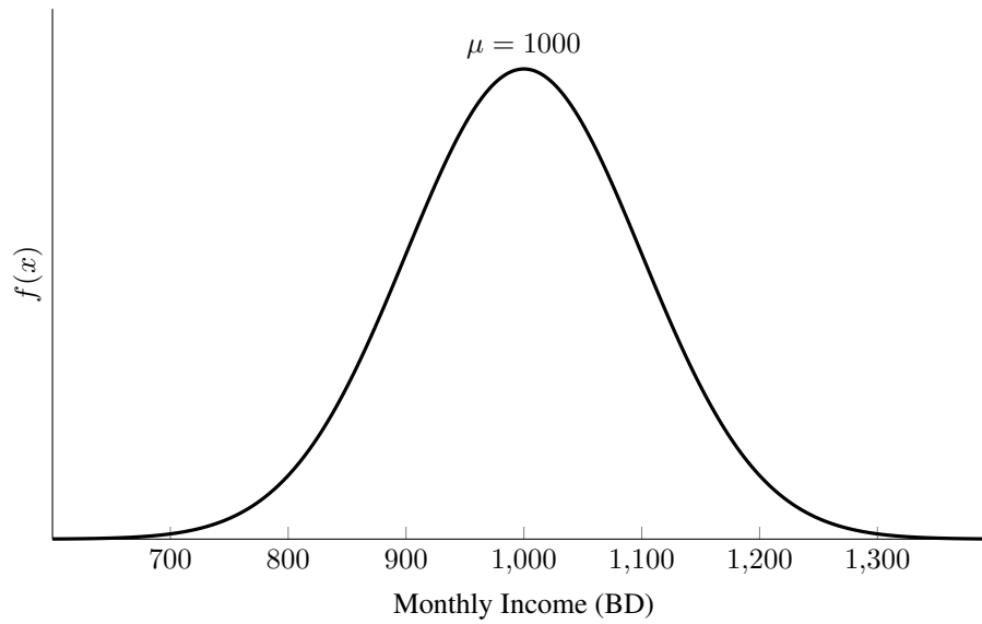
Figure 7.10: Normal Distribution of Monthly Income
