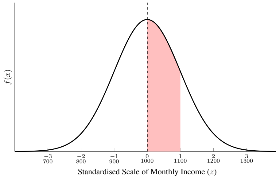
Figure 7.13: Standard Normal Distribution of Income
