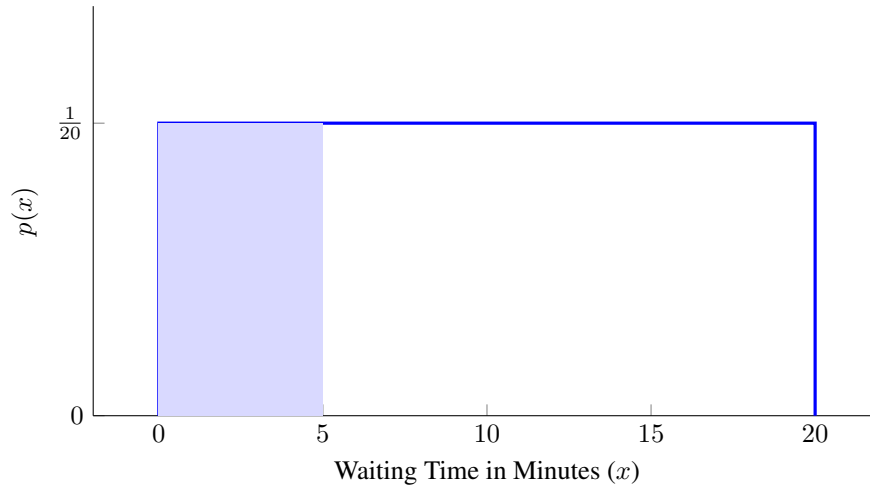
Figure 7.4: Uniform Distribution of Passenger Waiting Time
