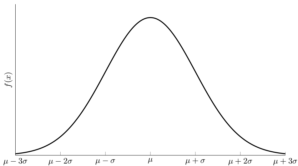
Figure 7.6: The Normal Distribution
