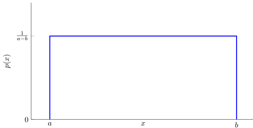
Figure 7.1: Uniform Distribution of Variable X
