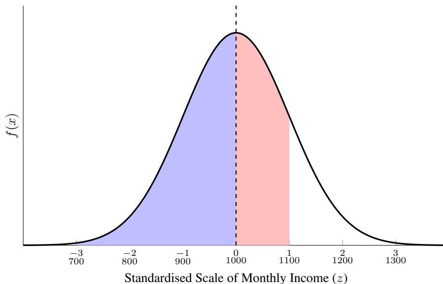
Figure 7.16: Standard Normal Distribution of Income
