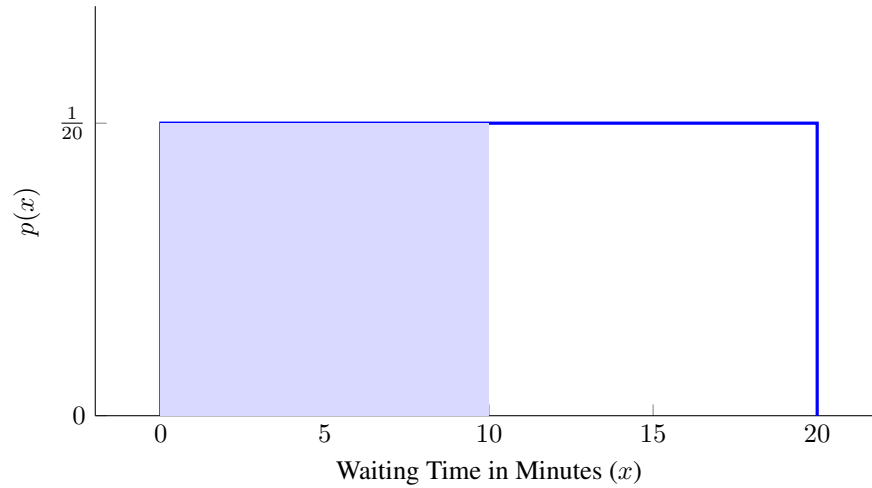
Figure 7.3: Uniform Distribution of Passenger Waiting Time
