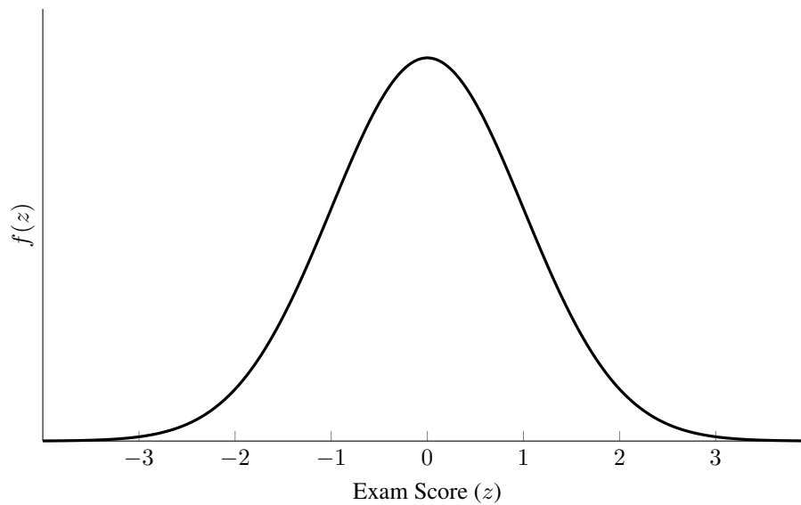
Figure 7.9: The Standard Normal Distribution
