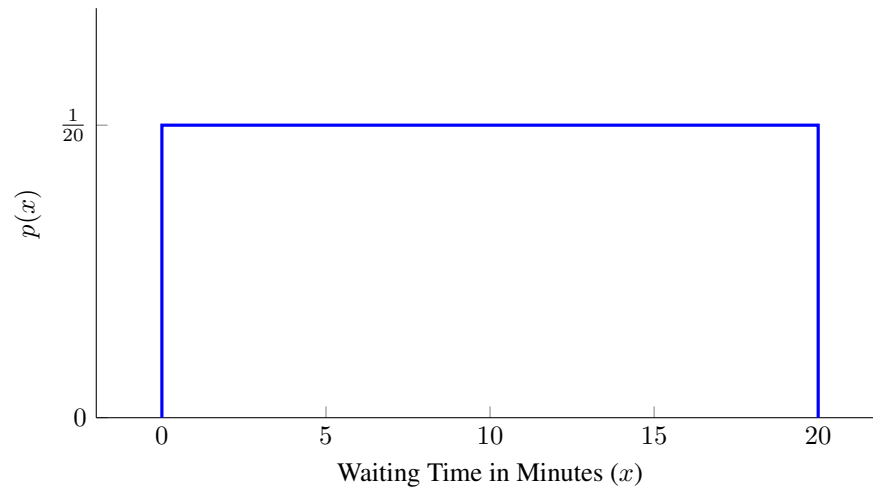
Figure 7.2: Uniform Distribution of Passenger Waiting Time
