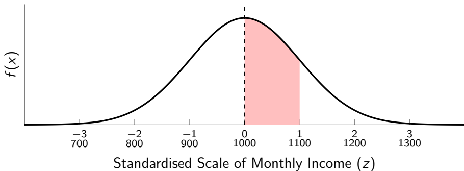
Figure 13: Standard Normal Distribution of Income
