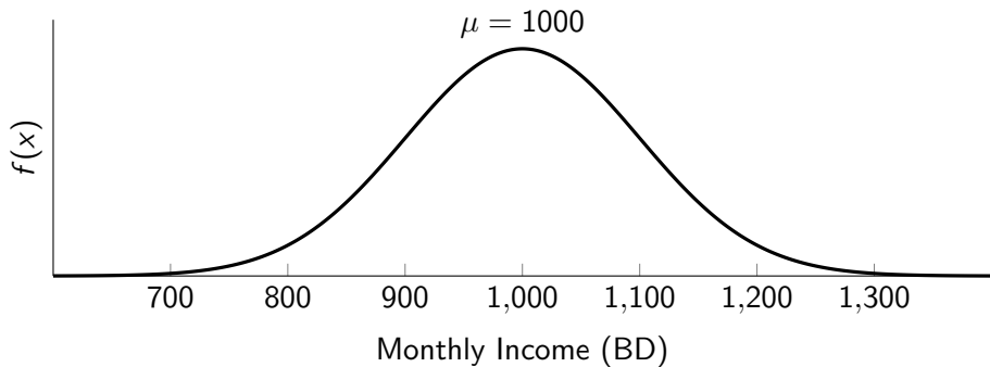
Figure 10: Normal Distribution of Monthly Income
