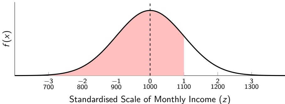
Figure 15: Standard Normal Distribution of Income
