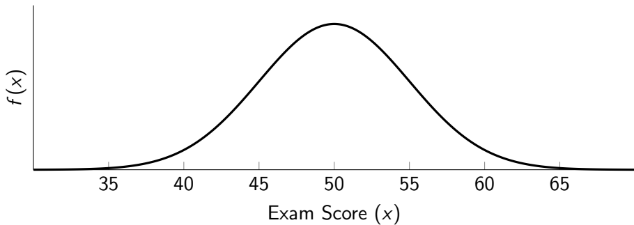
Figure 7: The Normal Distribution
