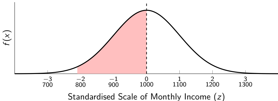
Figure 17: Standard Normal Distribution of Income
