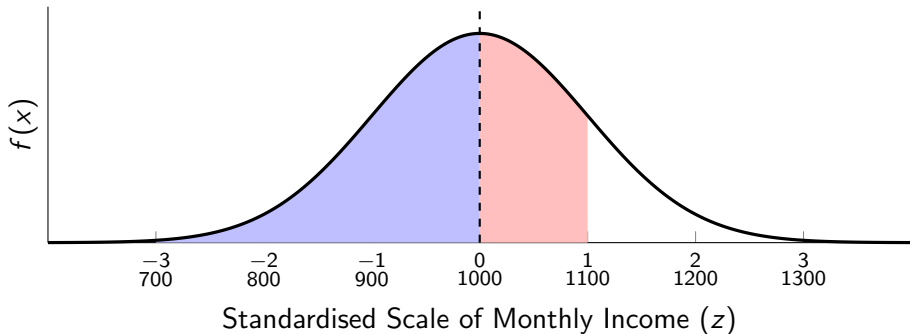
Figure 16: Standard Normal Distribution of Income
