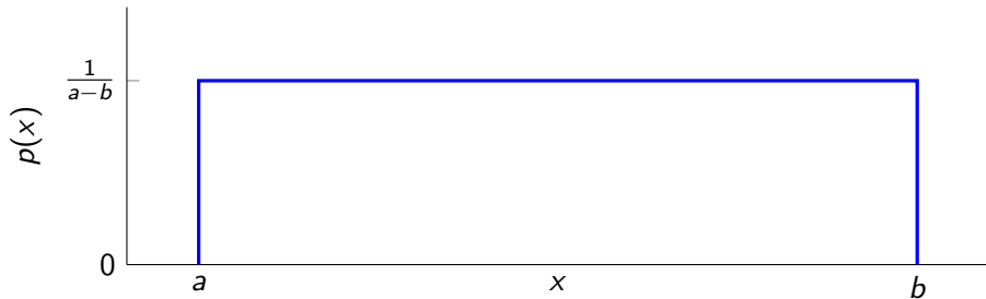
Figure 1: Uniform Distribution of Variable X
