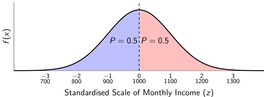
Figure 12: Standard Normal Distribution of Income
