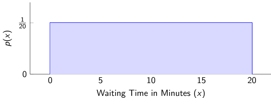
Figure 5: Uniform Distribution of Passenger Waiting Time
