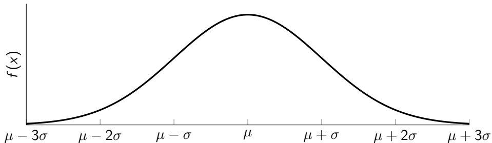
Figure 6: The Normal Distribution
