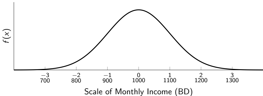
Figure 11: Standard Normal Distribution of Income
