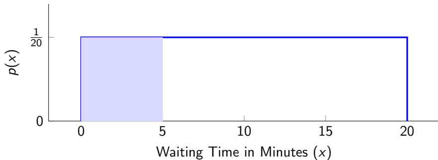
Figure 4: Uniform Distribution of Passenger Waiting Time
