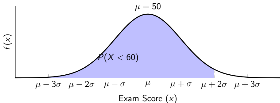
Figure 8: The Normal Distribution
