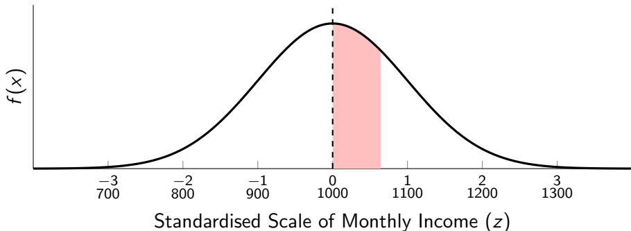
Figure 14: Standard Normal Distribution of Income
