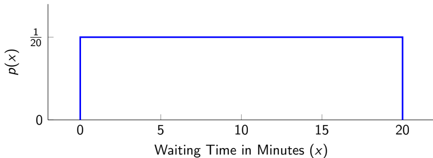
Figure 2: Uniform Distribution of Passenger Waiting Time
