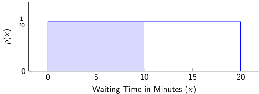
Figure 3: Uniform Distribution of Passenger Waiting Time
