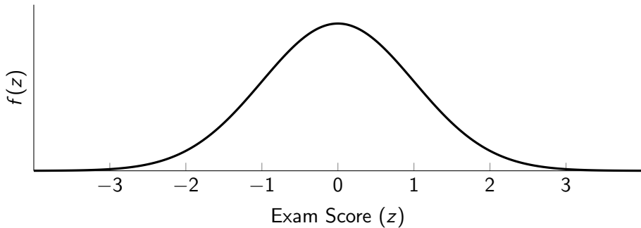
Figure 9: The Standard Normal Distribution
