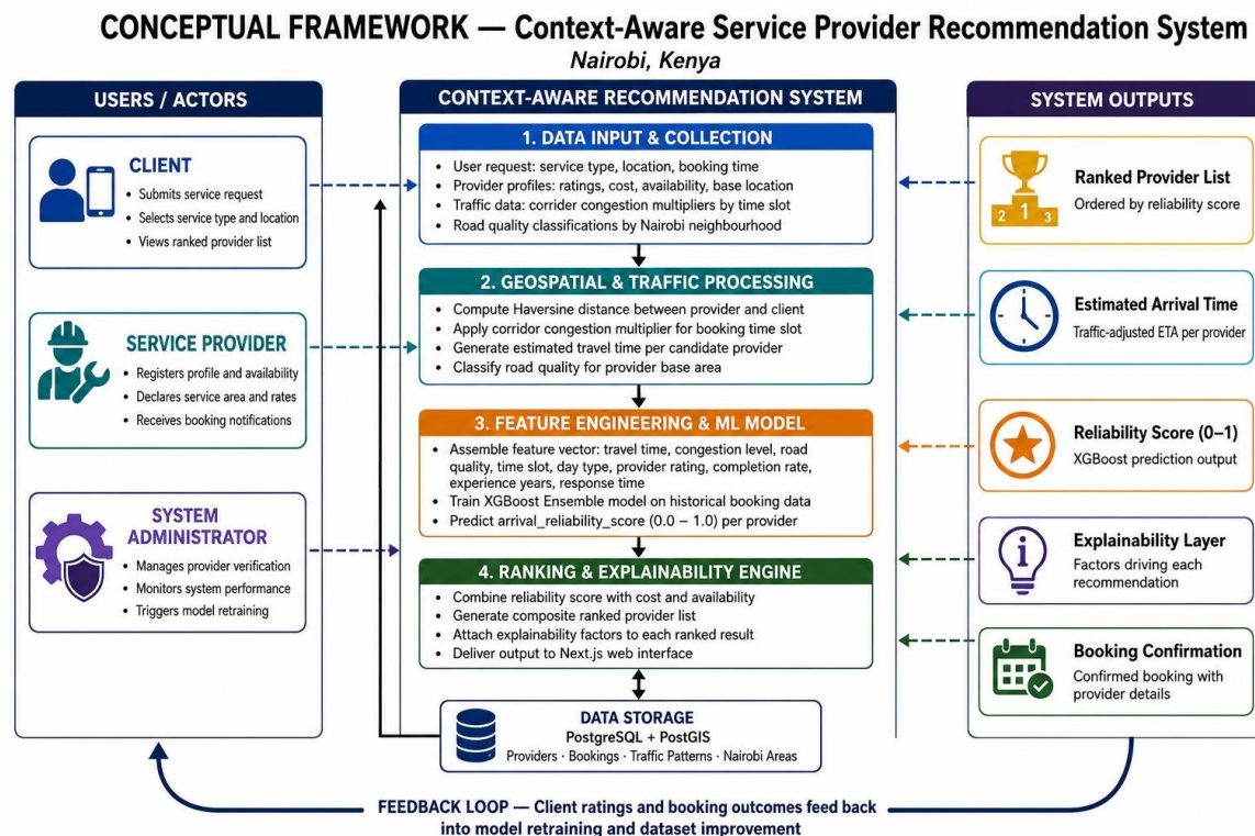
Figure 2.5.4 Conceptual Framework
