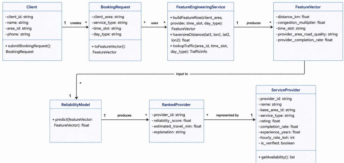
Service Recommender System – Class Diagram
