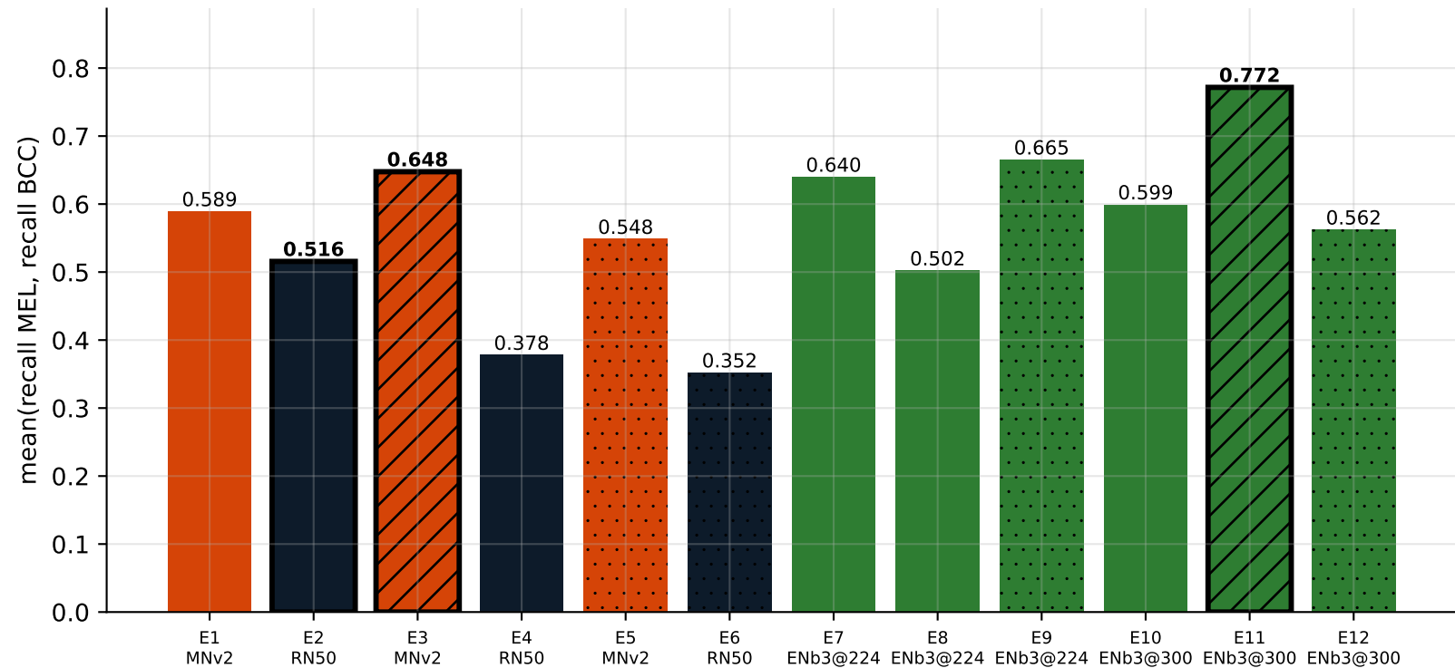
RQ2 selection criterion. Outlined bar is the best run for that architecture.
