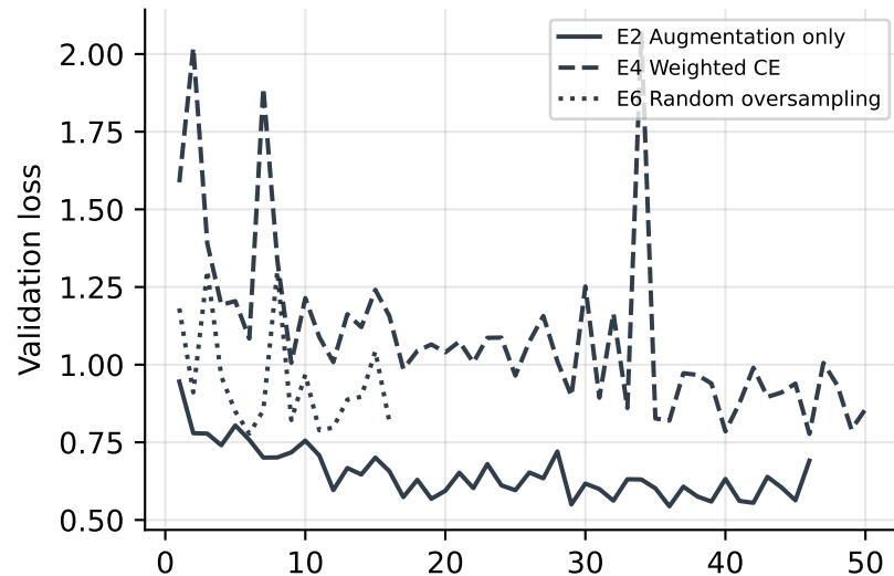
ResNet-50
