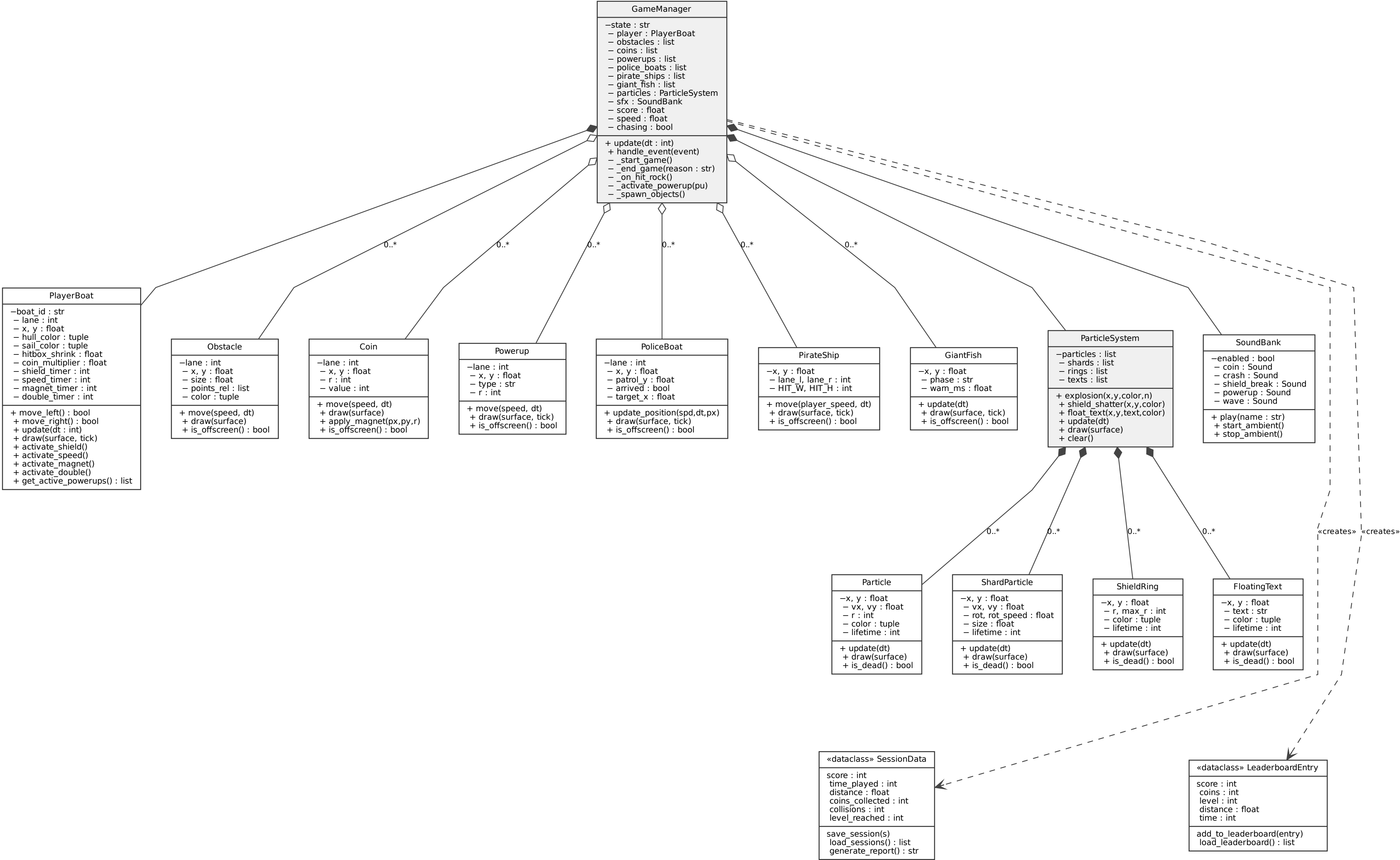
Pirate Escape — UML Class Diagram
