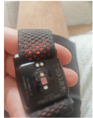
(b) Coospo HW9 (upper-arm sensor)
