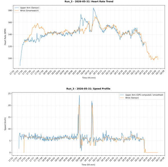
Figure 1: Comparison of heart rate kinetics (top) and velocity profiles (bottom) during Trial 3. The upper-arm sensor (blue) captures dynamic peaks, whereas the wrist sensor (orange) exhibits latency and data omissions.
