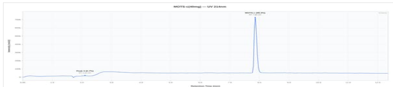
MOTS-C 40mg - MS47010: UV Chromatogram
