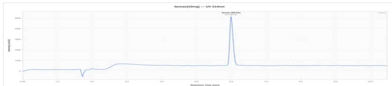
Semax 10mg - XA17010: UV Chromatogram
