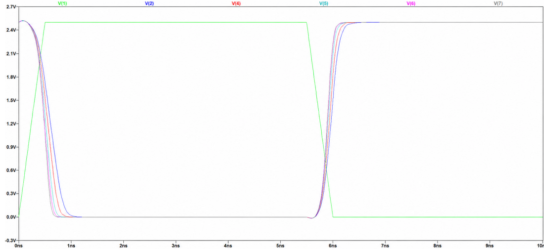
Figure 1: Transient Response of the Inverter for different values of W_n, W_p V
