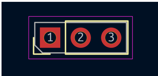
Figure 4.21: JST-XH 1x3
