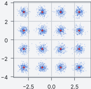
16-QAM, 4000 symbols
