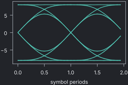
eye diagram, 300 traces at 8% opacity
