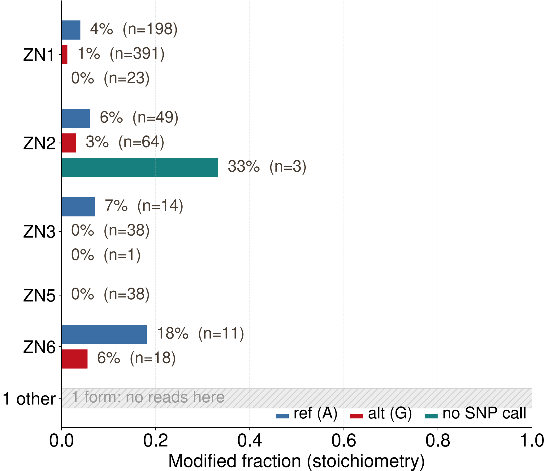
ALCAM chr3:105534693 (a) — per-fragmentform stoichiometry, split by SNP allele
