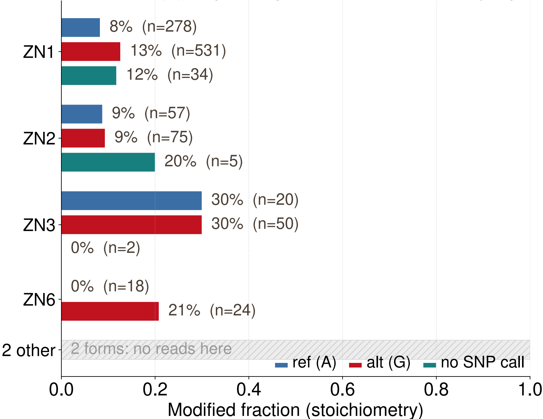
ALCAM chr3:105575839 (a) — per-fragmentform stoichiometry, split by SNP allele
