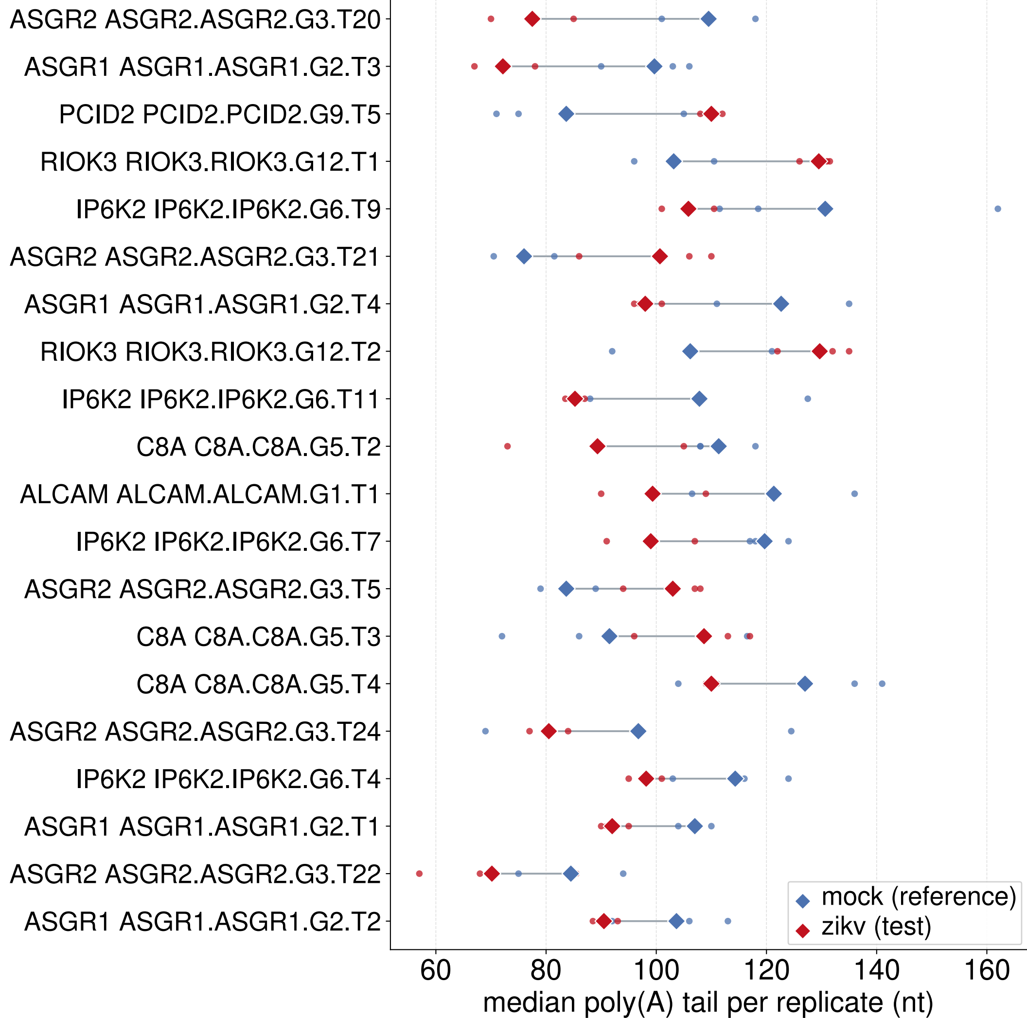
Differential poly(A) tail length — top 20 by effect size
