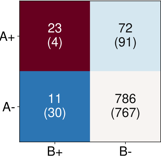
ASGR2 ax19229 d=1bp OR=49.9
