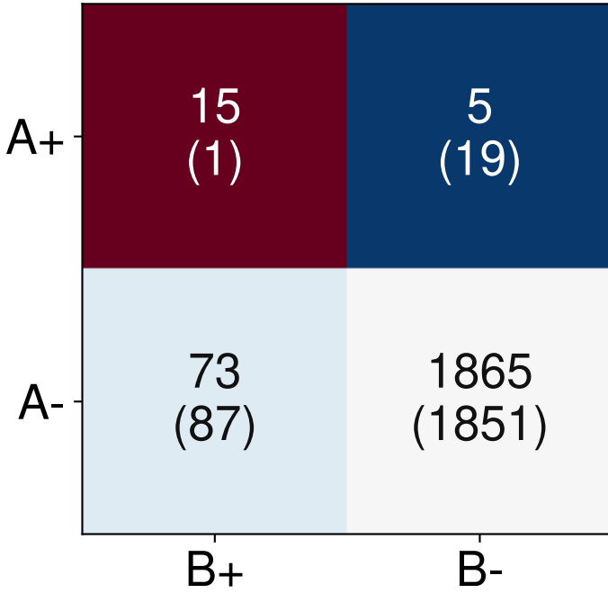
PCID2 ax17596 d=141bp OR=67.2
