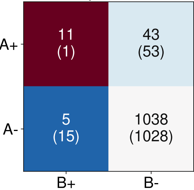
PCID2 axa d=14bp OR=38.3
