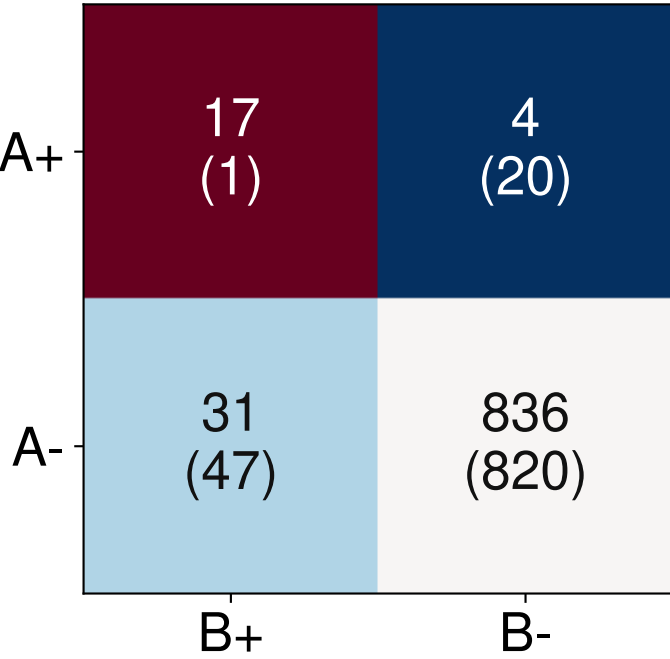
PCID2 axa d=384bp OR=53.4
