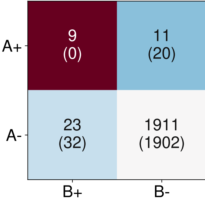
PCID2 ax17596 d=64bp OR=19.4
