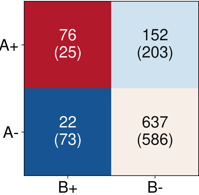
ASGR1 mxa d=1bp OR=22.2
