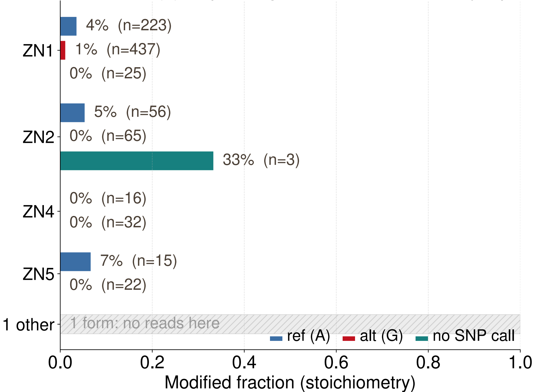
ALCAM chr3:105547247 (a) — per-fragmentform stoichiometry, split by SNP allele
