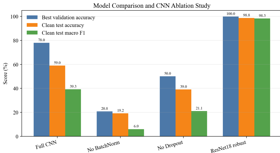
Figure 1. Model comparison and CNN ablation study.
