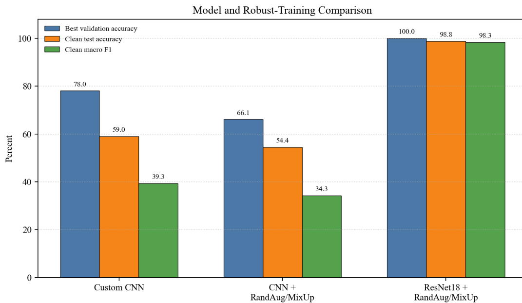
Figure 1. Custom CNN, robustly trained CNN, and robustly trained ResNet18 comparison.
