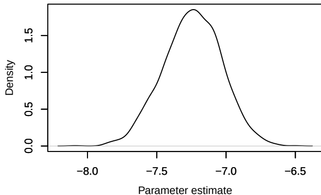
Density – loglik[283]
