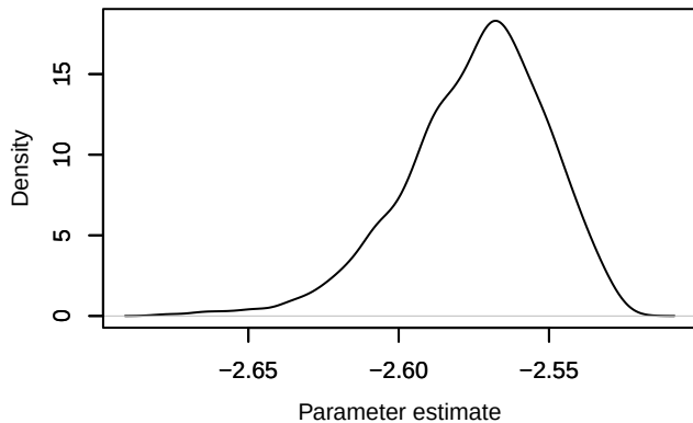
Density – loglik[342]
