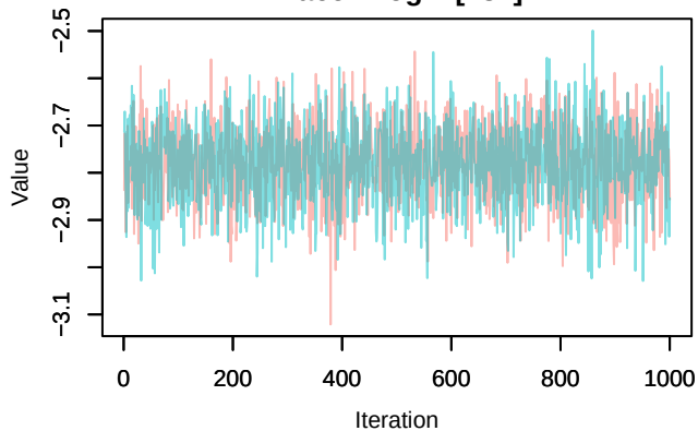
Trace – loglik[282]
