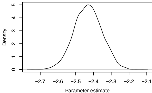
Density – loglik[274]
