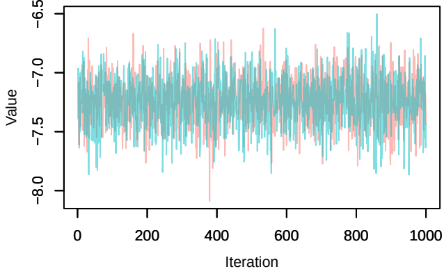
Trace – loglik[148]
