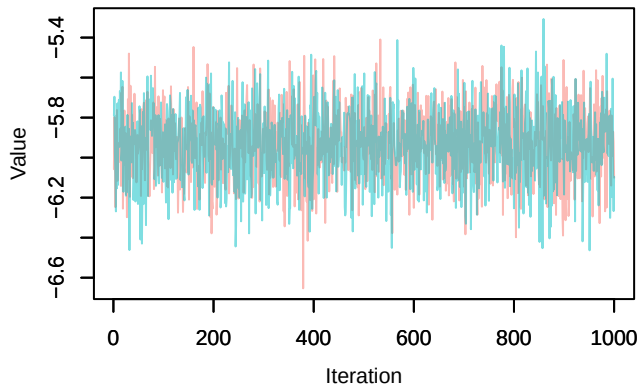
Trace – loglik[168]
