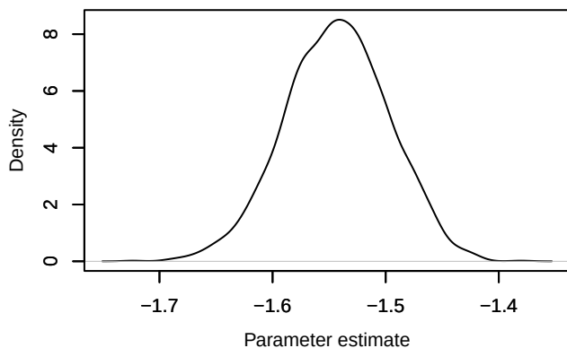
Density – loglik[288]
