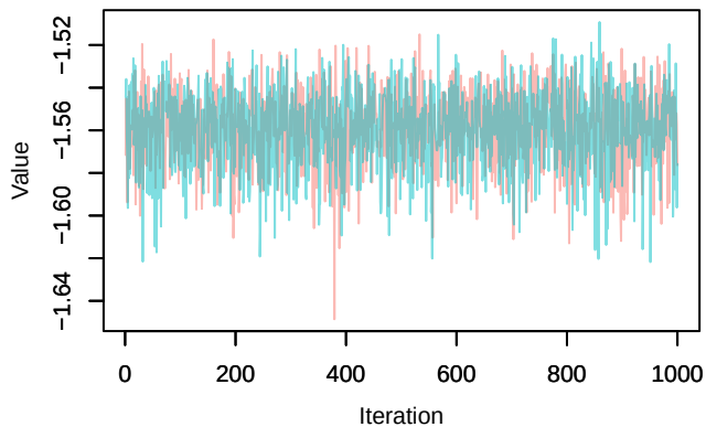
Trace – loglik[280]
