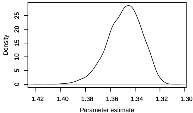
Density – loglik[66]
