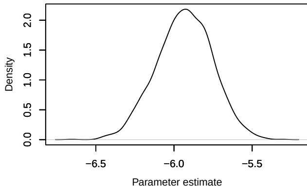
Density – loglik[168]
