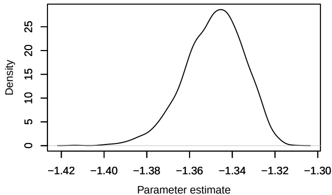
Density – loglik[165]
