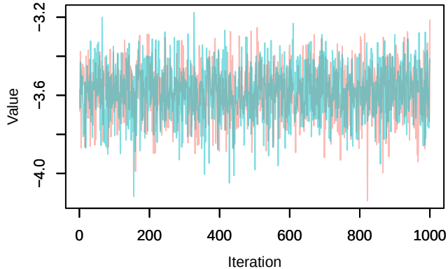
Trace – loglik[316]
