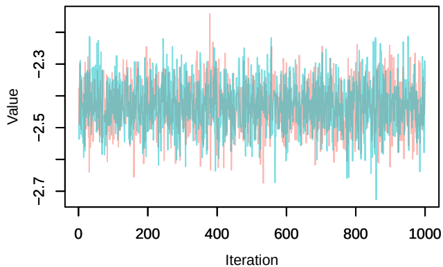
Trace – loglik[190]
