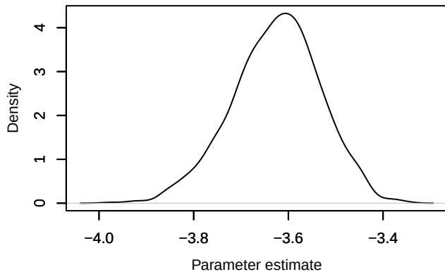
Density – loglik[384]
