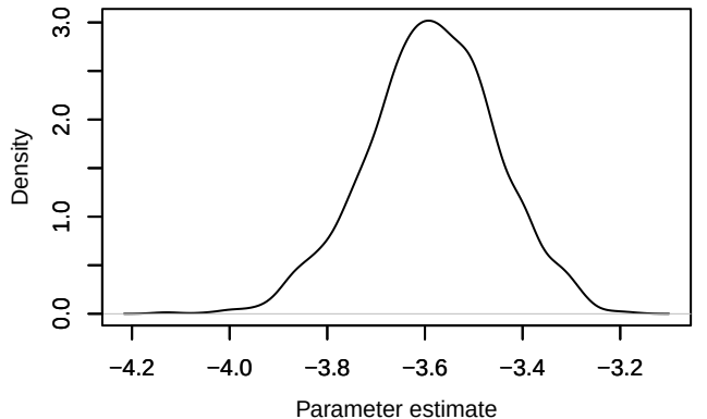
Density – loglik[388]
