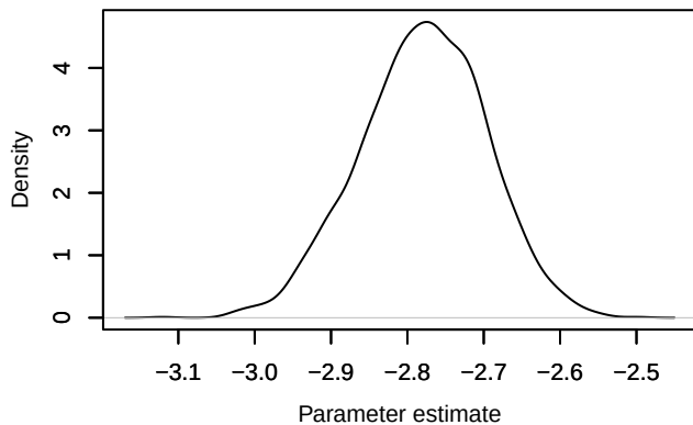
Density – loglik[259]
