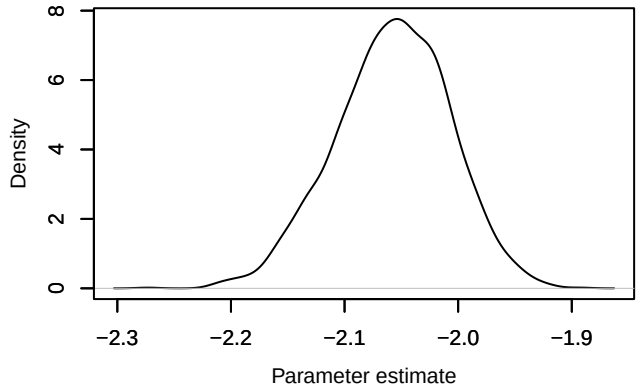
Density – loglik[295]
