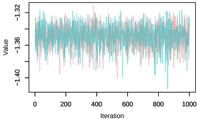
Trace – loglik[120]
