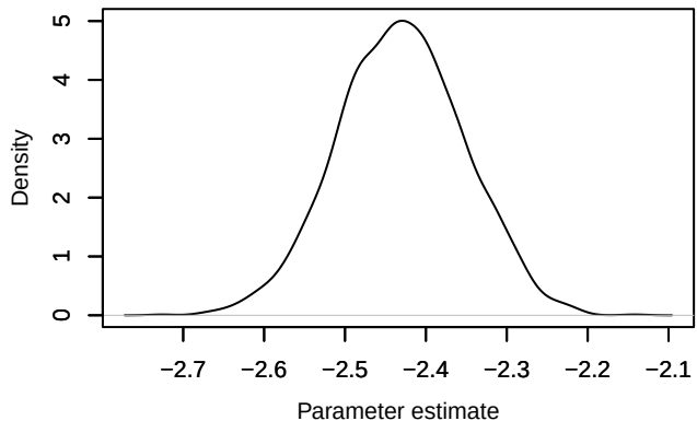
Density – loglik[106]
