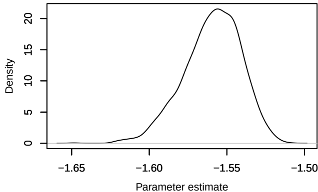
Density – loglik[145]
