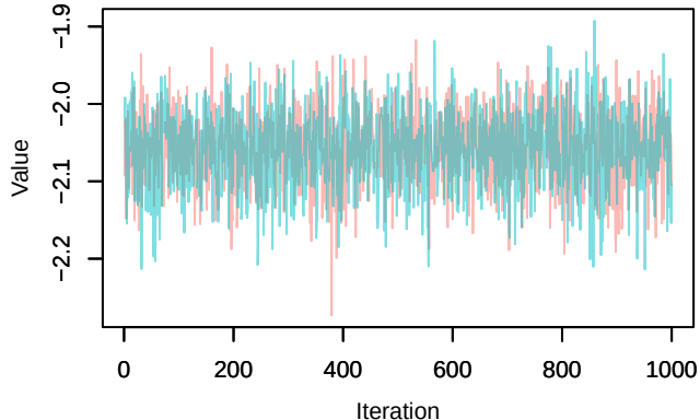
Trace – loglik[295]
