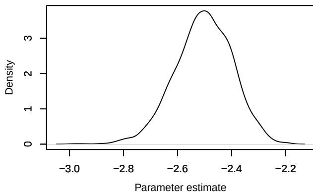
Density – loglik[328]
