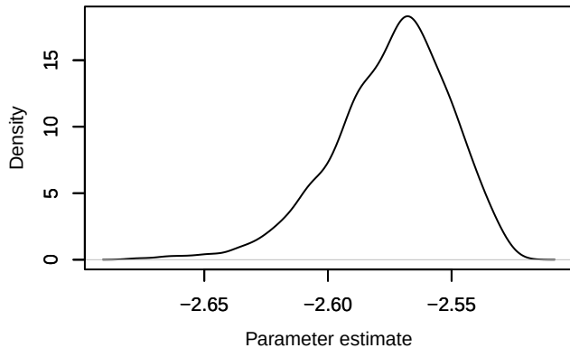
Density – loglik[382]
