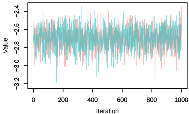
Trace – loglik[343]
