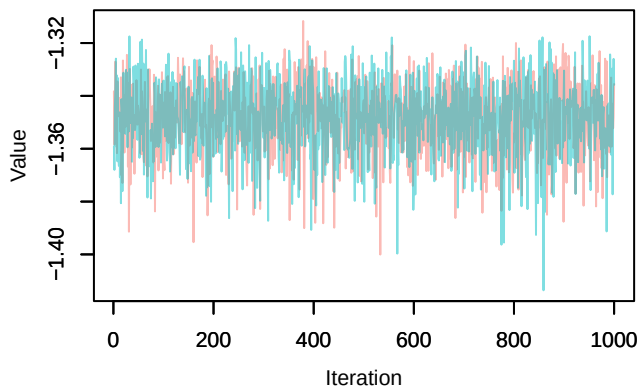
Trace – loglik[234]
