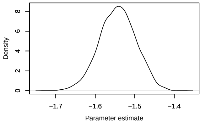
Density – loglik[232]
