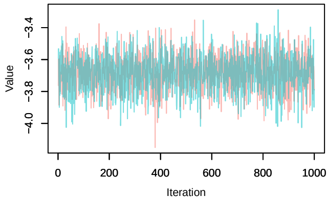
Trace – loglik[162]
