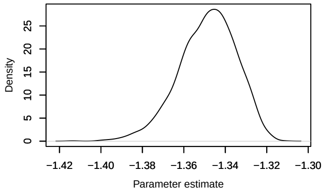
Density – loglik[246]
