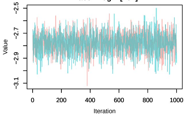
Trace – loglik[153]
