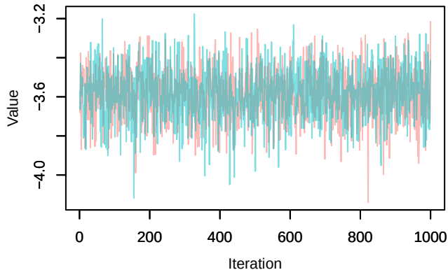
Trace – loglik[337]
