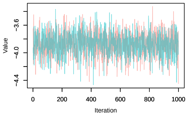
Trace – loglik[303]
