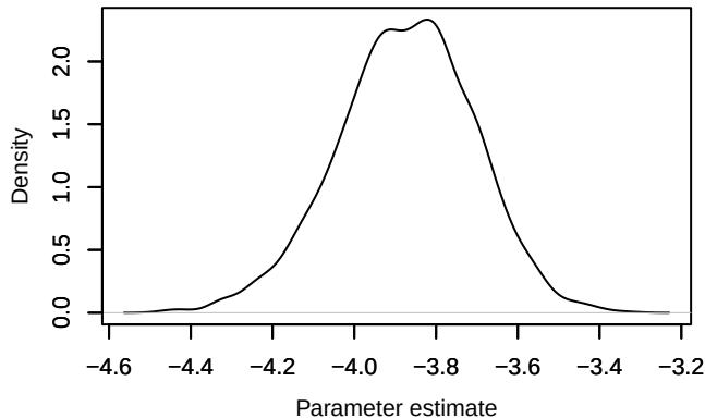
Density – loglik[400]
