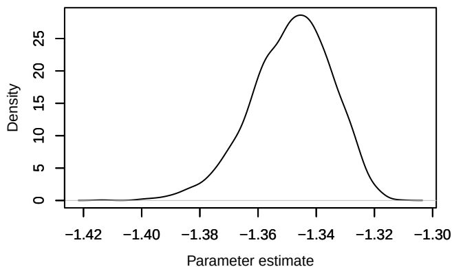
Density – loglik[222]
