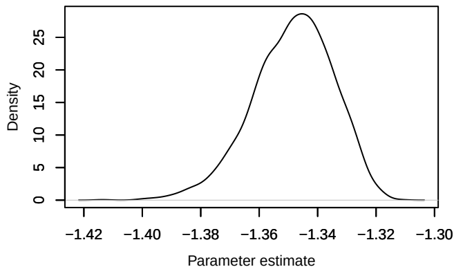
Density – loglik[205]
