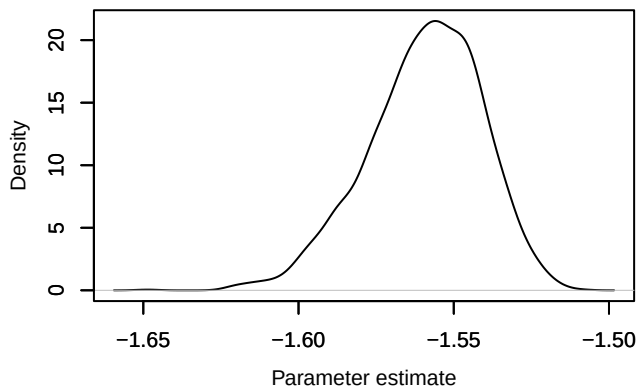
Density – loglik[150]
