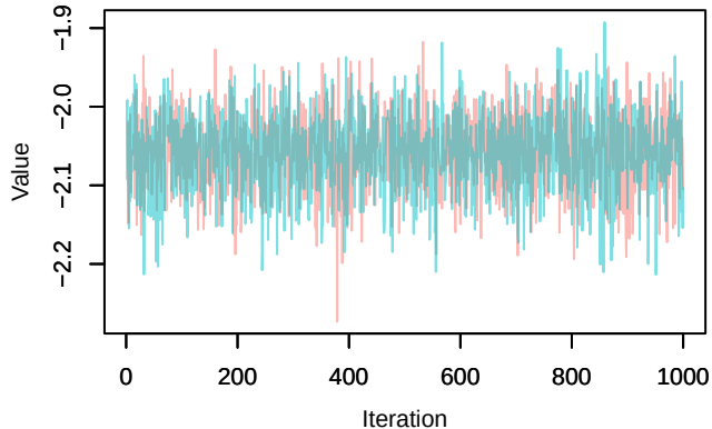
Trace – loglik[208]
