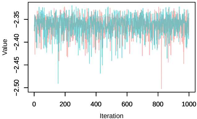
Trace – loglik[346]
