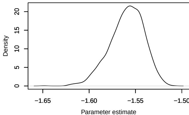
Density – loglik[280]
