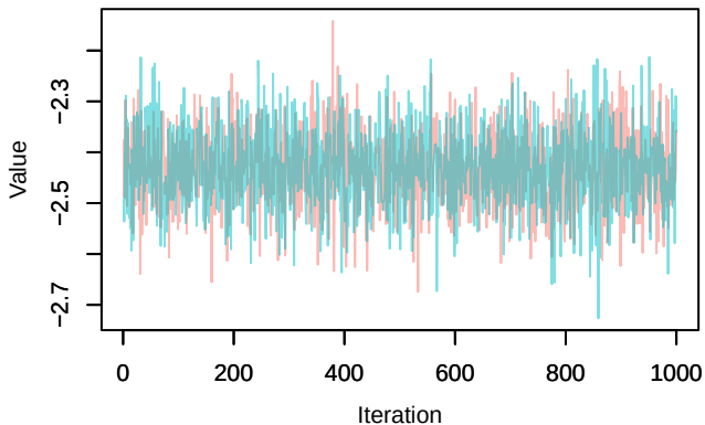
Trace – loglik[148]
