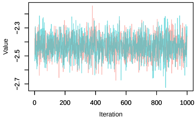
Trace – loglik[204]
