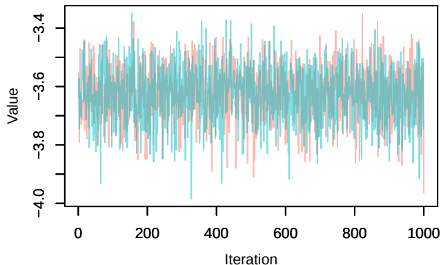
Trace – loglik[337]
