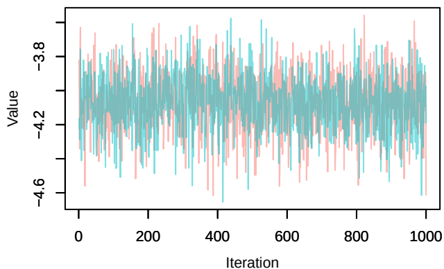
Trace – loglik[370]
