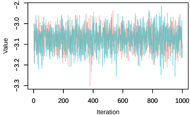
Trace – loglik[301]
