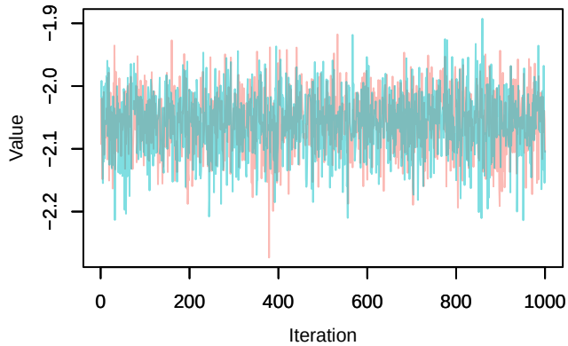
Trace – loglik[142]
