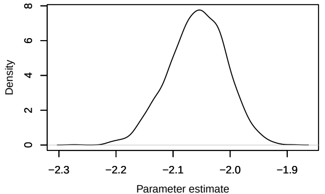
Density – loglik[202]
