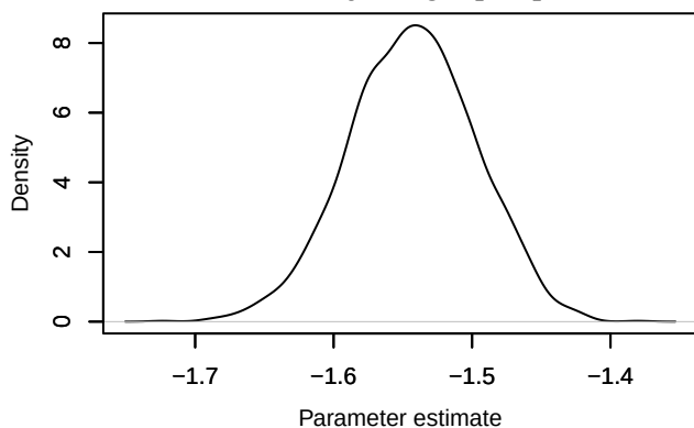
Density – loglik[240]
