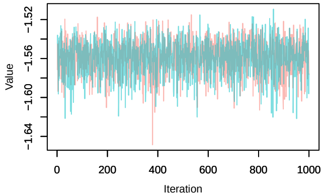
Trace – loglik[145]
