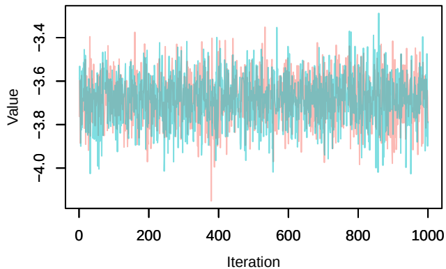
Trace – loglik[201]
