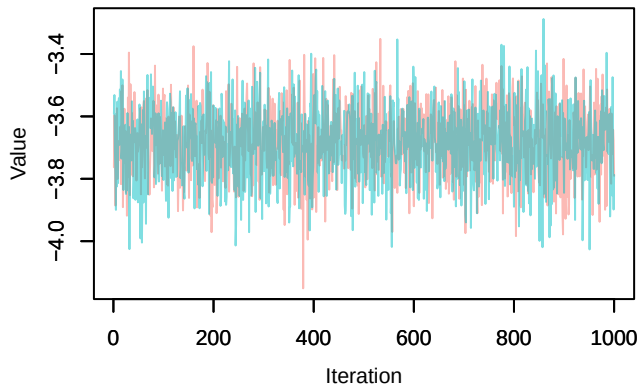
Trace – loglik[277]
