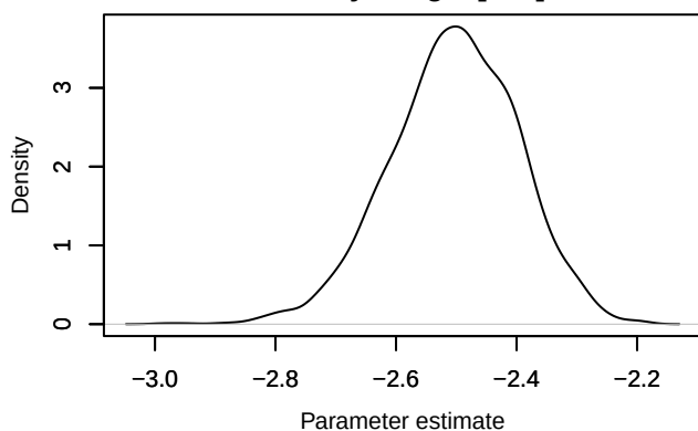
Density – loglik[355]
