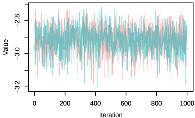
Trace – loglik[357]
