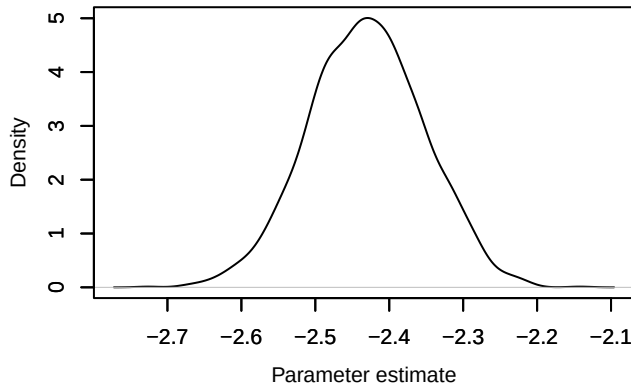
Density – loglik[163]
