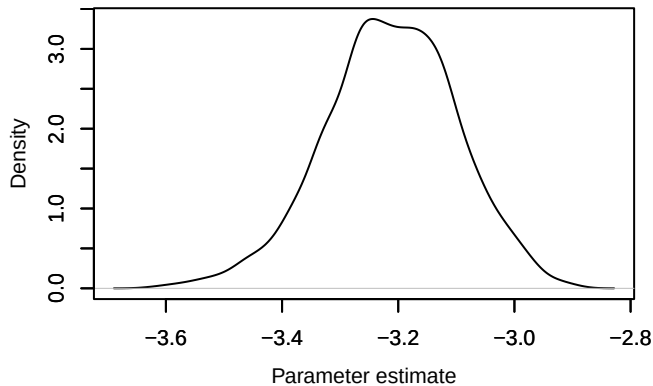
Density – loglik[324]
