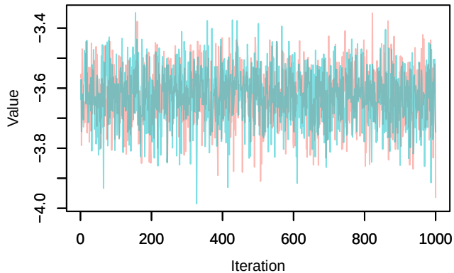
Trace – loglik[394]
