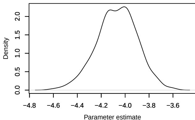
Density – loglik[370]
