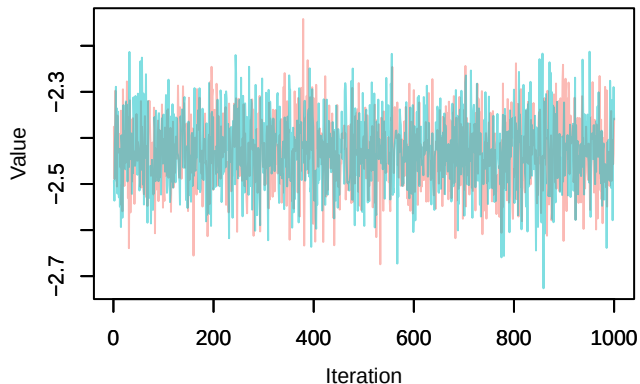
Trace – loglik[130]
