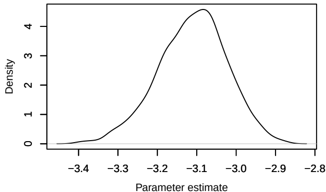
Density – loglik[330]
