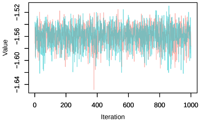
Trace – loglik[135]
