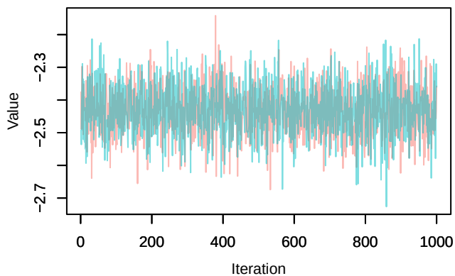
Trace – loglik[100]
