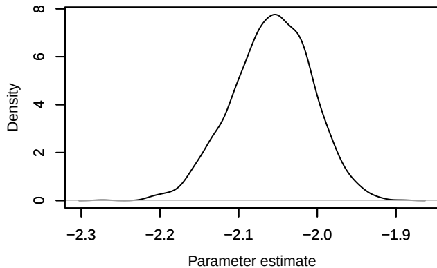
Density – loglik[222]
