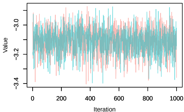
Trace – loglik[310]
