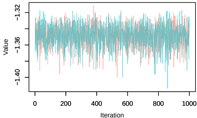
Trace – loglik[108]
