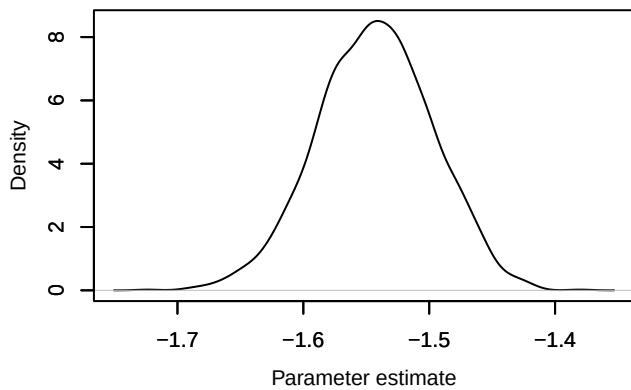
Density – loglik[127]
