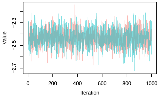
Trace – loglik[106]
