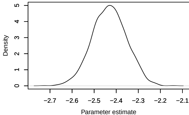
Density – loglik[244]
