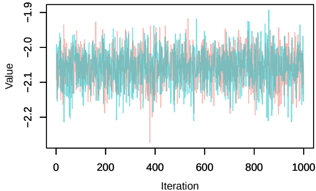
Trace – loglik[121]
