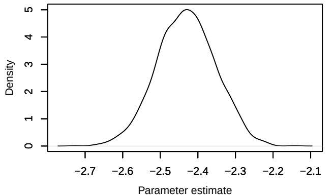
Density – loglik[220]
