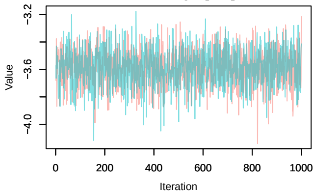
Trace – loglik[321]
