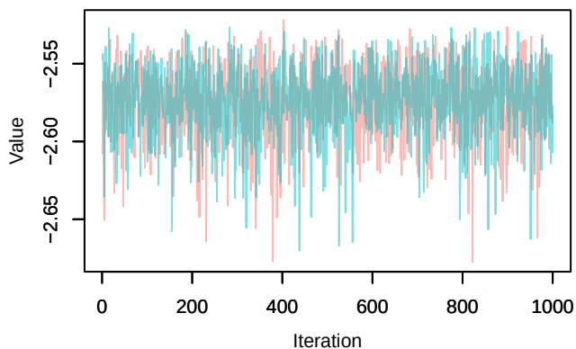
Trace – loglik[312]
