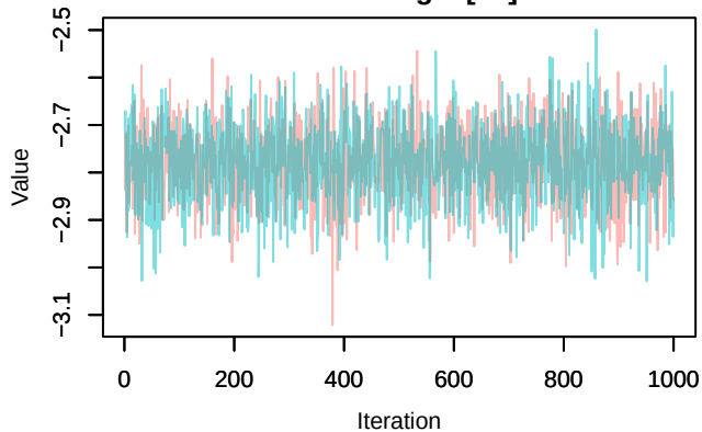
Trace – loglik[36]
