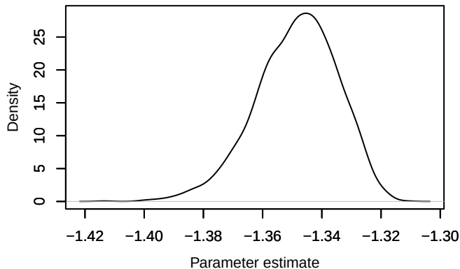
Density – loglik[37]
