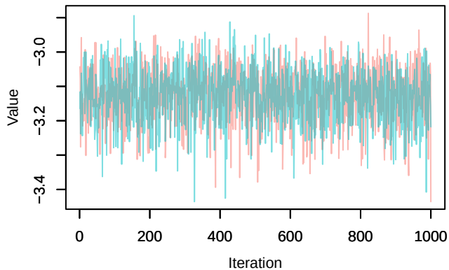
Trace – loglik[381]
