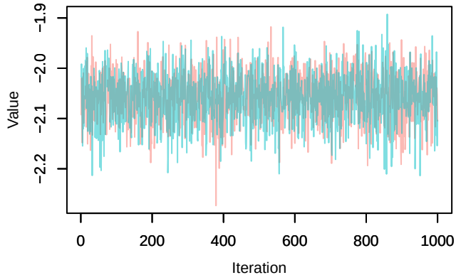
Trace – loglik[184]
