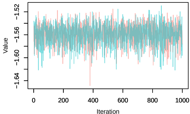
Trace – loglik[238]
