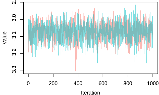
Trace – loglik[379]
