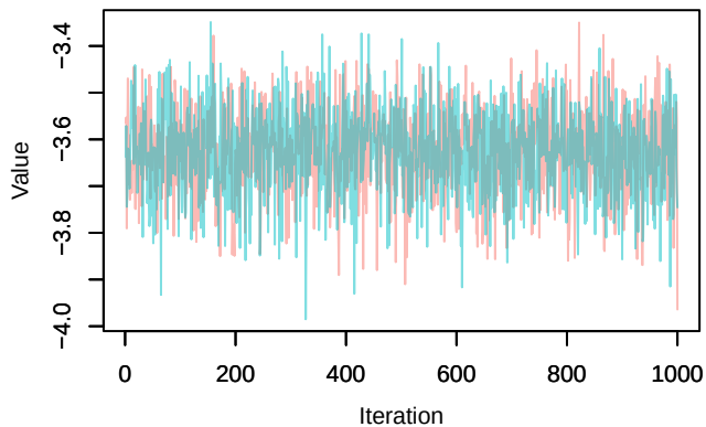
Trace – loglik[375]
