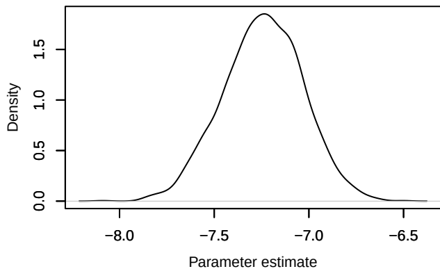
Density – loglik[148]
