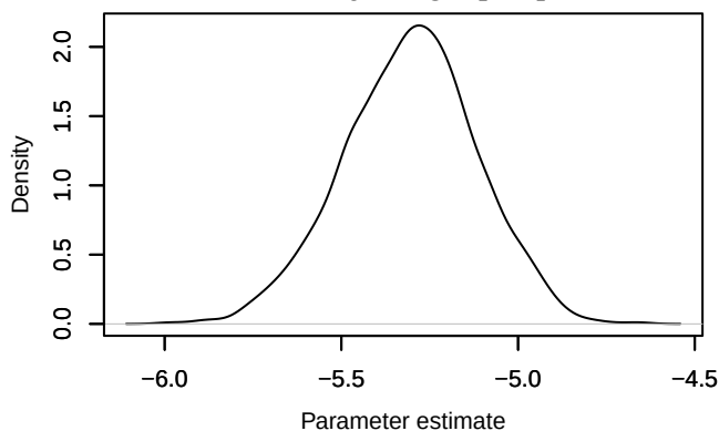
Density – loglik[307]
