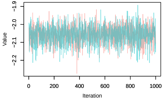
Trace – loglik[178]
