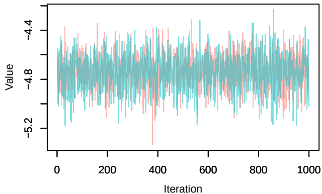
Trace – loglik[180]
