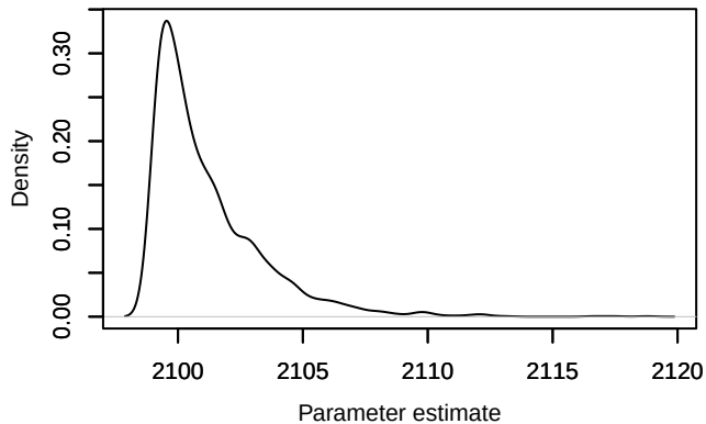
Density – lambda
