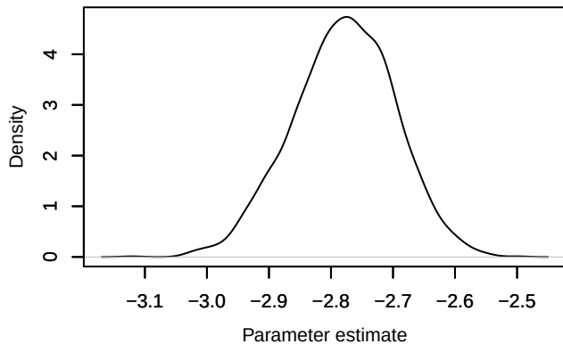
Density – loglik[159]
