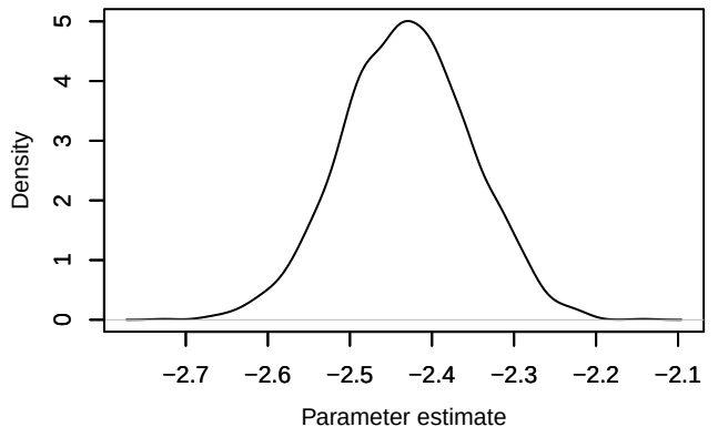
Density – loglik[202]
