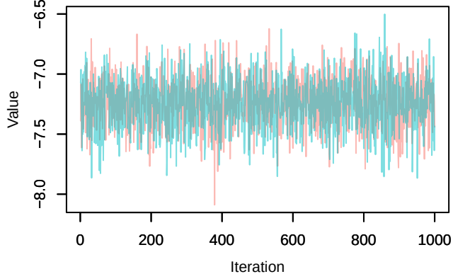
Trace – loglik[253]
