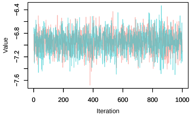
Trace – loglik[315]
