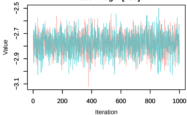
Trace – loglik[156]
