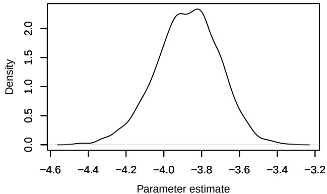
Density – loglik[385]
