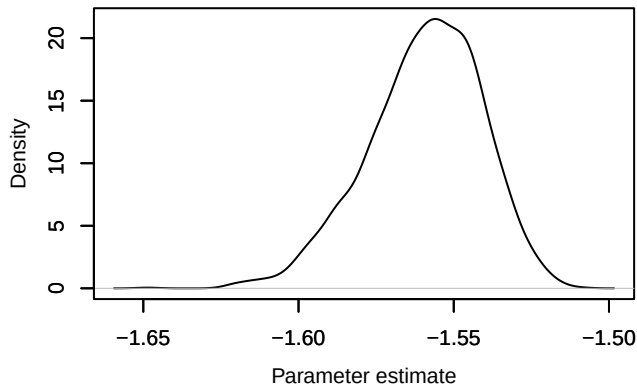
Density – loglik[286]
