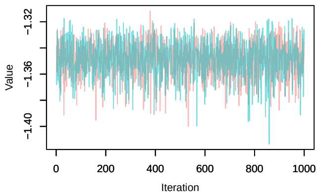
Trace – loglik[268]
