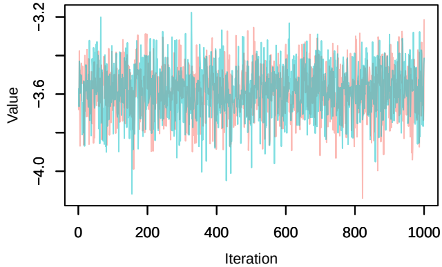
Trace – loglik[358]
