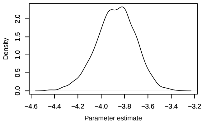
Density – loglik[303]
