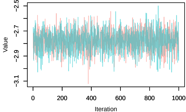
Trace – loglik[166]
