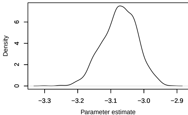
Density – loglik[301]
