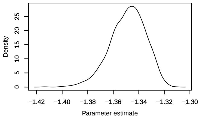
Density – loglik[78]
