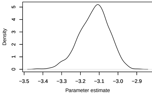
Density – loglik[358]
