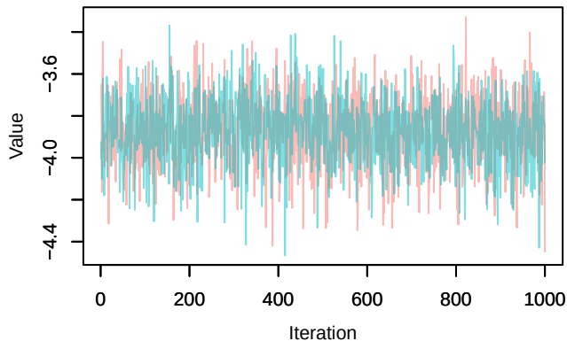
Trace – loglik[336]
