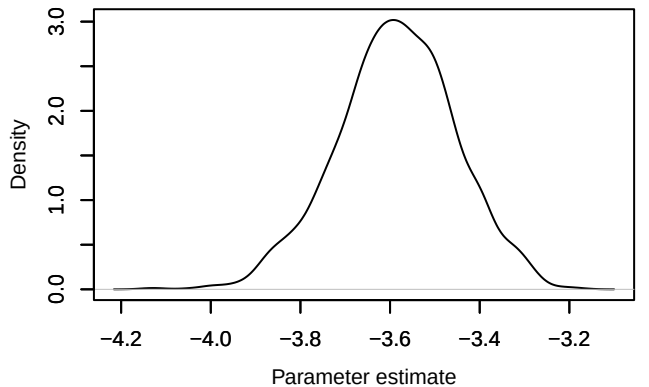
Density – loglik[388]
