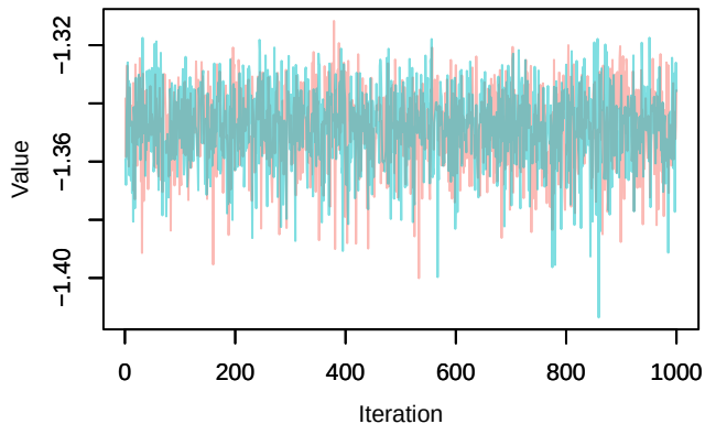
Trace – loglik[297]
