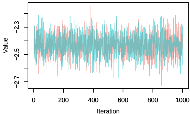
Trace – loglik[121]
