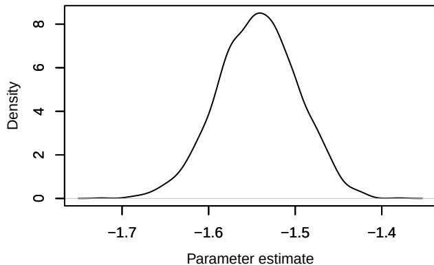
Density – loglik[184]
