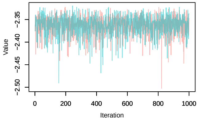
Trace – loglik[348]
