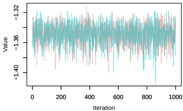
Trace – loglik[127]
