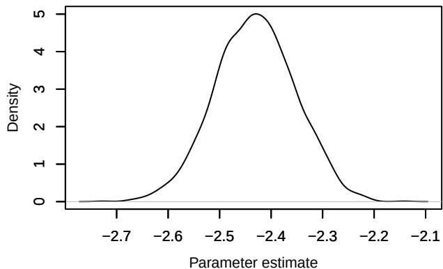
Density – loglik[217]
