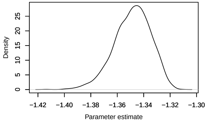
Density – loglik[103]
