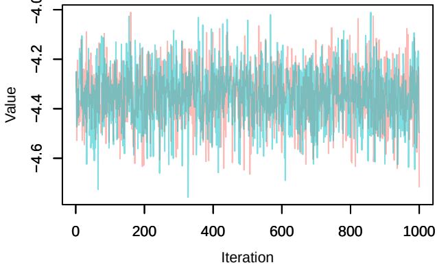
Trace – loglik[346]
