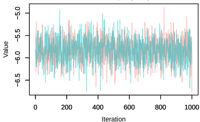
Trace – loglik[390]
