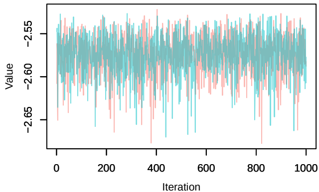
Trace – loglik[342]
