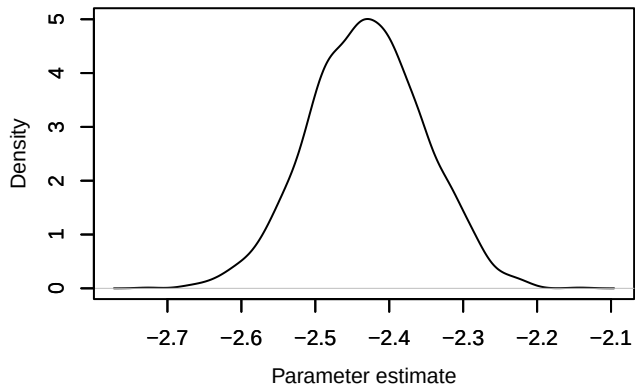
Density – loglik[276]
