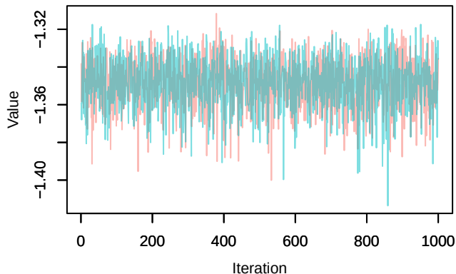
Trace – loglik[118]
