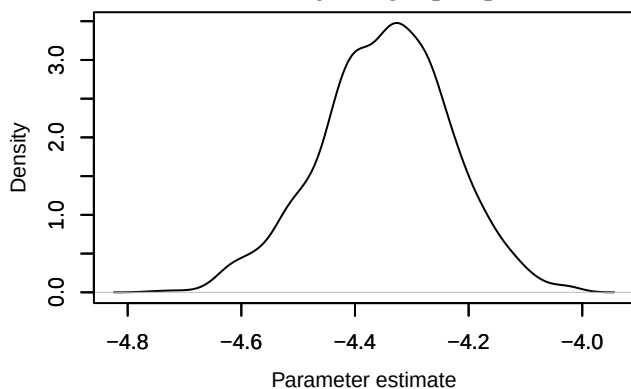
Density – loglik[352]
