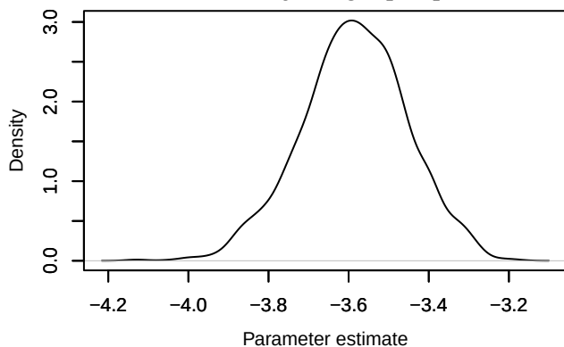
Density – loglik[327]
