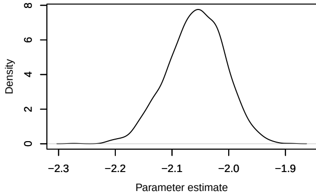
Density – loglik[265]
