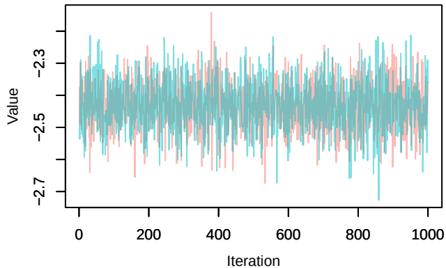
Trace – loglik[160]
