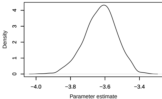
Density – loglik[375]
