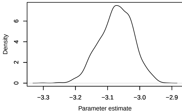
Density – loglik[318]
