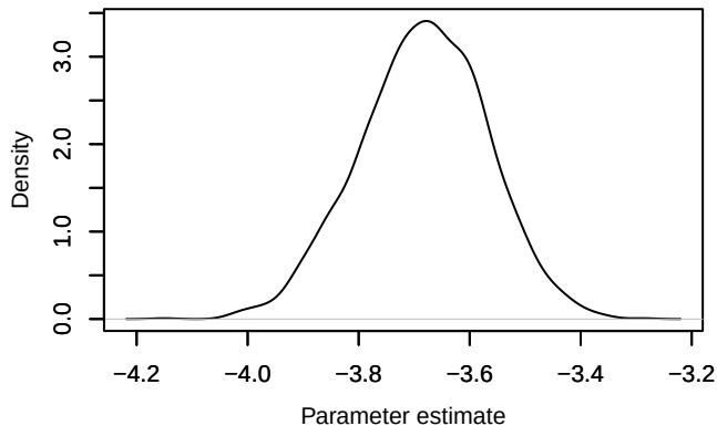
Density – loglik[162]
