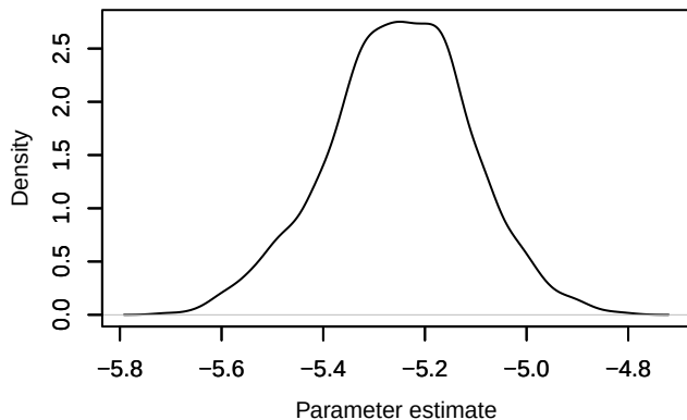
Density – loglik[379]
