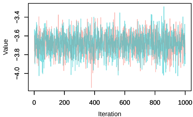
Trace – loglik[289]
