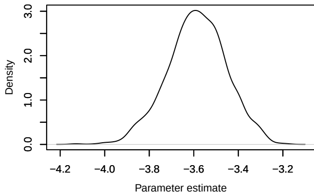
Density – loglik[309]
