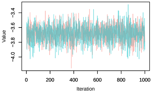
Trace – loglik[244]
