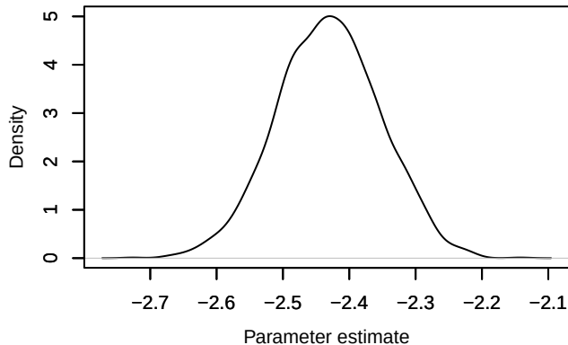
Density – loglik[211]
