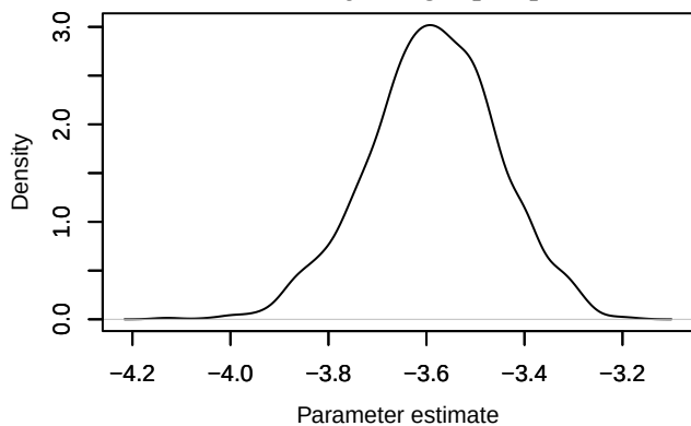
Density – loglik[306]
