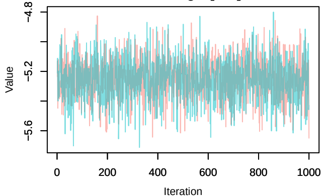
Trace – loglik[307]
