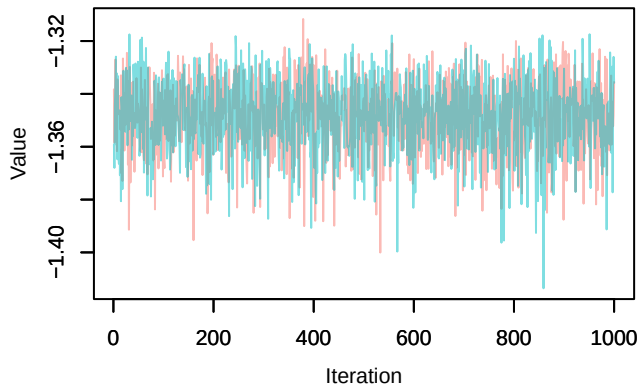
Trace – loglik[166]
