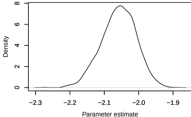
Density – loglik[193]
