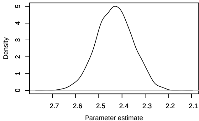
Density – loglik[277]
