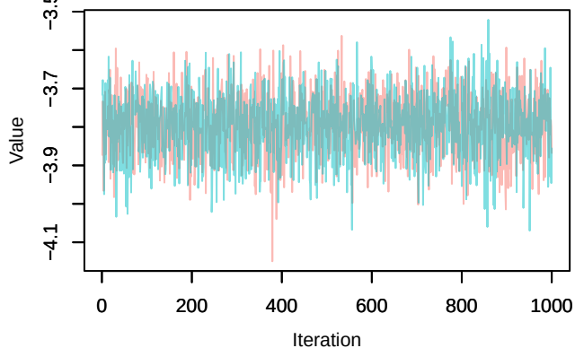
Trace – loglik[333]
