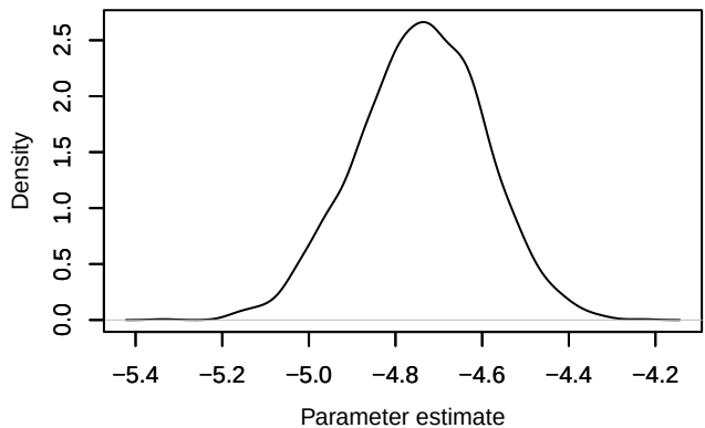
Density – loglik[286]
