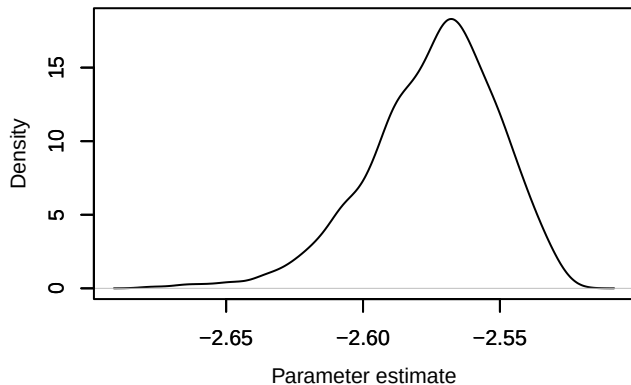
Density – loglik[343]
