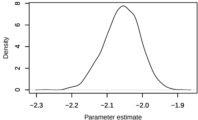
Density – loglik[136]
