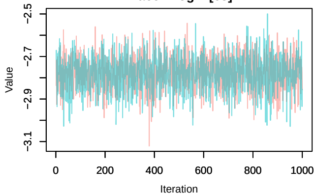
Trace – loglik[69]
