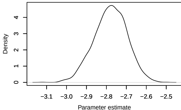
Density – loglik[72]
