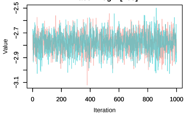
Trace – loglik[159]
