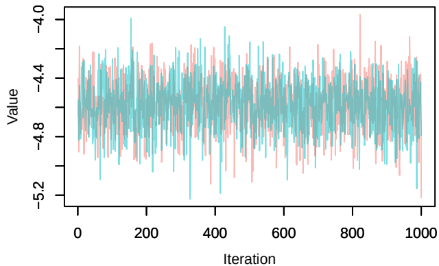
Trace – loglik[339]
