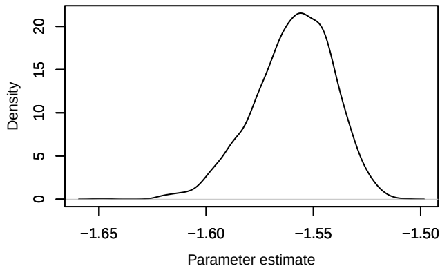
Density – loglik[198]
