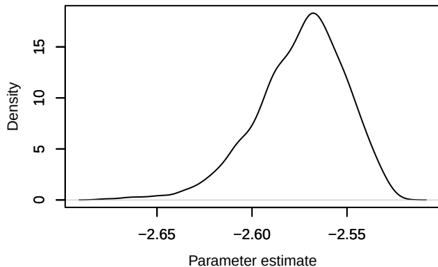
Density – loglik[378]
