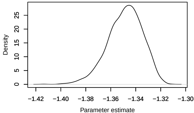
Density – loglik[97]
