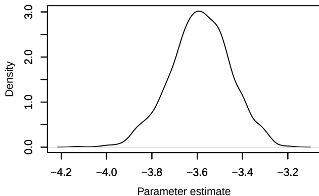
Density – loglik[367]
