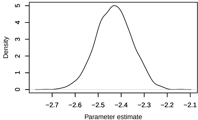
Density – loglik[292]
