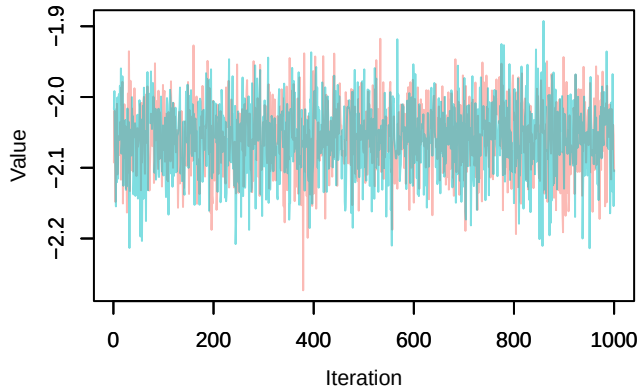
Trace – loglik[151]
