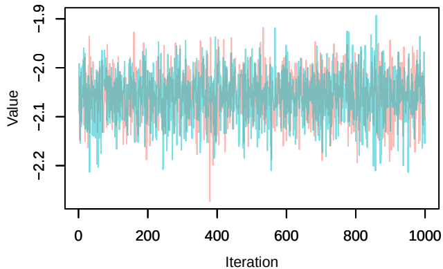
Trace – loglik[241]
