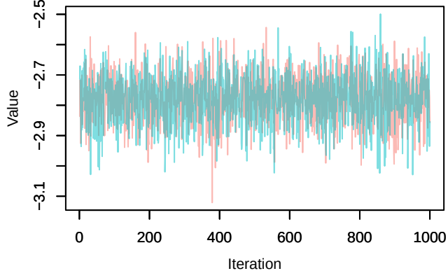
Trace – loglik[271]
