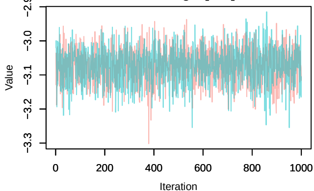
Trace – loglik[361]
