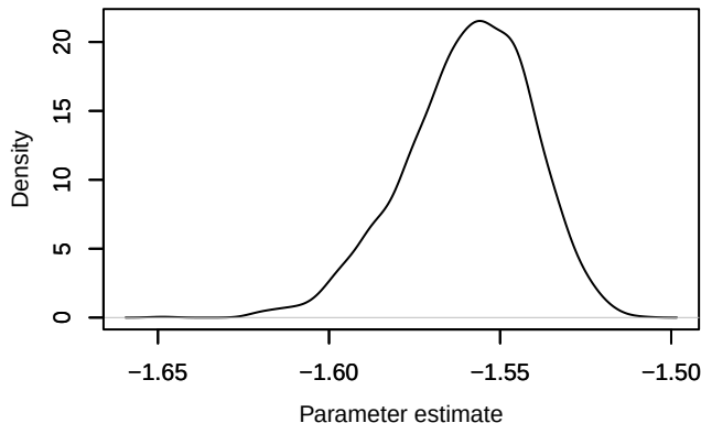
Density – loglik[238]
