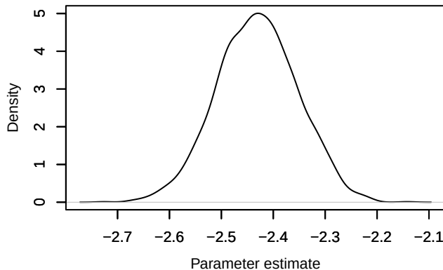
Density – loglik[226]
