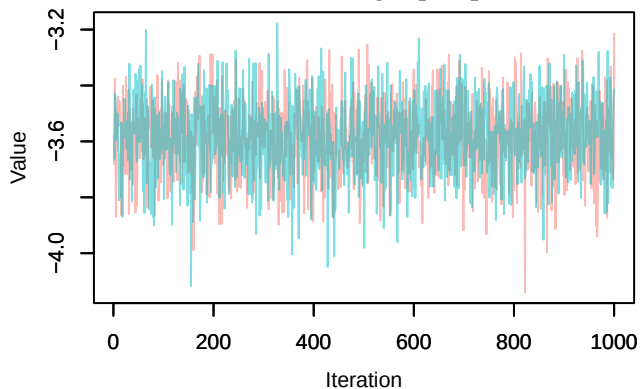
Trace – loglik[327]
