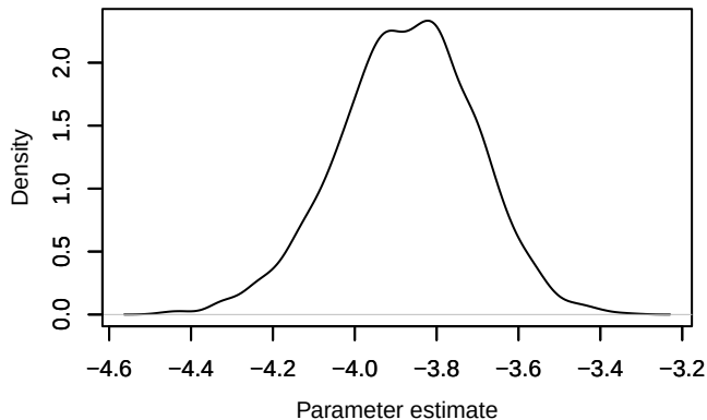
Density – loglik[336]
