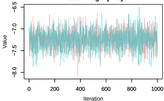
Trace – loglik[171]
