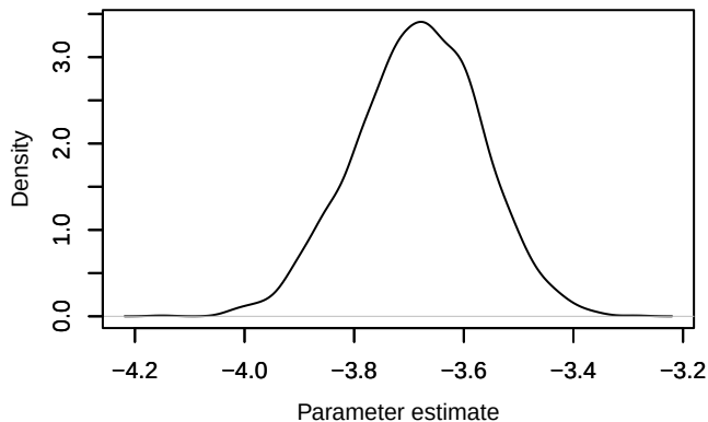
Density – loglik[28]
