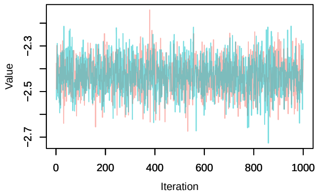
Trace – loglik[238]
