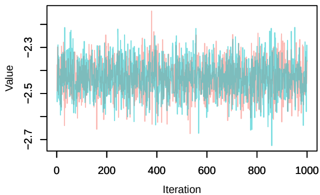
Trace – loglik[46]
