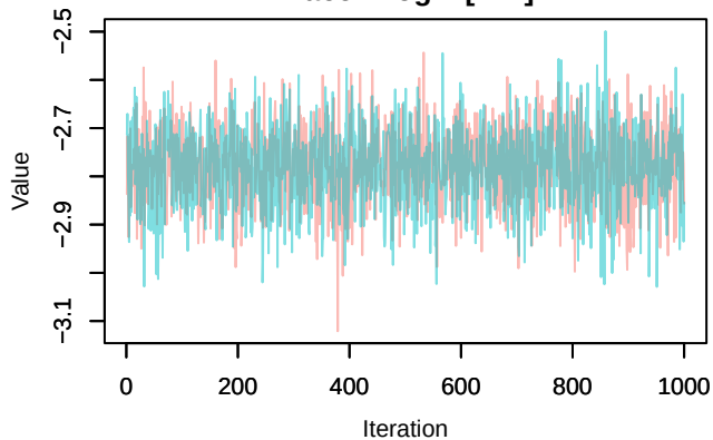
Trace – loglik[225]
