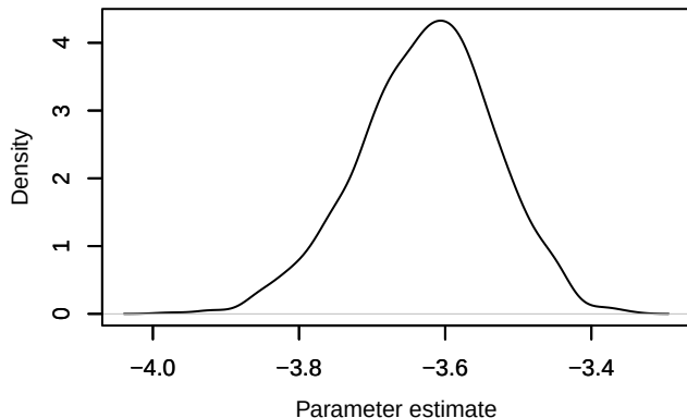
Density – loglik[337]
