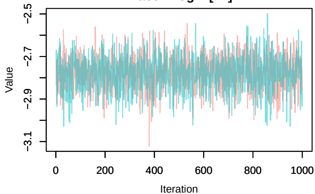
Trace – loglik[48]
