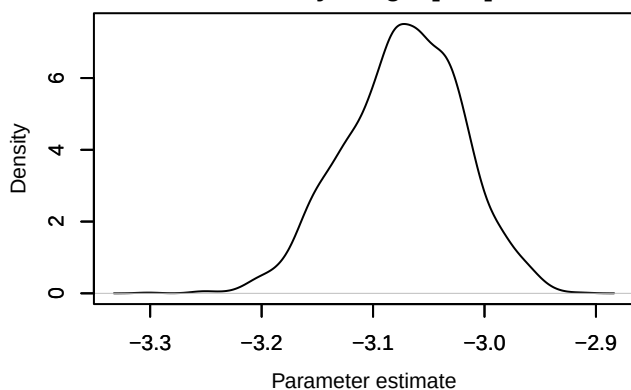
Density – loglik[361]
