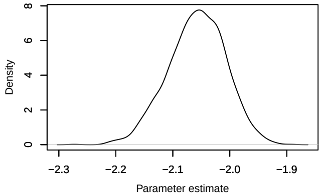
Density – loglik[208]
