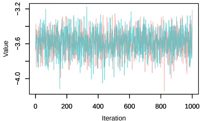
Trace – loglik[367]
