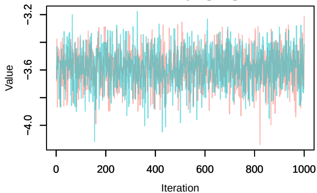
Trace – loglik[321]
