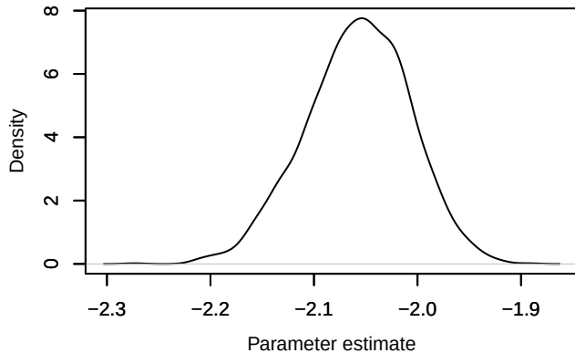
Density – loglik[184]
