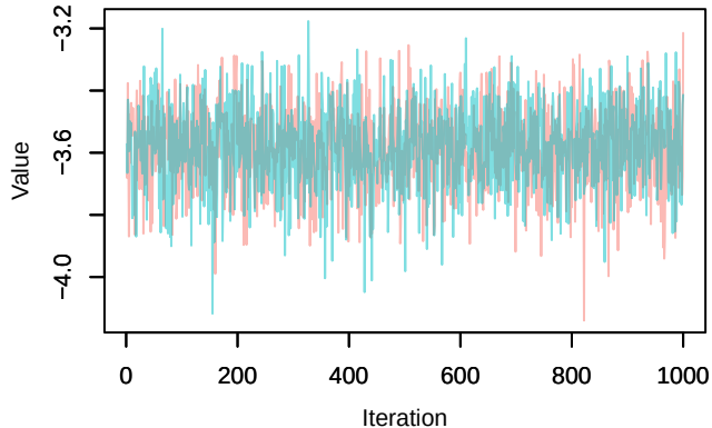
Trace – loglik[325]
