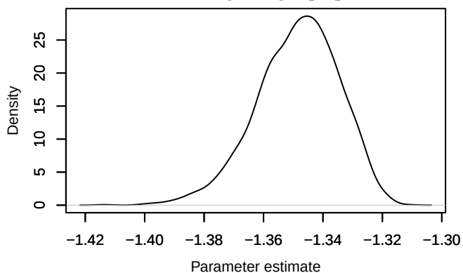
Density – loglik[99]
