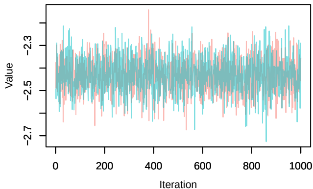
Trace – loglik[217]
