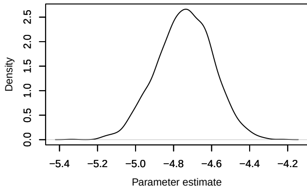
Density – loglik[180]
