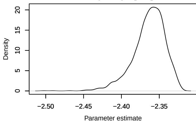
Density – loglik[360]
