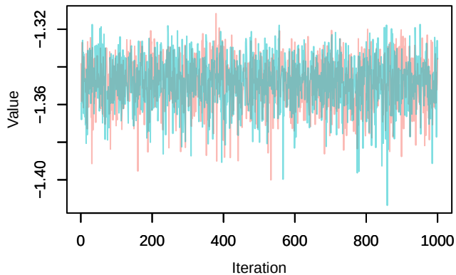
Trace – loglik[219]
