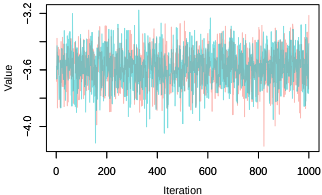
Trace – loglik[397]
