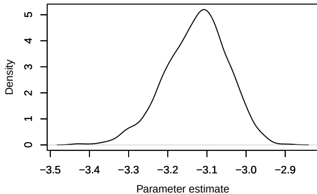
Density – loglik[381]
