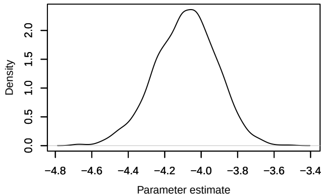
Density – loglik[331]
