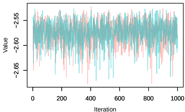
Trace – loglik[340]
