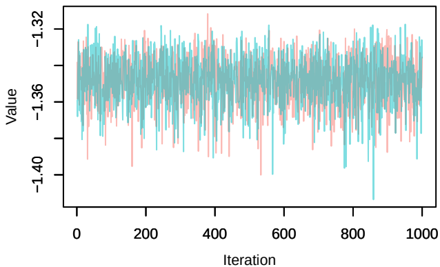
Trace – loglik[124]
