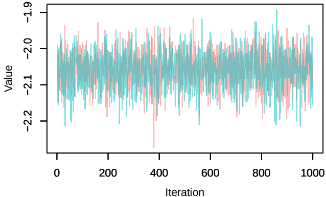
Trace – loglik[136]
