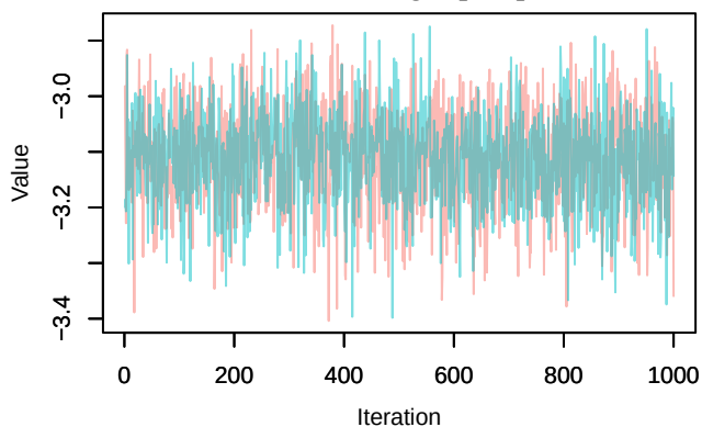
Trace – loglik[355]
