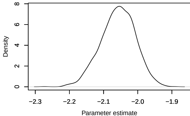
Density – loglik[195]
