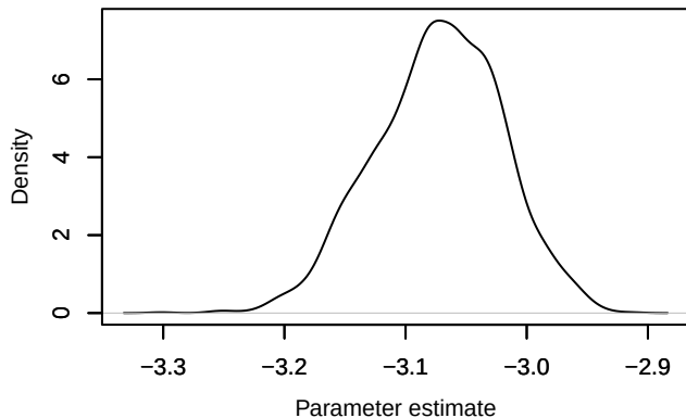
Density – loglik[397]
