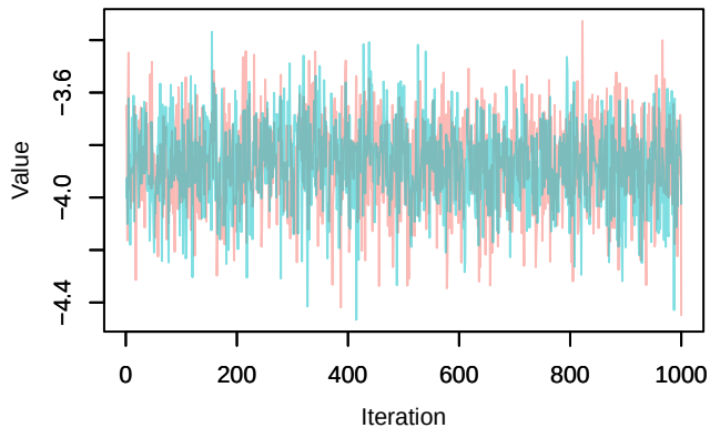
Trace – loglik[387]
