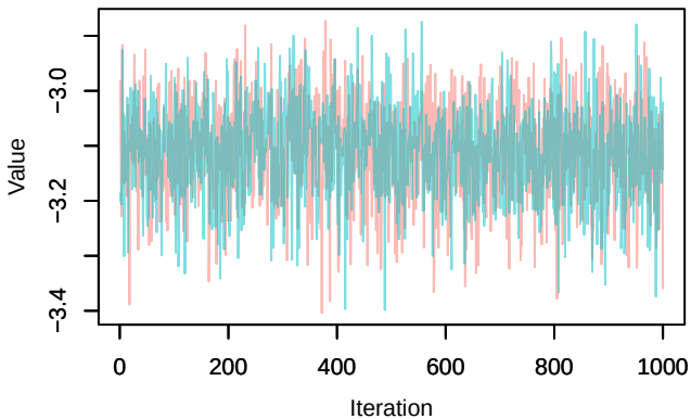
Trace – loglik[345]
