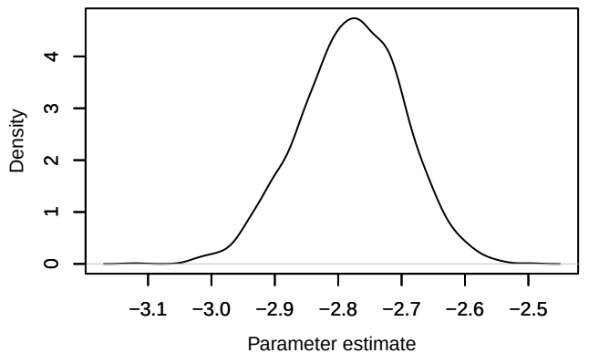
Density – loglik[166]
