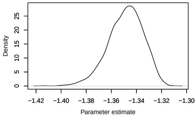
Density – loglik[124]
