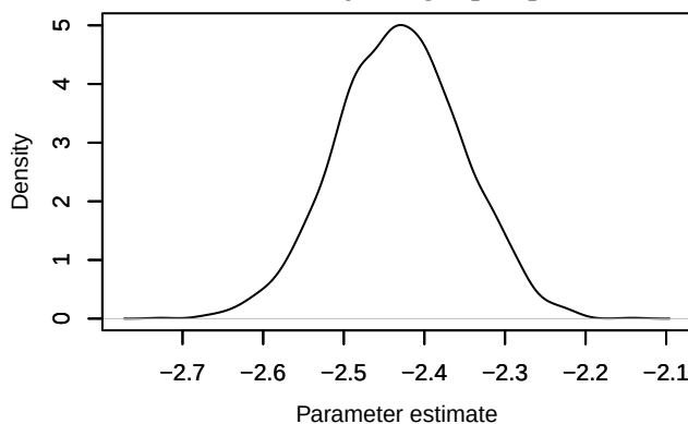
Density – loglik[249]
