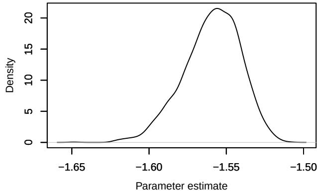
Density – loglik[13]
