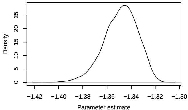
Density – loglik[301]
