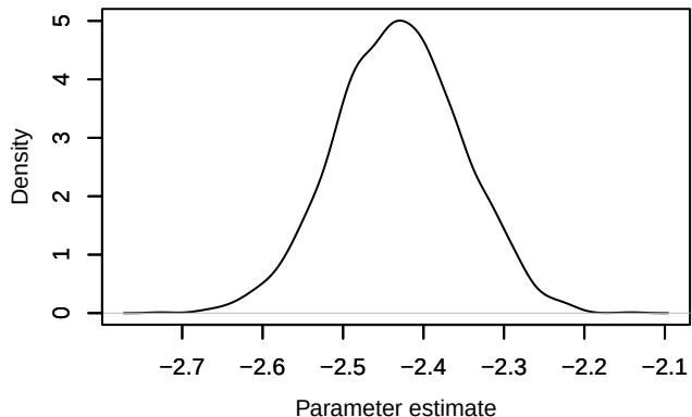
Density – loglik[130]
