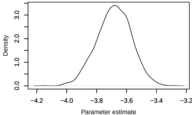
Density – loglik[1]
