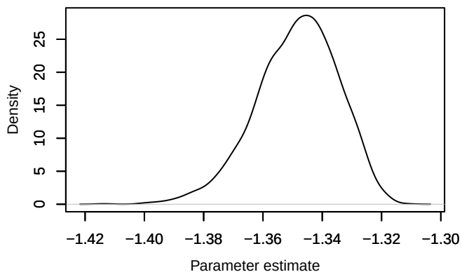
Density – loglik[195]
