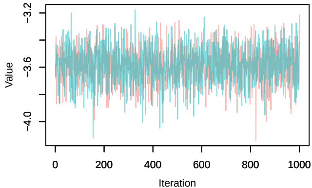
Trace – loglik[388]
