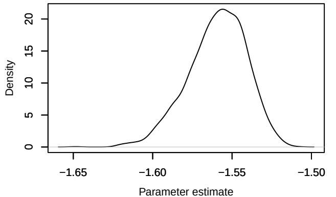
Density – loglik[298]
