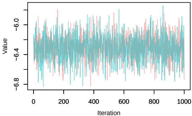
Trace – loglik[396]
