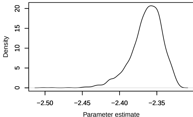
Density – loglik[400]
