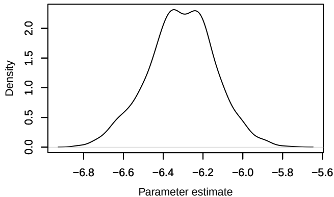
Density – loglik[396]
