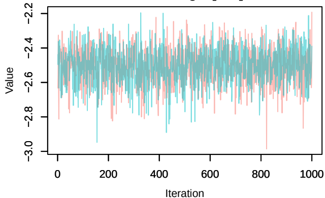
Trace – loglik[355]
