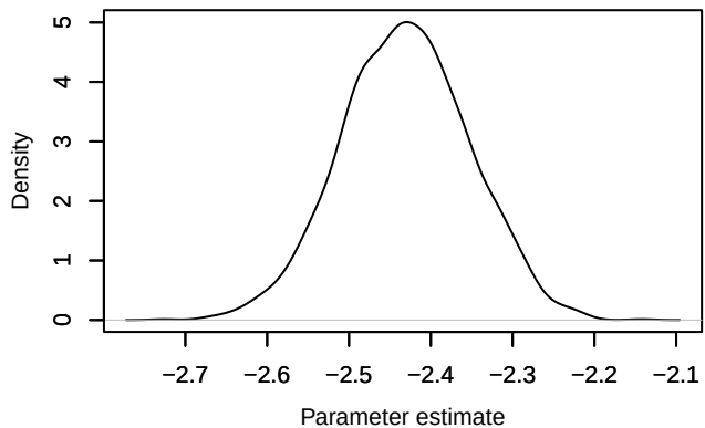
Density – loglik[169]
