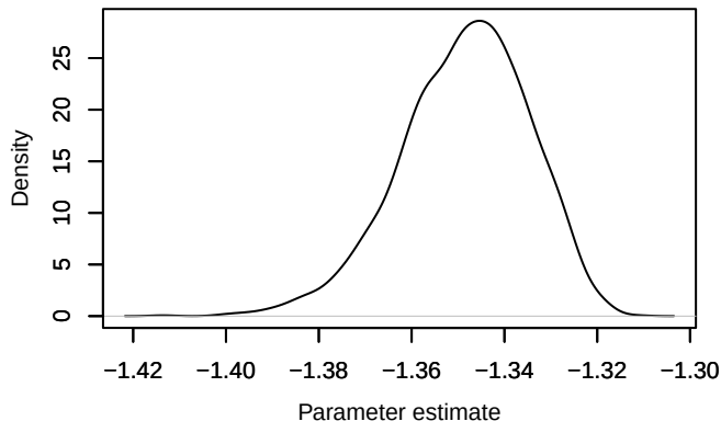
Density – loglik[217]
