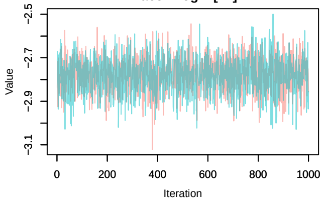
Trace – loglik[72]
