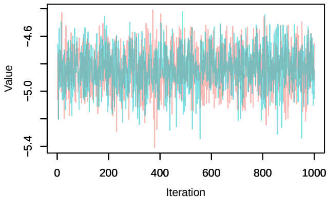
Trace – loglik[399]
