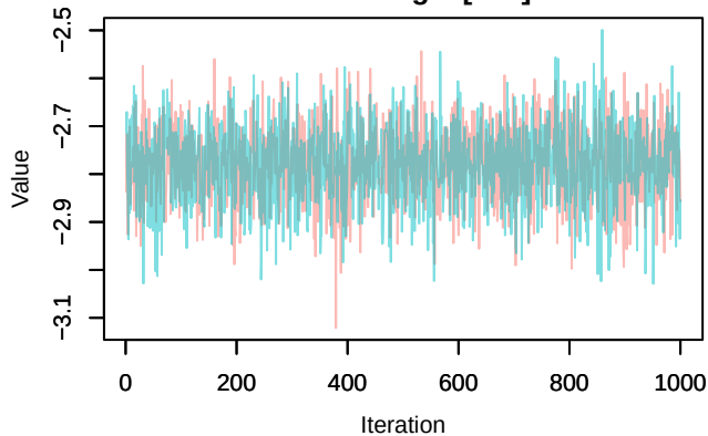
Trace – loglik[255]
