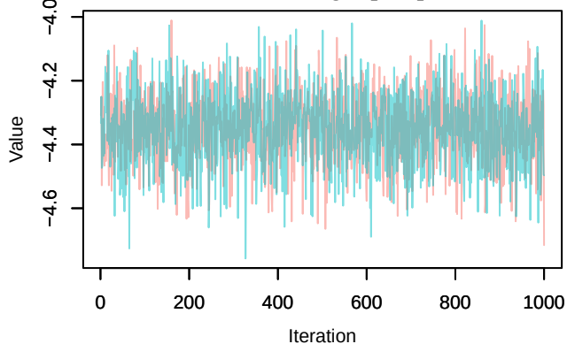
Trace – loglik[352]
