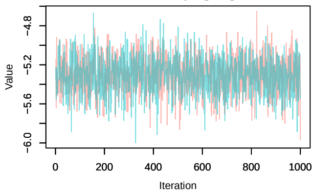
Trace – loglik[307]
