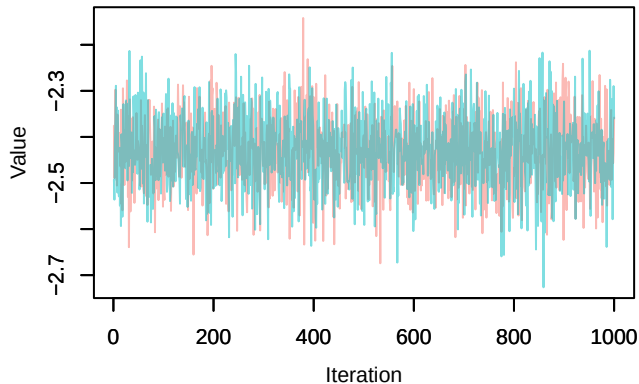
Trace – loglik[211]
