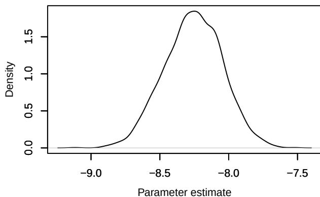
Density – loglik[339]
