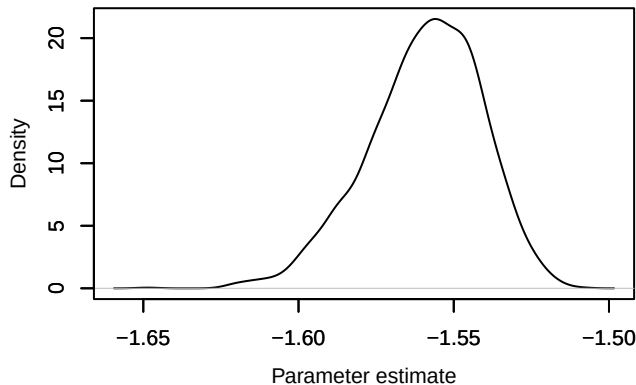
Density – loglik[237]
