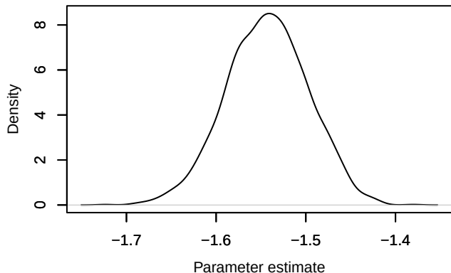
Density – loglik[205]
