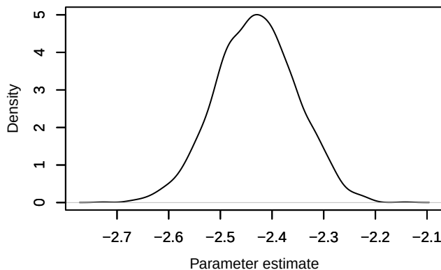
Density – loglik[270]
