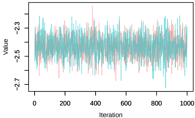
Trace – loglik[276]
