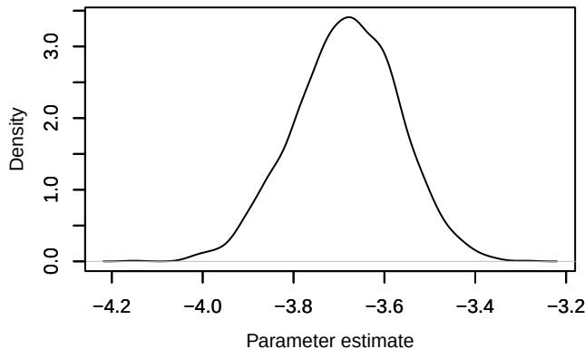
Density – loglik[244]
