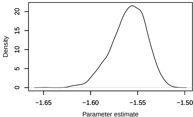
Density – loglik[208]
