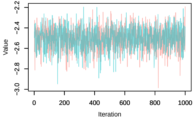
Trace – loglik[328]
