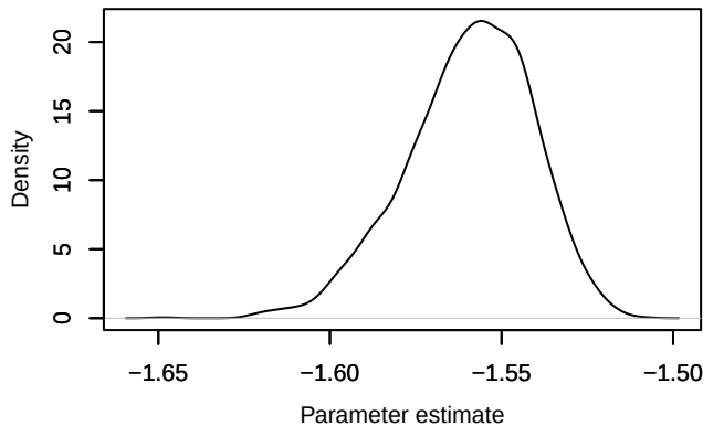
Density – loglik[291]
