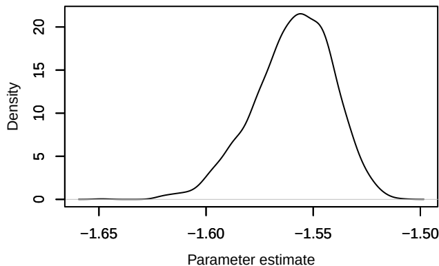
Density – loglik[139]
