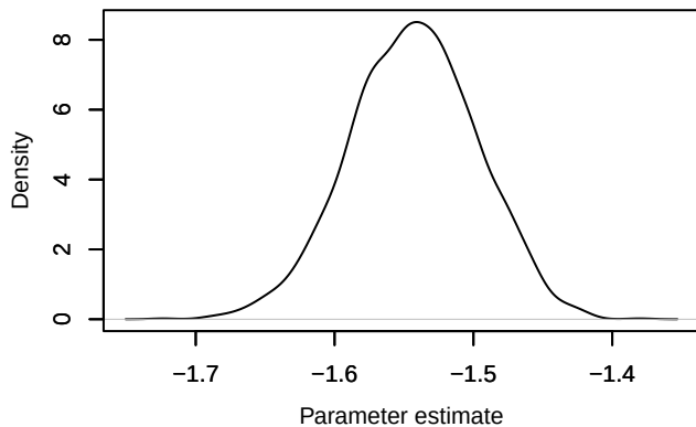
Density – loglik[150]
