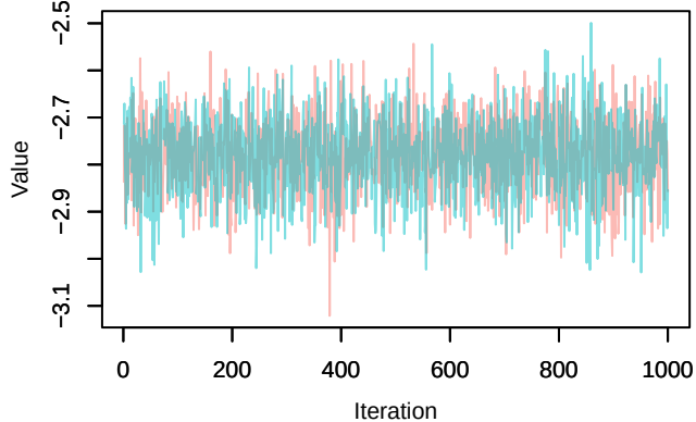
Trace – loglik[112]
