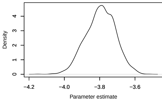
Density – loglik[376]
