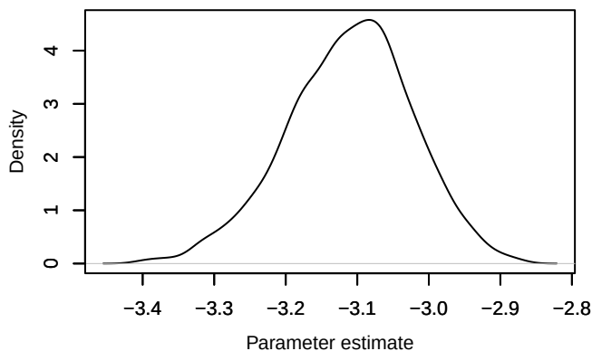
Density – loglik[310]
