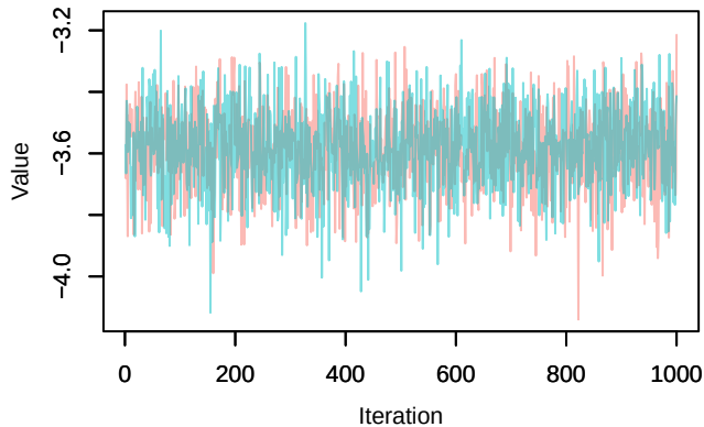
Trace – loglik[366]
