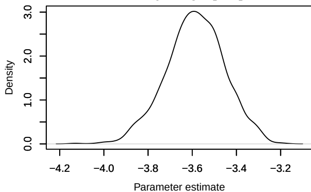
Density – loglik[390]
