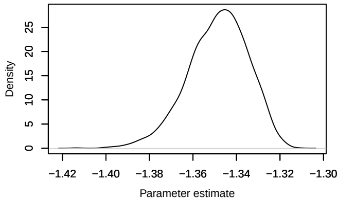
Density – loglik[108]
