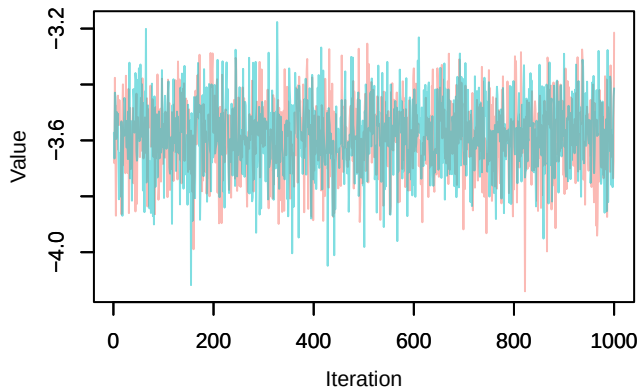
Trace – loglik[369]
