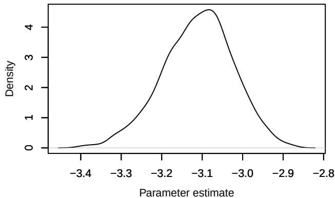
Density – loglik[345]
