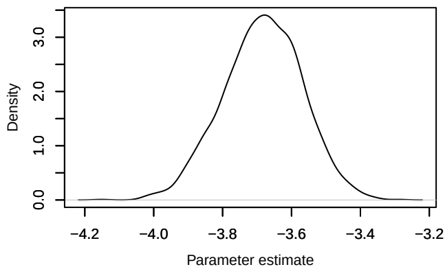
Density – loglik[289]
