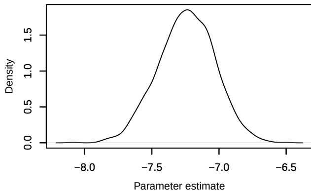
Density – loglik[253]
