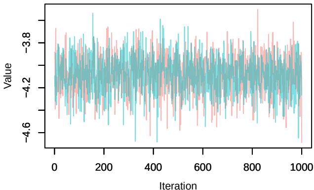
Trace – loglik[331]
