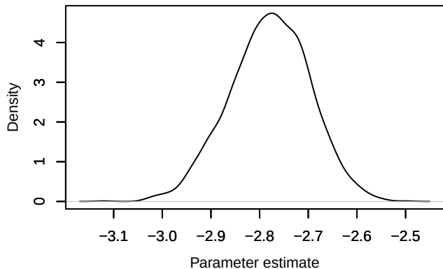
Density – loglik[262]
