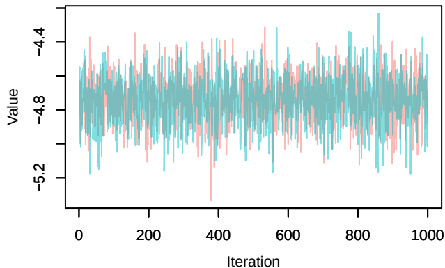
Trace – loglik[67]
