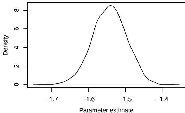
Density – loglik[280]
