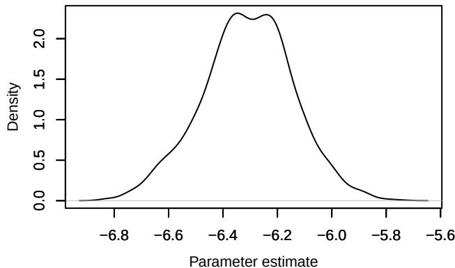
Density – loglik[319]
