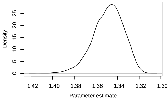
Density – loglik[295]
