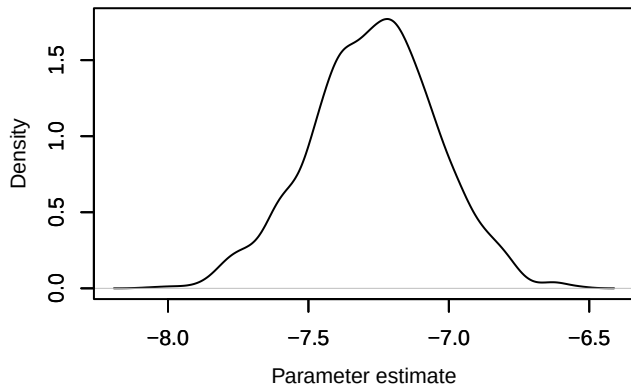
Density – loglik[394]
