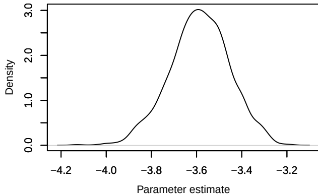
Density – loglik[325]
