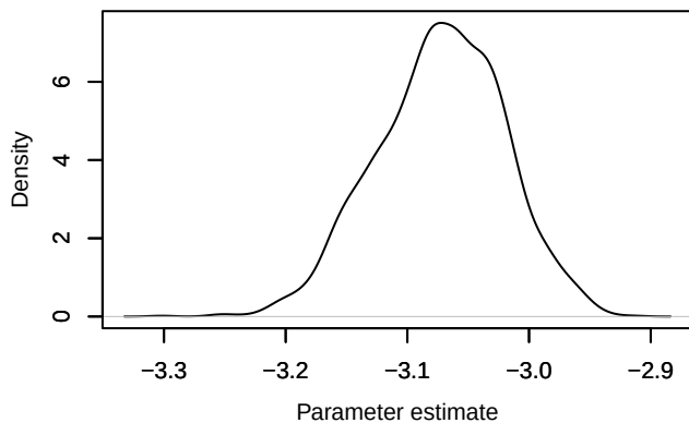
Density – loglik[319]
