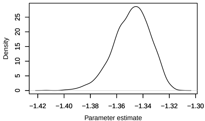
Density – loglik[196]
