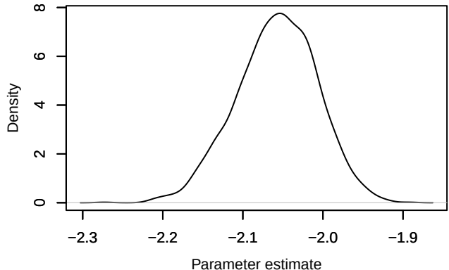
Density – loglik[199]
