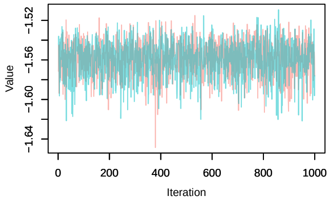
Trace – loglik[169]
