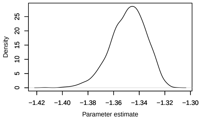
Density – loglik[234]
