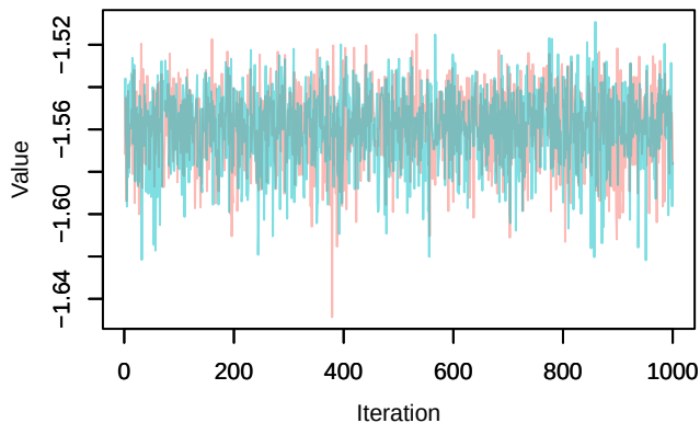
Trace – loglik[139]
