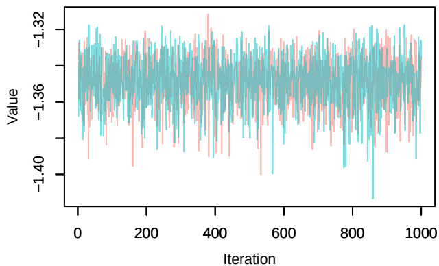
Trace – loglik[196]
