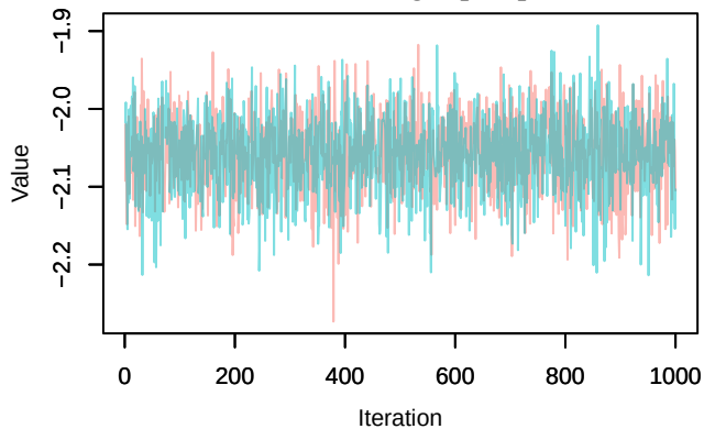
Trace – loglik[141]
