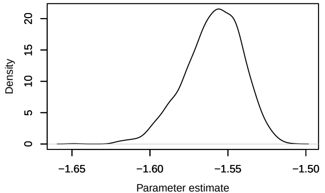
Density – loglik[88]
