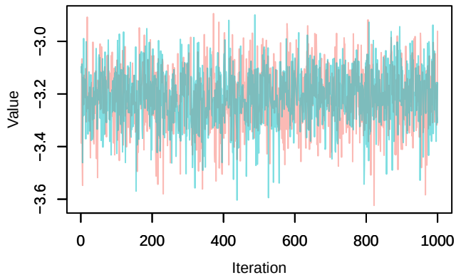
Trace – loglik[324]
