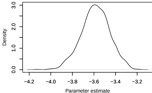
Density – loglik[331]
