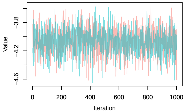
Trace – loglik[393]
