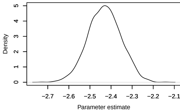
Density – loglik[190]
