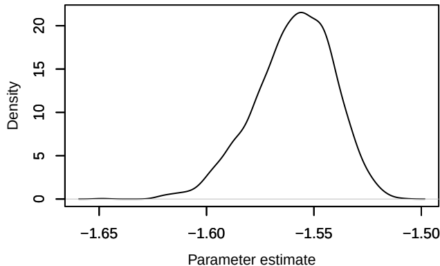
Density – loglik[118]
