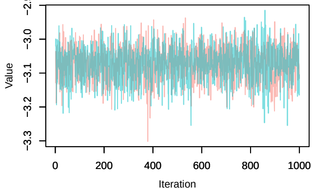
Trace – loglik[319]
