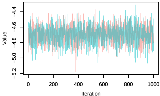
Trace – loglik[382]
