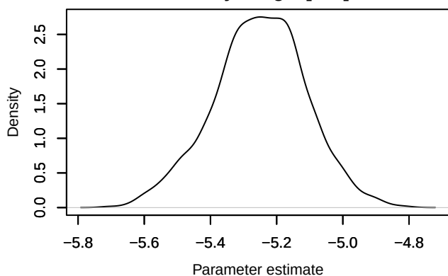
Density – loglik[307]
