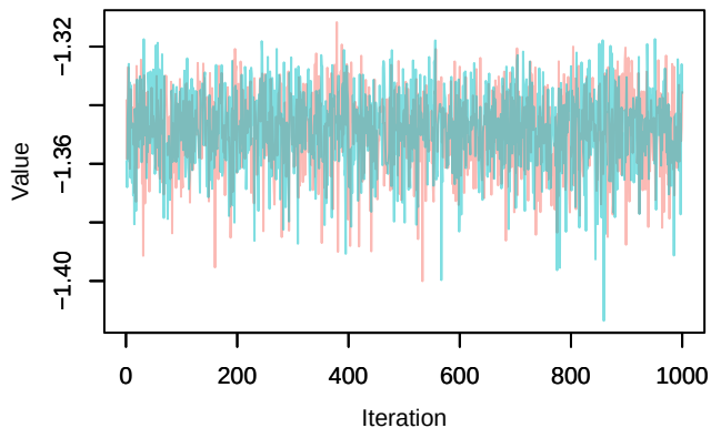
Trace – loglik[205]
