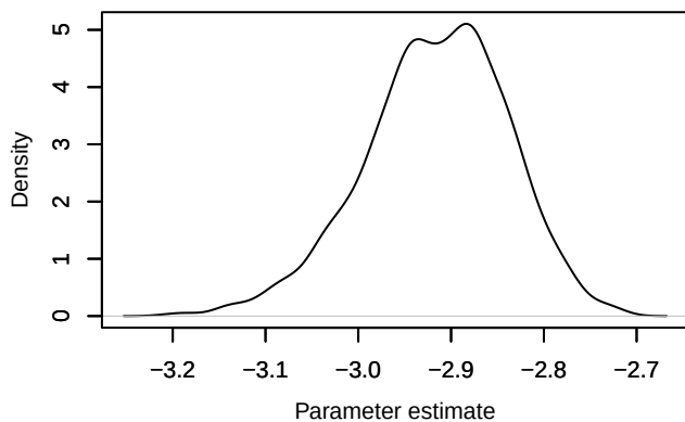
Density – loglik[391]
