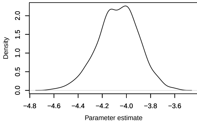
Density – loglik[393]
