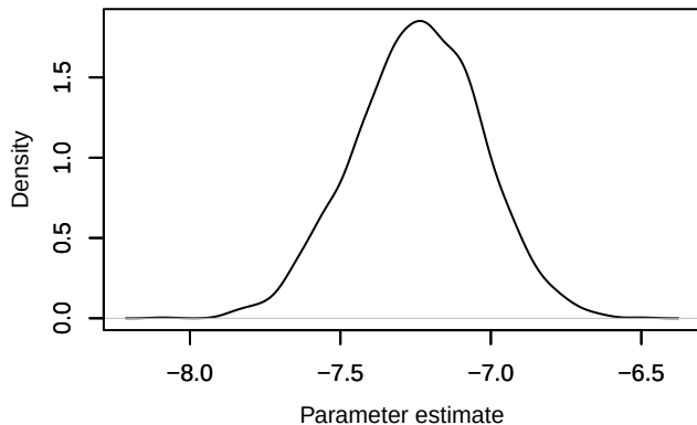
Density – loglik[171]
