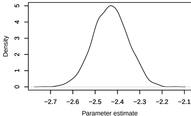
Density – loglik[148]
