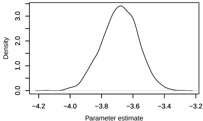
Density – loglik[277]
