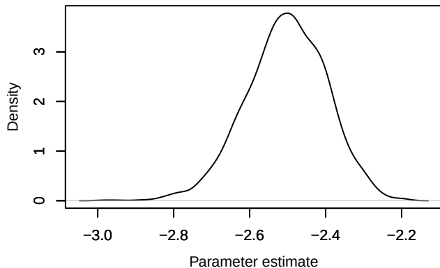
Density – loglik[349]
