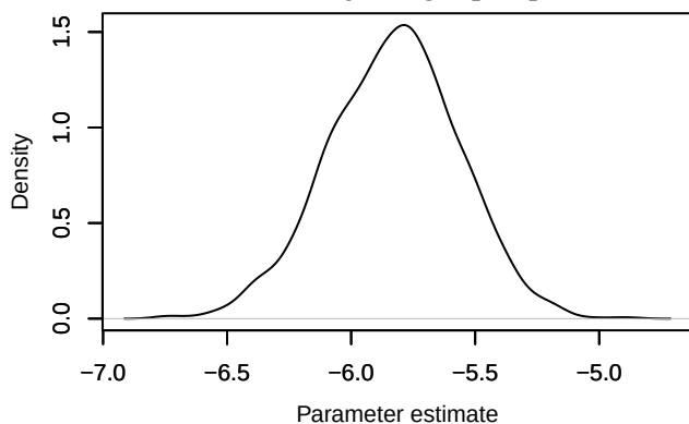
Density – loglik[390]
