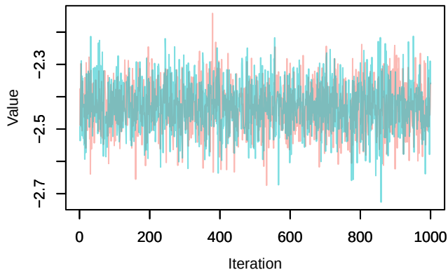
Trace – loglik[210]
