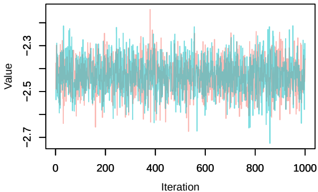
Trace – loglik[243]
