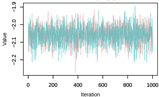
Trace – loglik[3]
