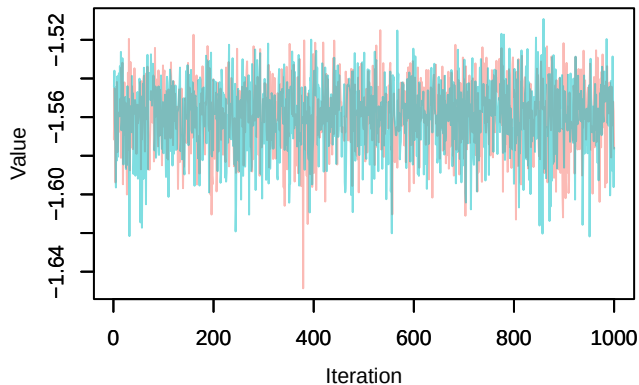
Trace – loglik[117]
