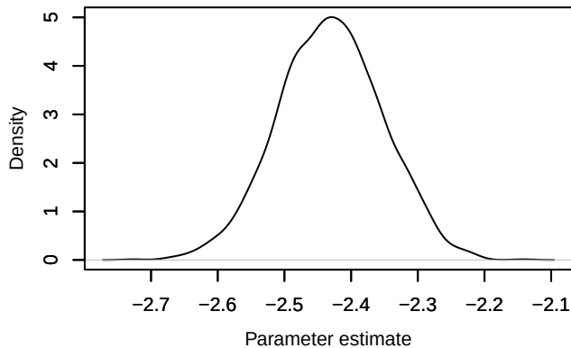
Density – loglik[279]
