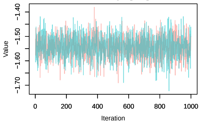
Trace – loglik[240]
