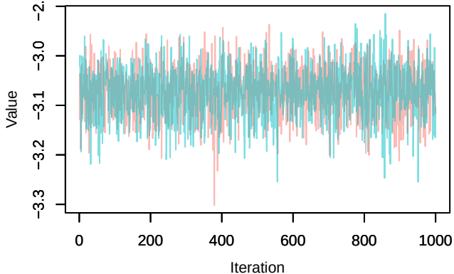
Trace – loglik[397]
