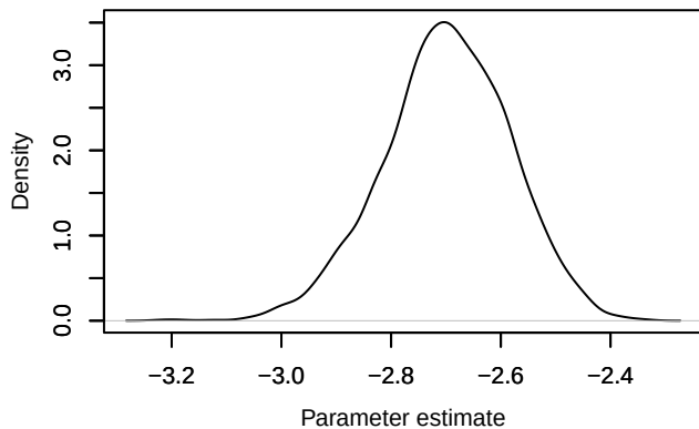
Density – loglik[343]
