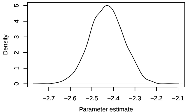
Density – loglik[133]
