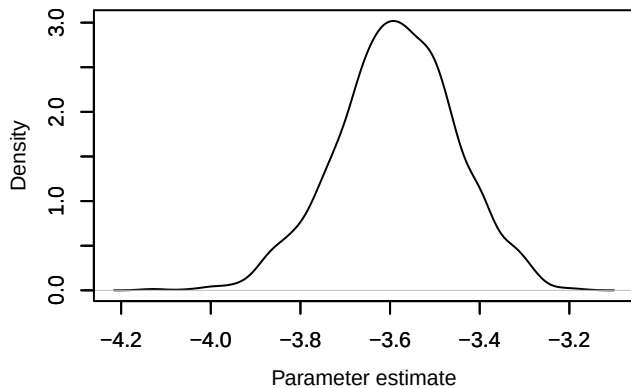
Density – loglik[366]
