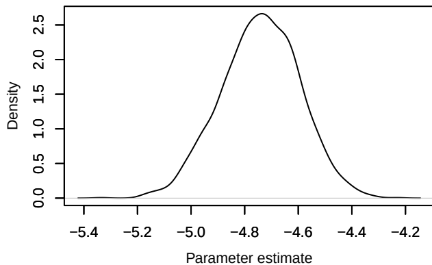
Density – loglik[235]
