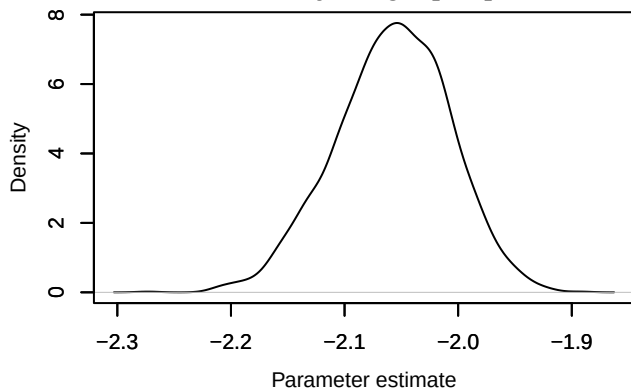
Density – loglik[174]
