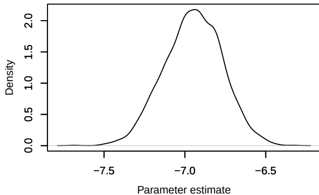
Density – loglik[315]
