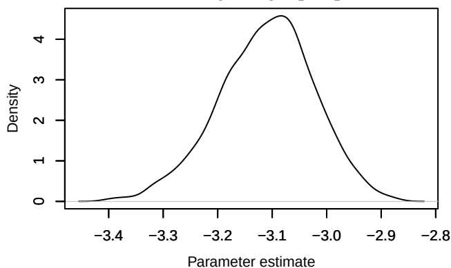
Density – loglik[355]
