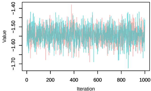
Trace – loglik[232]
