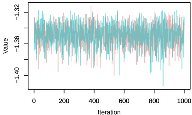
Trace – loglik[301]
