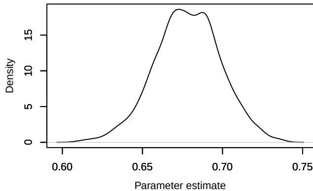
Density – p
