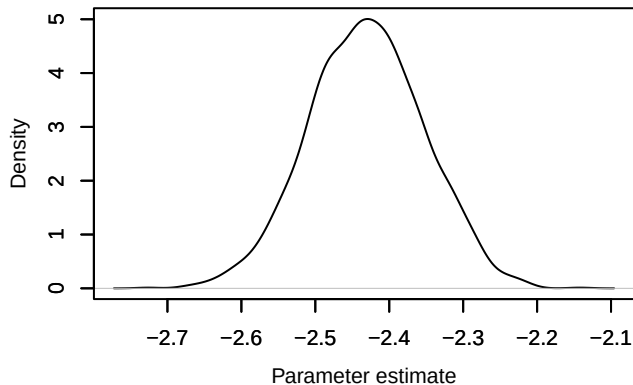
Density – loglik[210]
