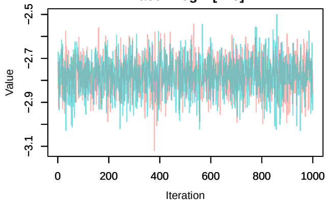
Trace – loglik[144]
