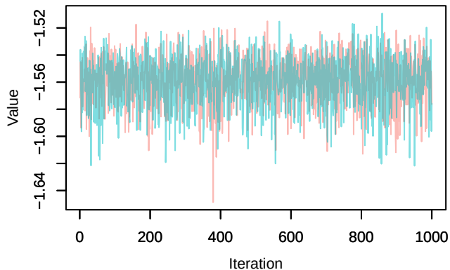
Trace – loglik[237]
