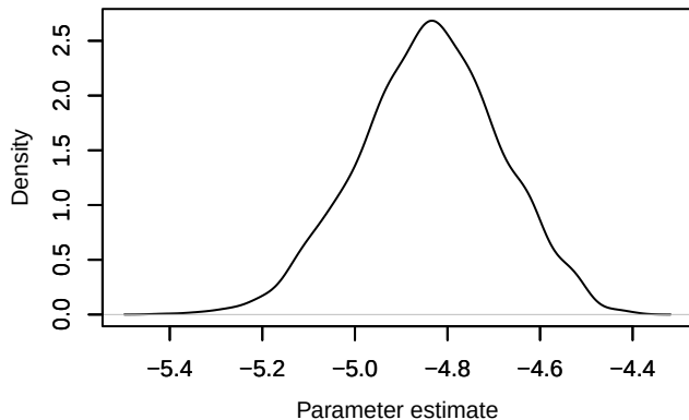
Density – loglik[399]
