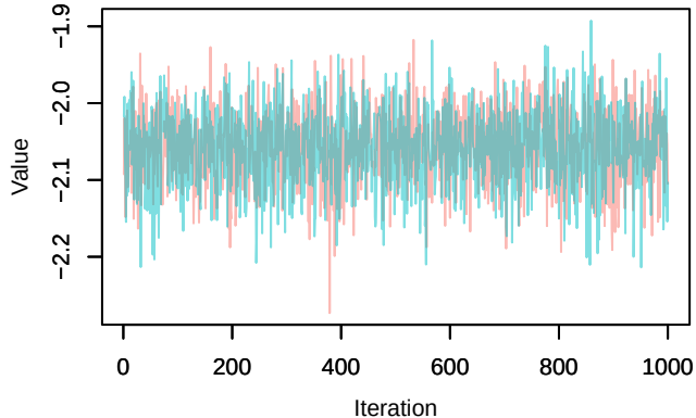
Trace – loglik[253]
