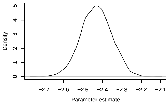
Density – loglik[267]
