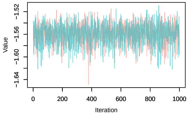
Trace – loglik[291]
