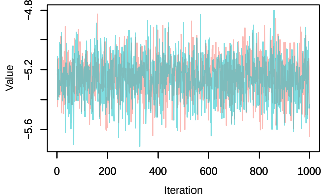
Trace – loglik[379]
