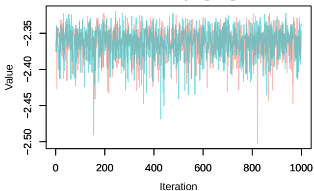
Trace – loglik[360]
