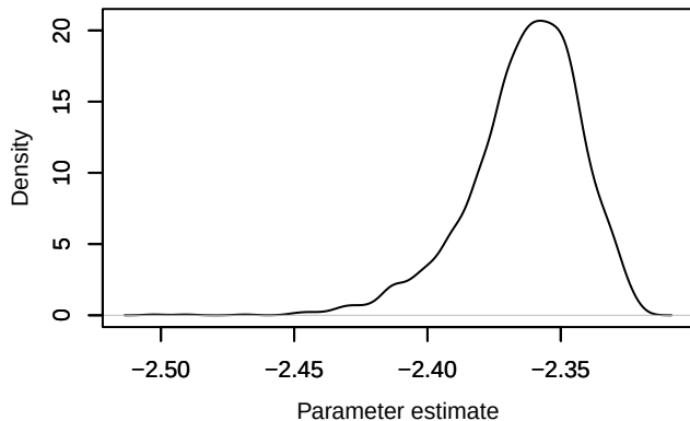
Density – loglik[348]
