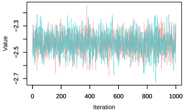
Trace – loglik[256]
