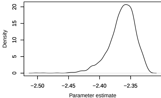
Density – loglik[346]
