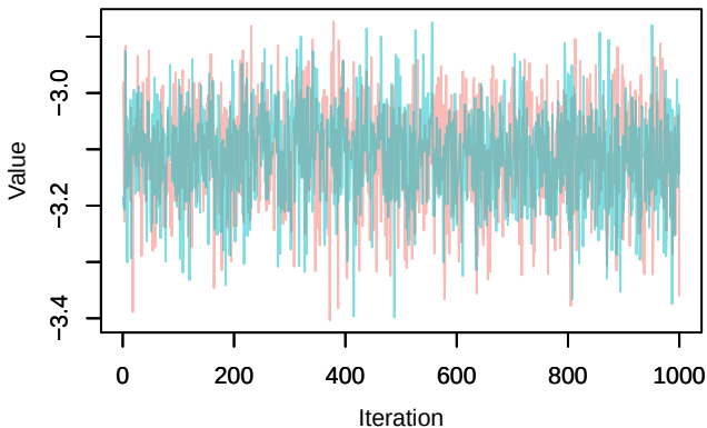
Trace – loglik[330]
