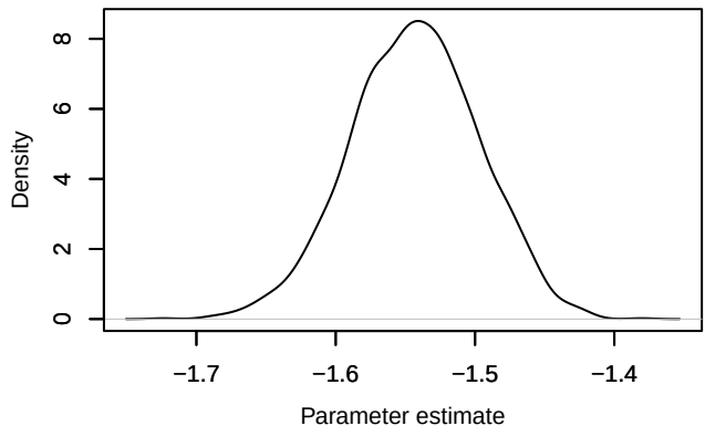
Density – loglik[22]
