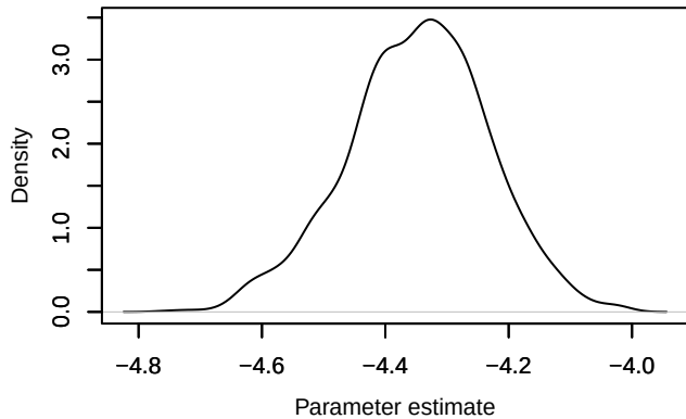
Density – loglik[346]
