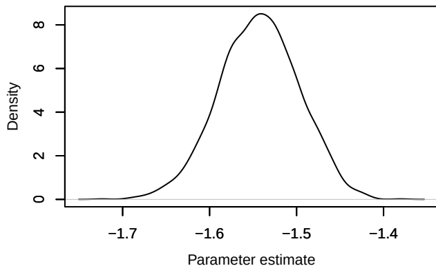
Density – loglik[226]
