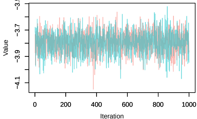
Trace – loglik[376]
