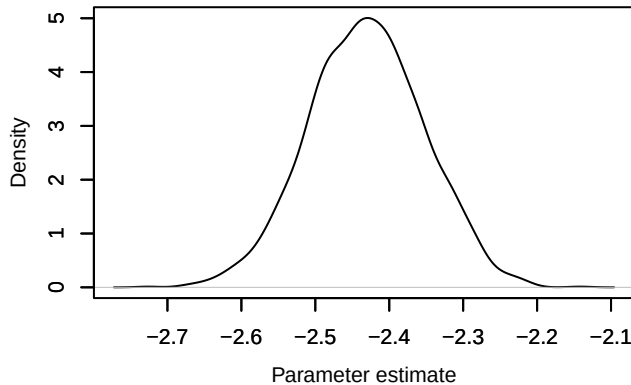
Density – loglik[256]
