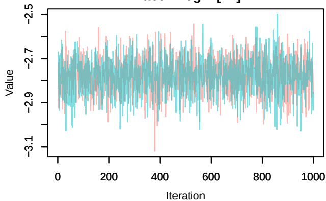
Trace – loglik[12]
