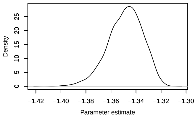
Density – loglik[268]
