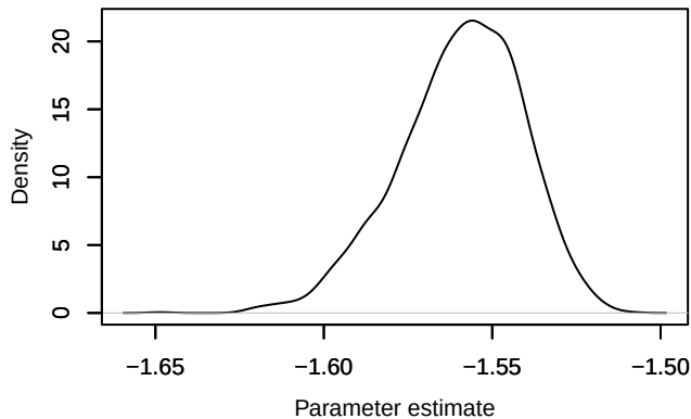
Density – loglik[105]
