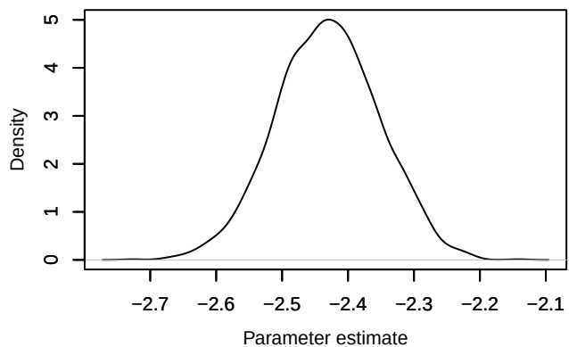
Density – loglik[10]
