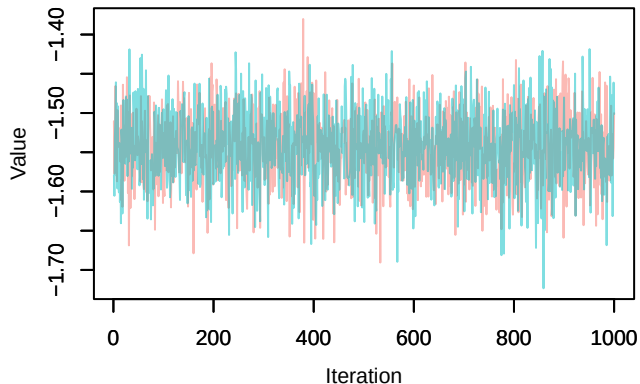
Trace – loglik[205]
