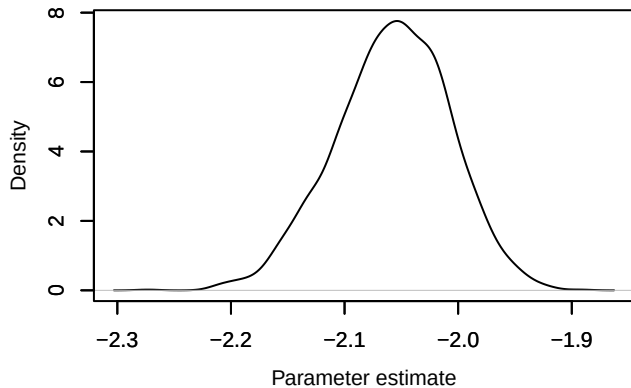
Density – loglik[151]
