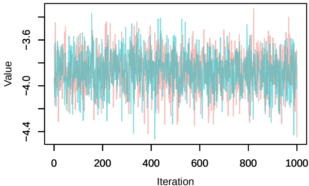
Trace – loglik[400]
