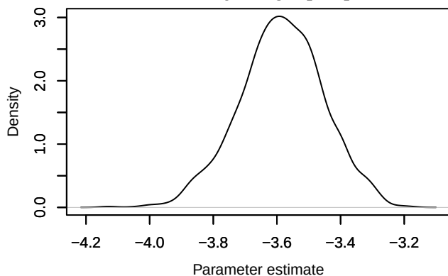
Density – loglik[321]
