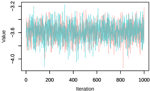
Trace – loglik[331]
