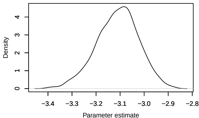
Density – loglik[372]
