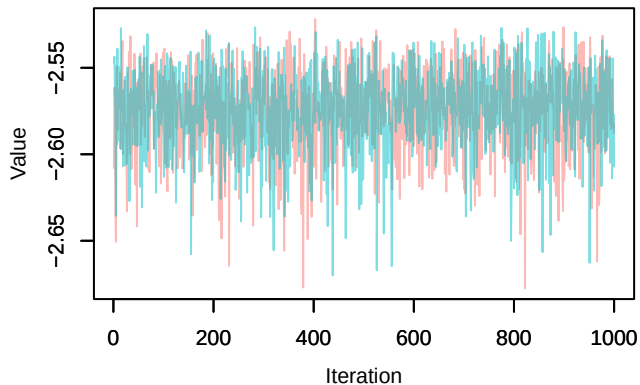
Trace – loglik[343]
