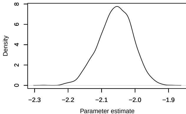
Density – loglik[250]
