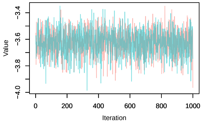
Trace – loglik[384]
