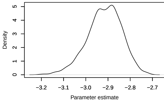
Density – loglik[325]
