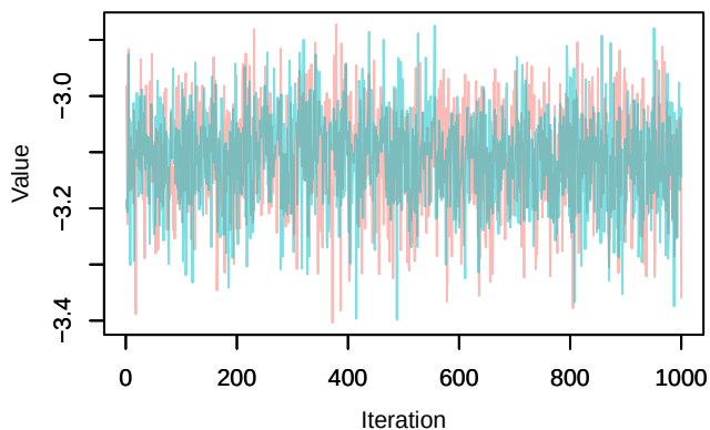
Trace – loglik[372]
