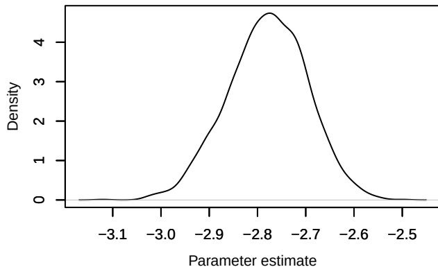
Density – loglik[157]
