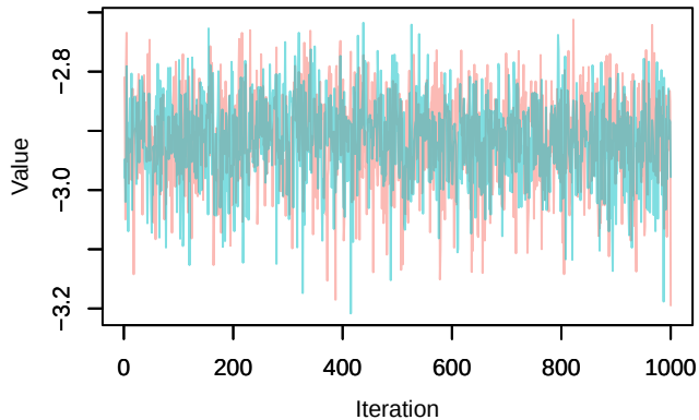
Trace – loglik[364]
