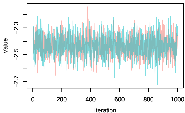
Trace – loglik[249]
