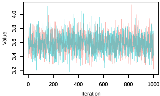
Trace – loglik[1]
