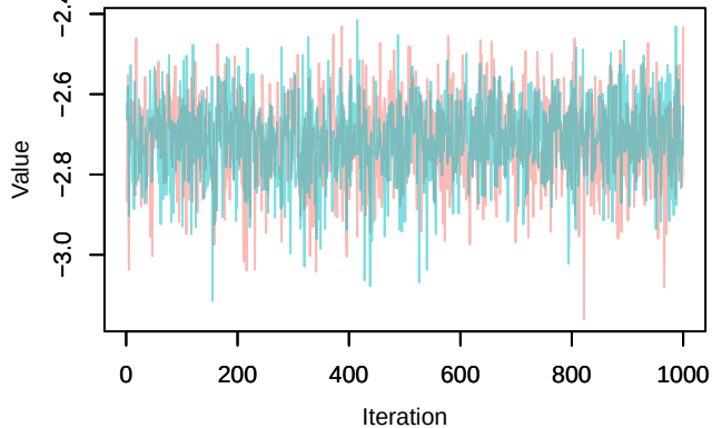
Trace – loglik[349]
