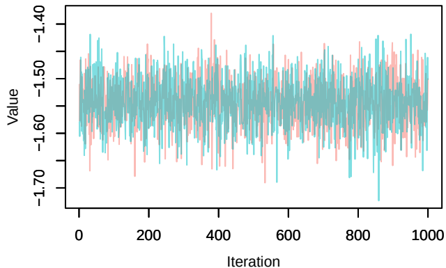
Trace – loglik[184]
