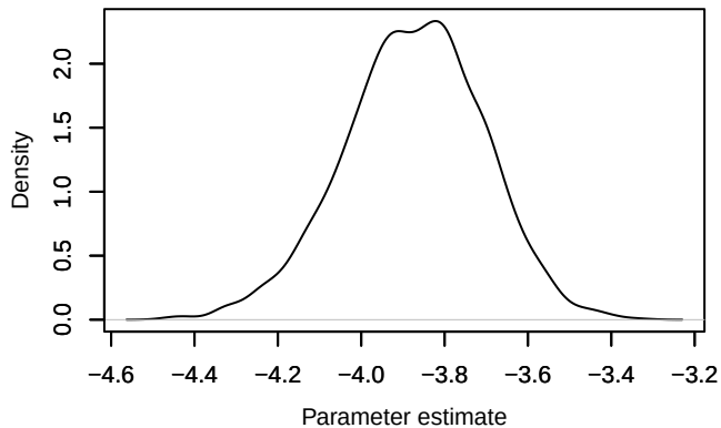
Density – loglik[387]
