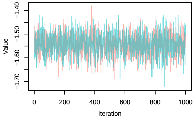
Trace – loglik[178]
