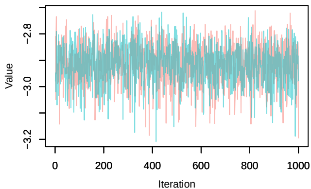
Trace – loglik[391]
