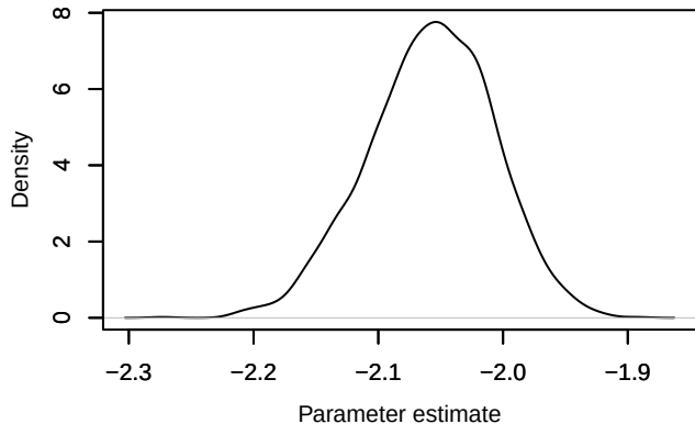
Density – loglik[178]
