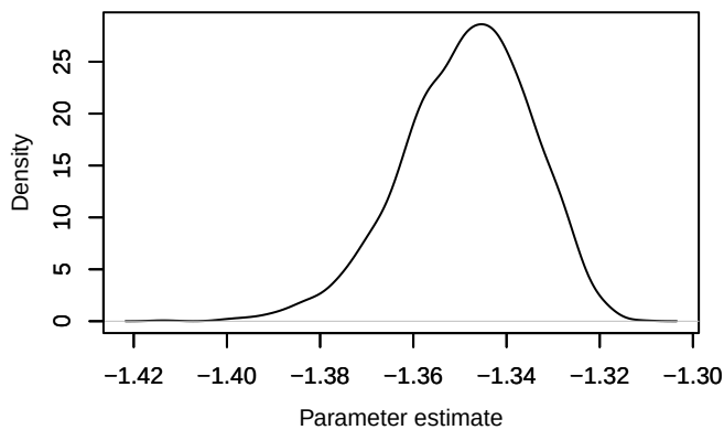
Density – loglik[127]
