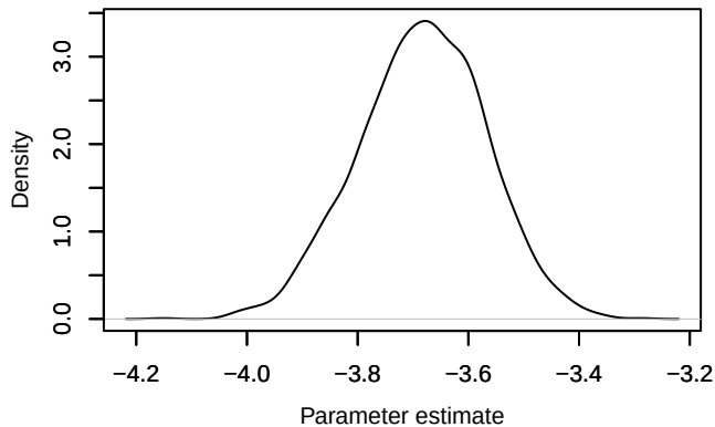
Density – loglik[201]
