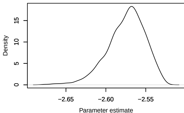
Density – loglik[340]
