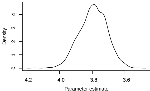
Density – loglik[316]
