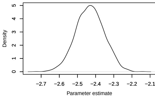
Density – loglik[46]
