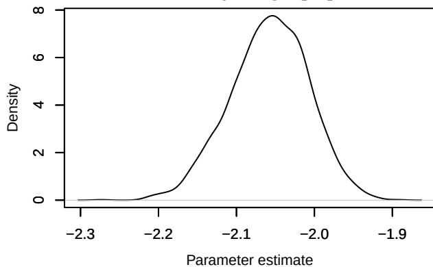
Density – loglik[18]
