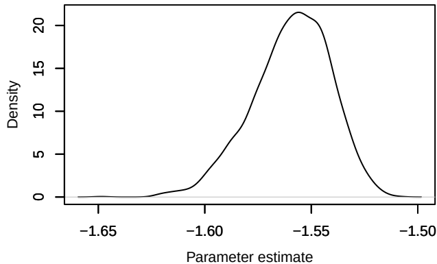
Density – loglik[193]
