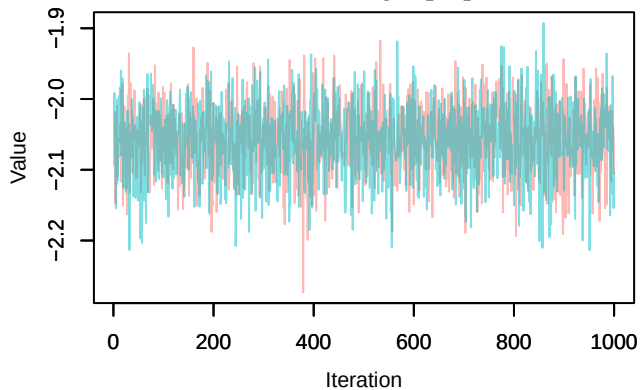
Trace – loglik[99]
