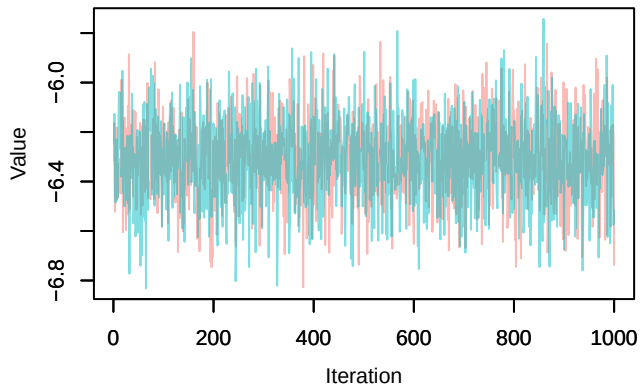
Trace – loglik[319]
