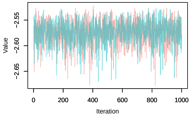
Trace – loglik[378]
