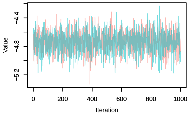
Trace – loglik[235]
