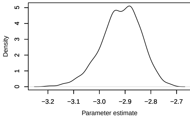
Density – loglik[357]
