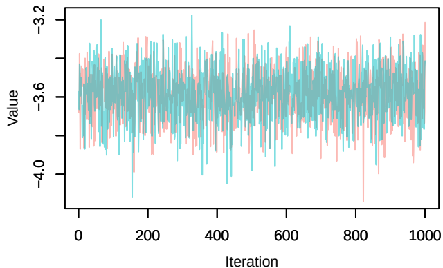
Trace – loglik[373]
