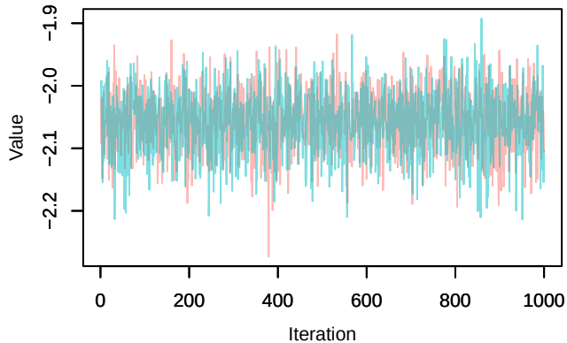
Trace – loglik[267]
