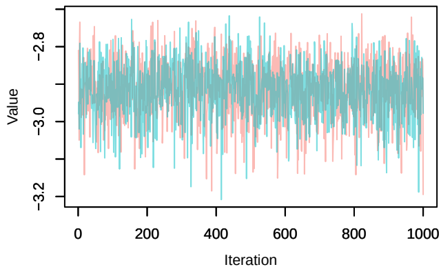
Trace – loglik[325]
