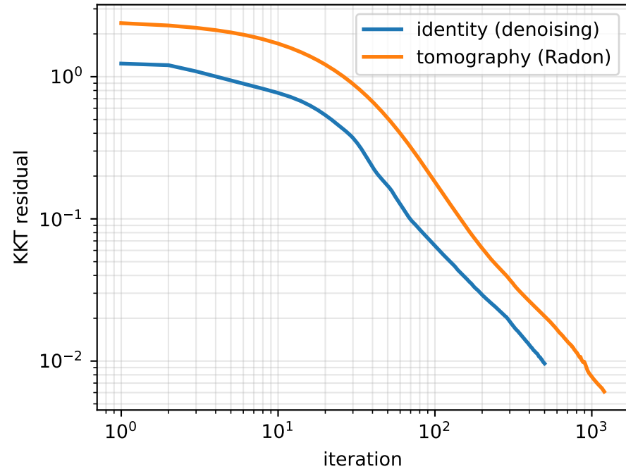
run_zero convergence (deviations = 0)
