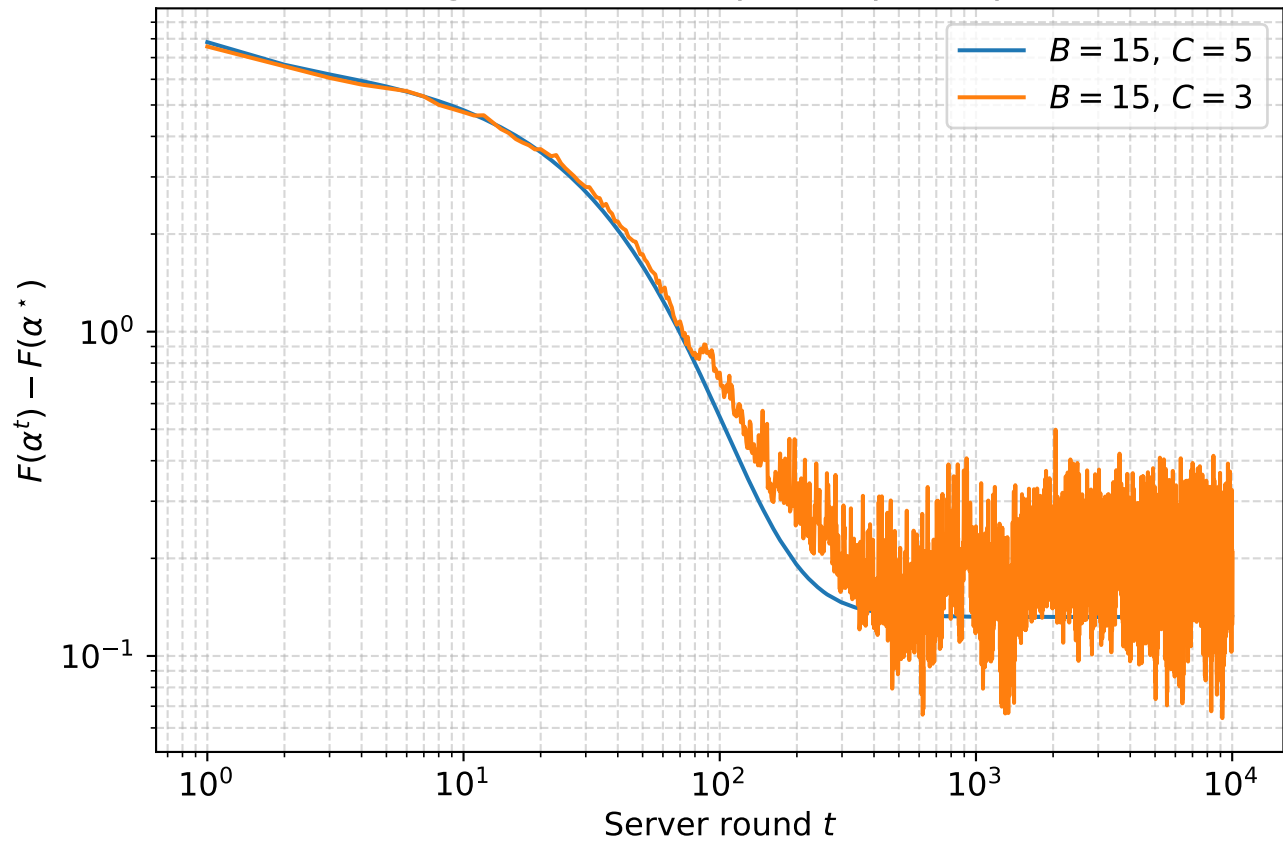
FedAvg: mini-batch / partial participation
