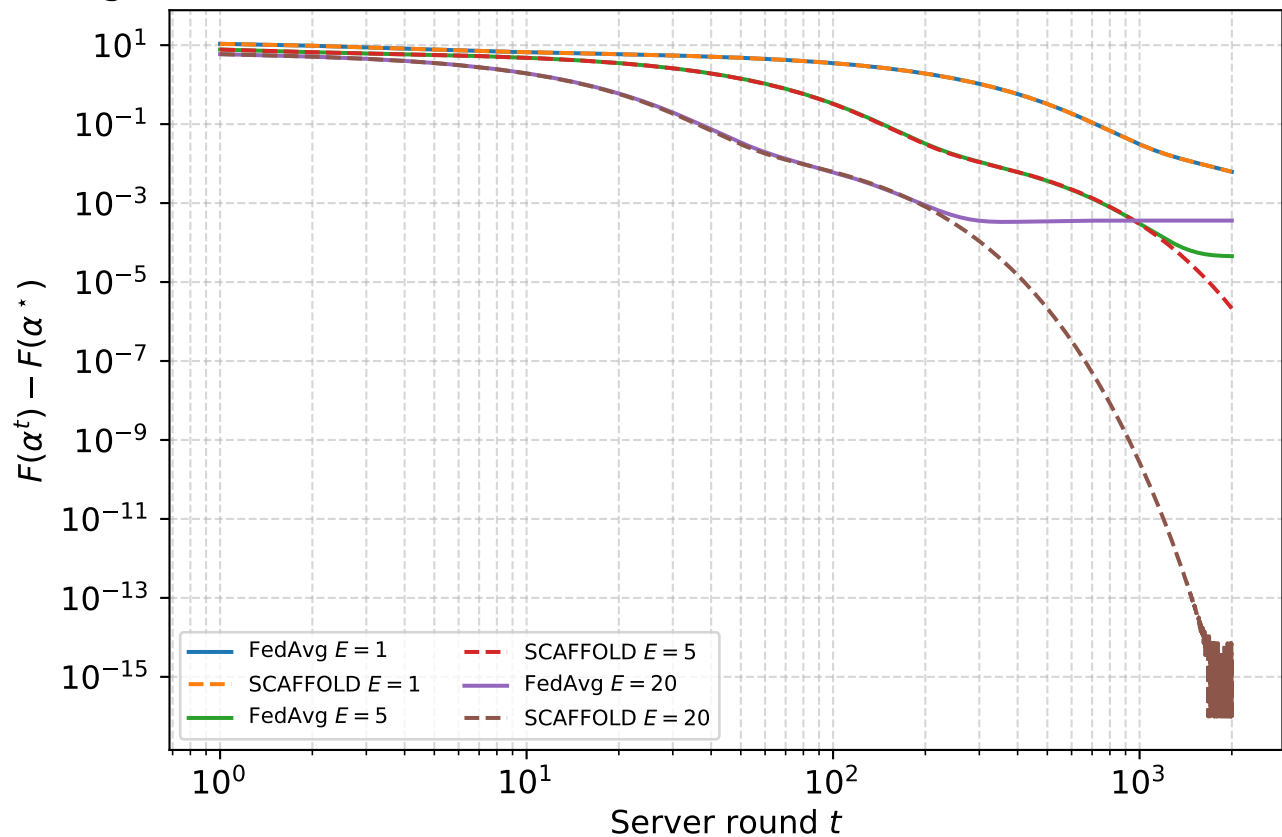
FedAvg vs. SCAFFOLD ( B = 20 , \text{lr} = 0.002 ); control variates reduce cli
