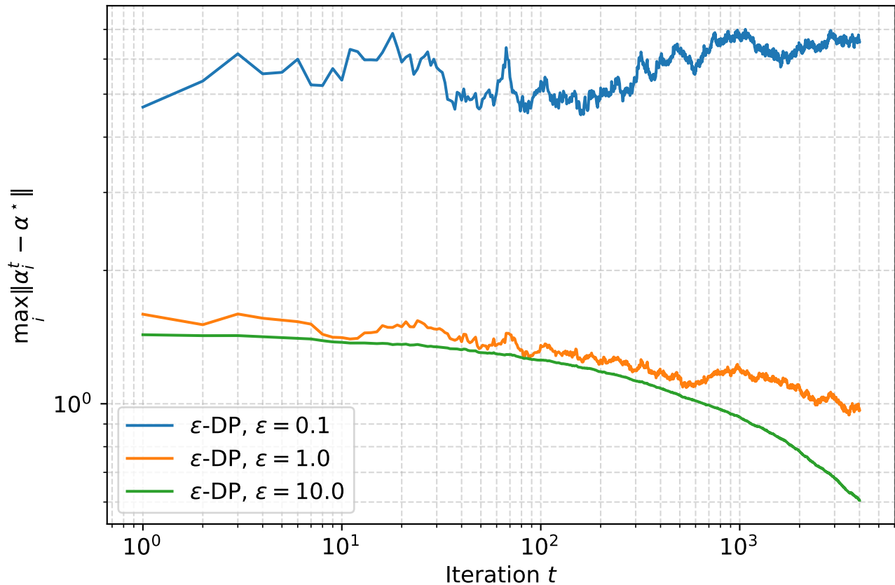
DGD with Laplacian noise (noise scale \propto 1/\varepsilon )
