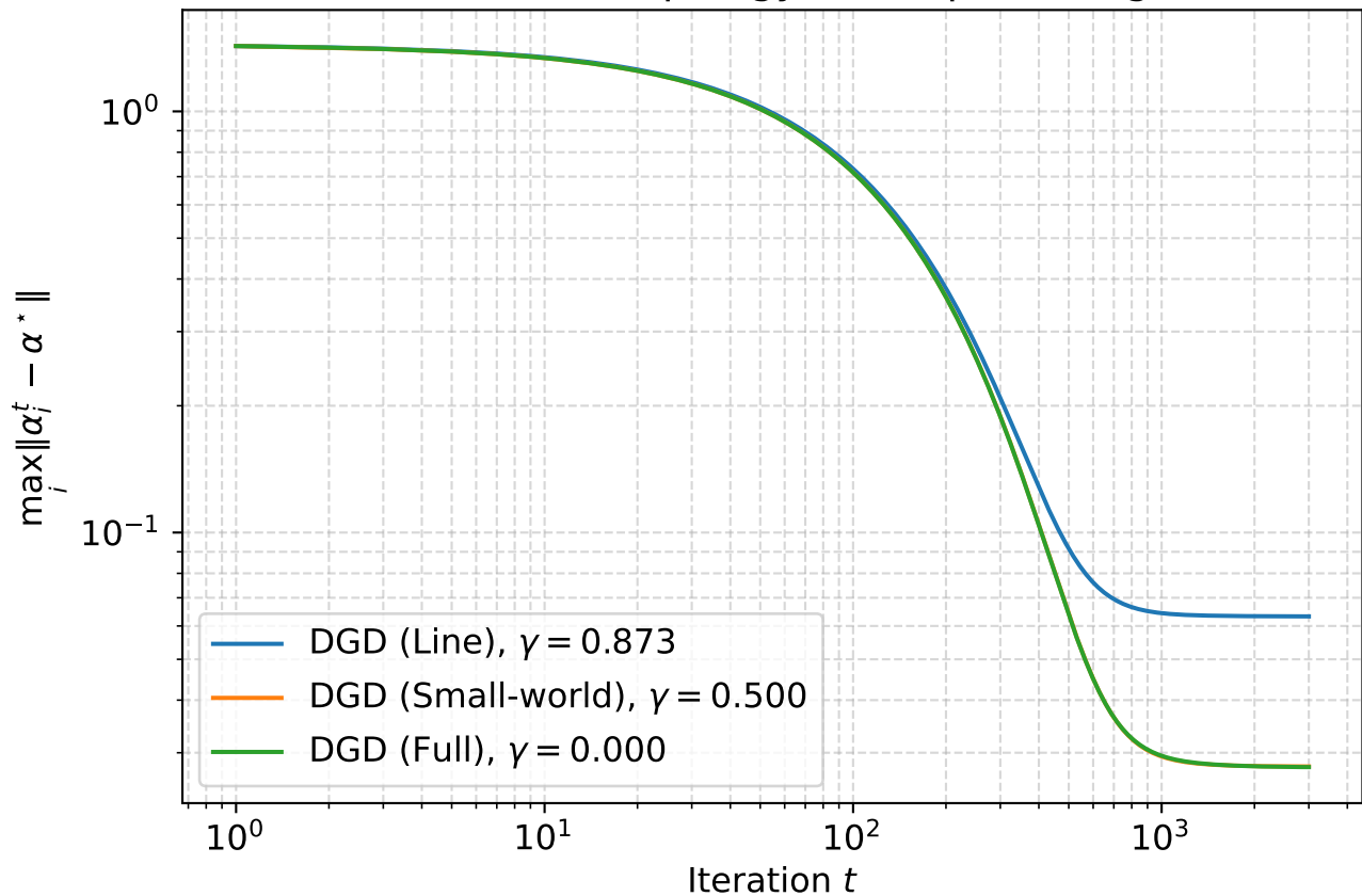
DGD: effect of topology (Metropolis weights)
