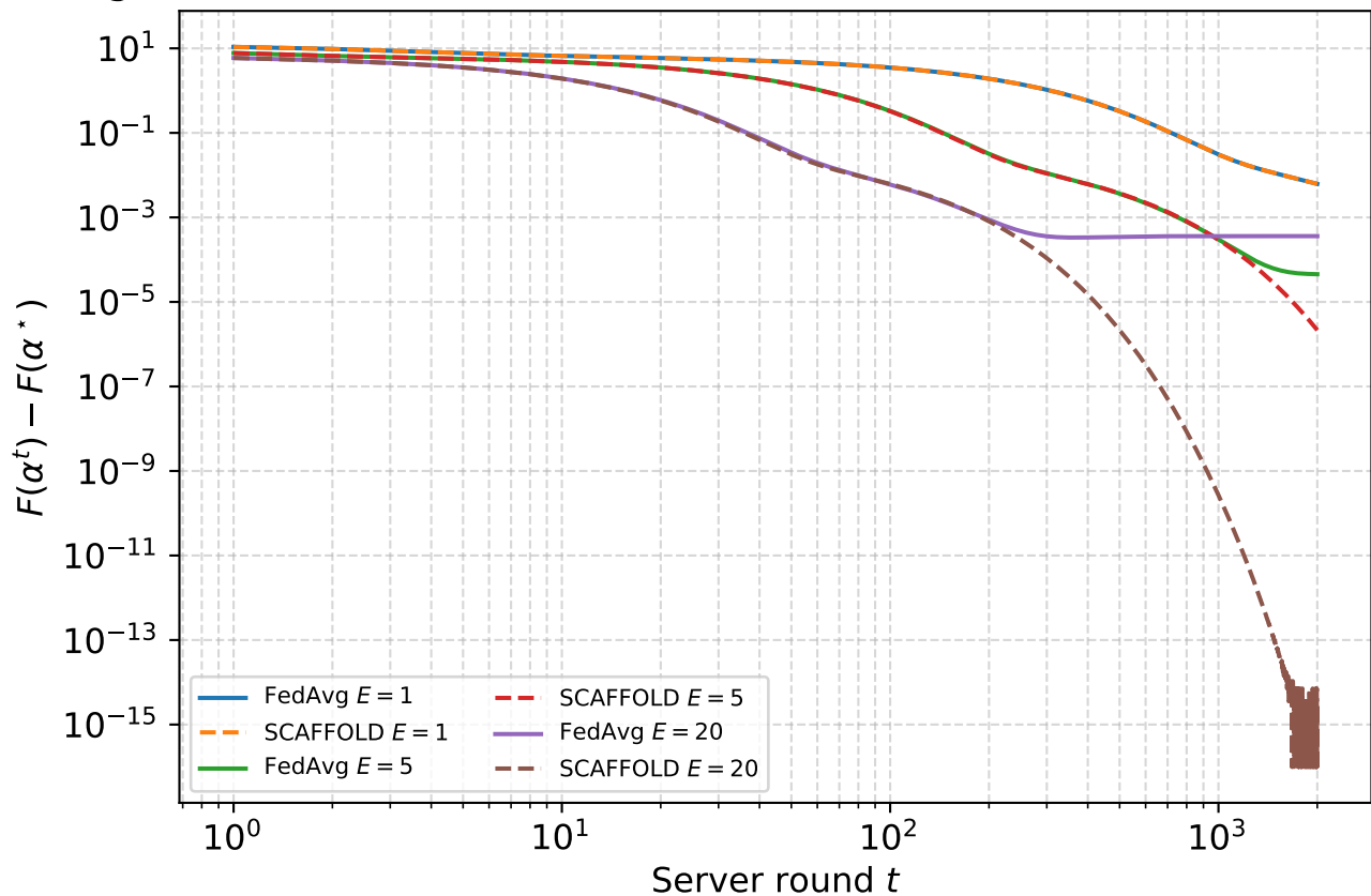
FedAvg vs. SCAFFOLD ( B = 20 , \text{lr} = 0.002 ); control variates reduce cli
