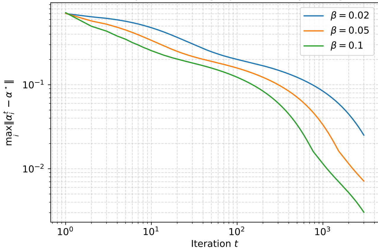
ADMM vs. \beta (stable range; \beta \gtrsim 0.15 may diverge)
