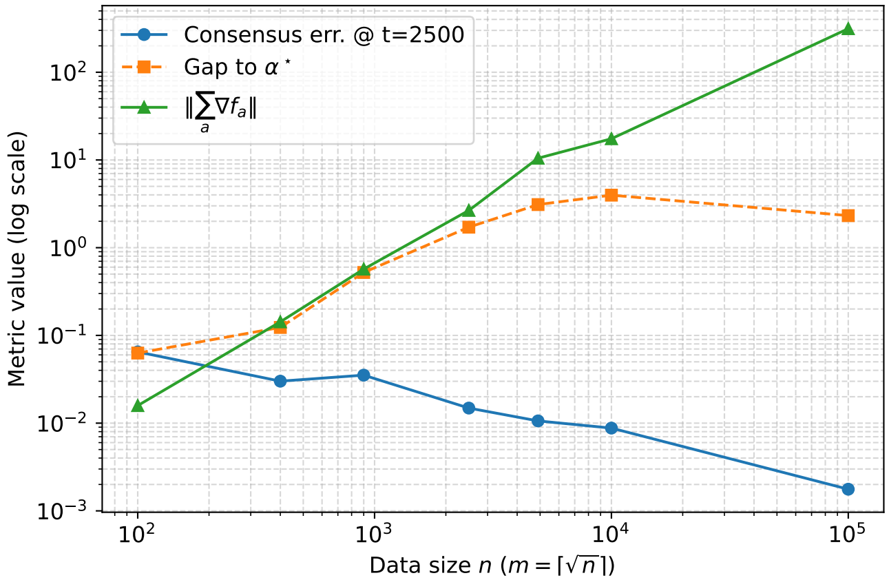
DGD scaling: larger n increases local problem size m ; fixed iterations
