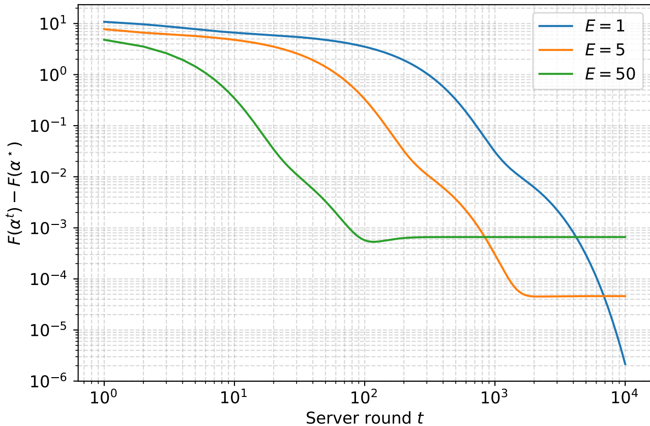
FedAvg: B = 20 , C = 5 , constant \text{lr} = 0.002
