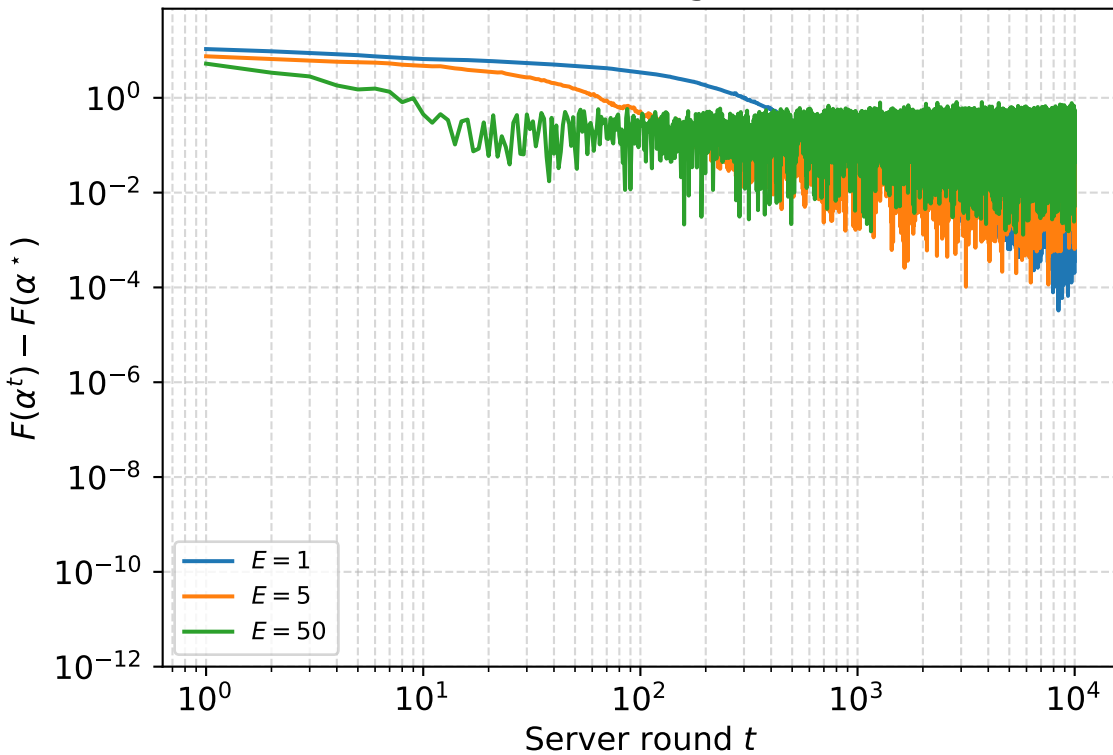
FedAvg
