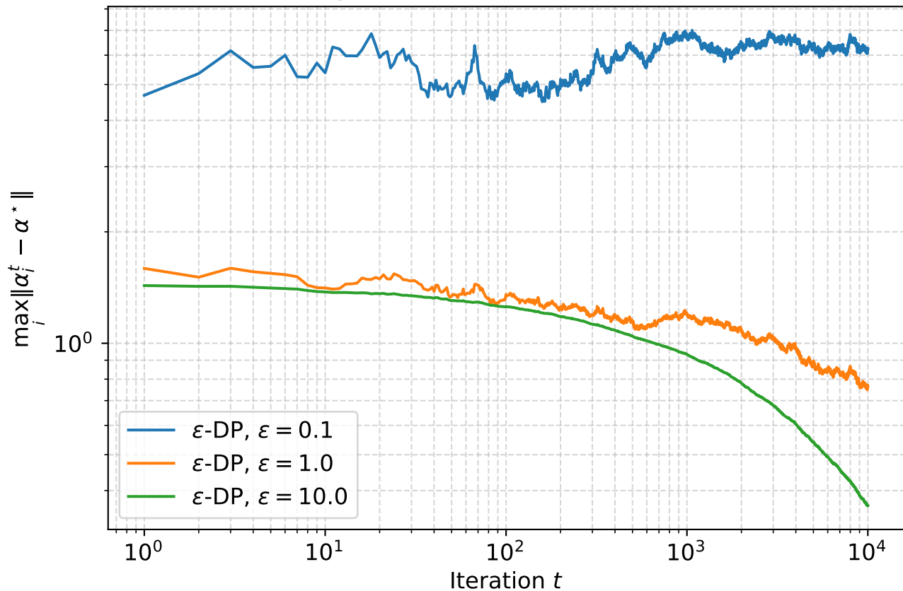
DGD with Laplacian noise ( n = 100, m = 10, a = 5 )
