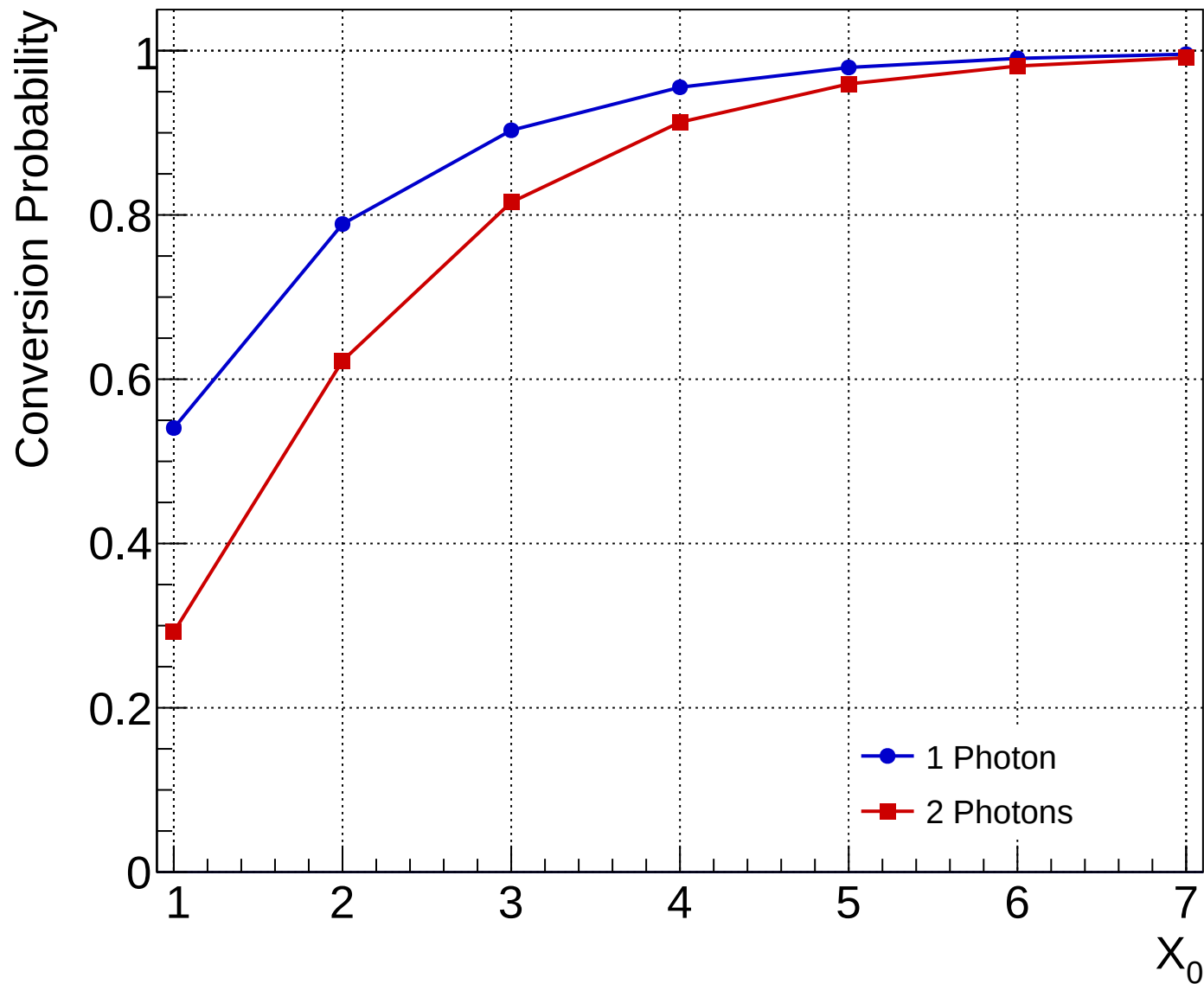
Photon Conversion Probability vs Material Thickness
