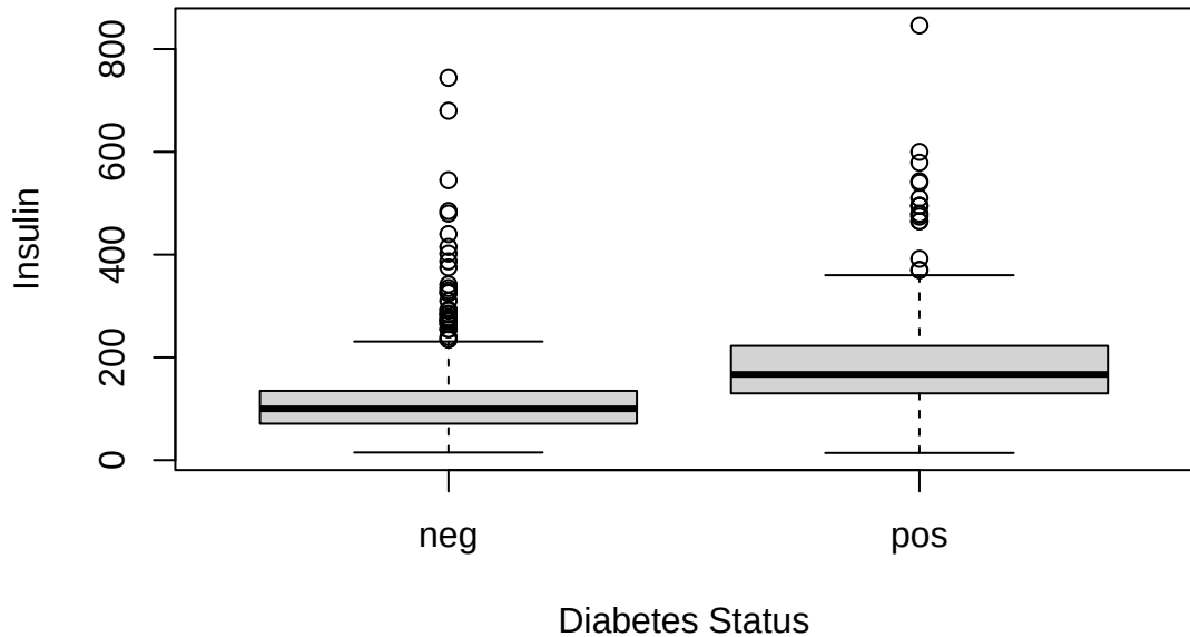
Boxplot of Insulin by Diabetes Status
