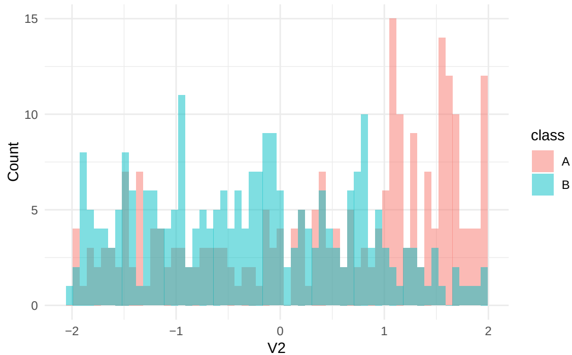
Histogram of V2 by Class
