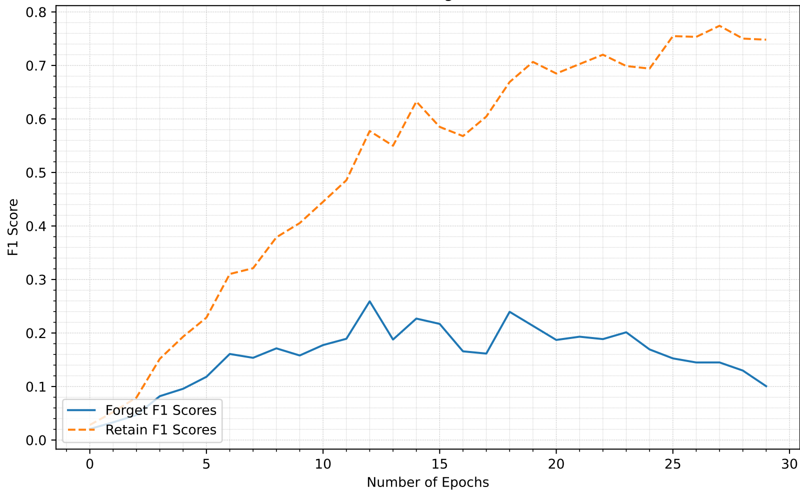
MIA F1 Score as the Target Model Unlearns
