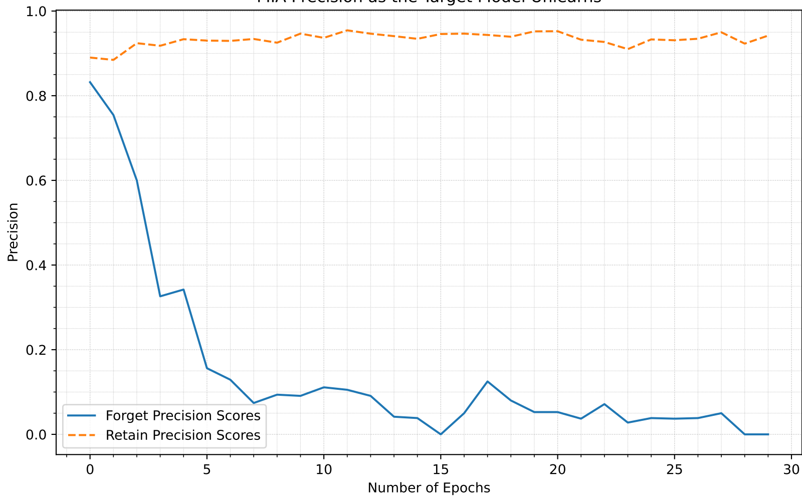
MIA Precision as the Target Model Unlearns
