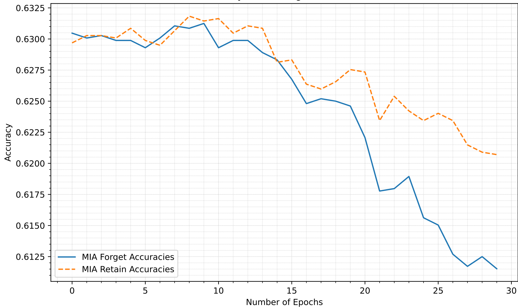
MIA Accuracy as the Target Model Unlearns
