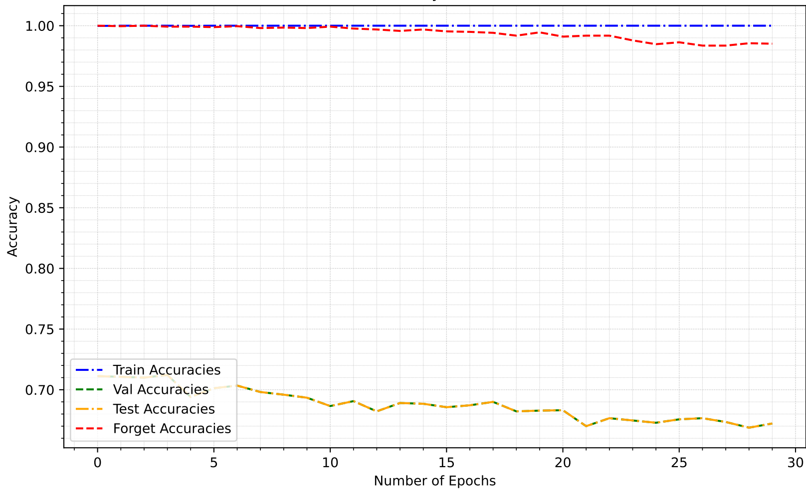
Accuracy Curves
