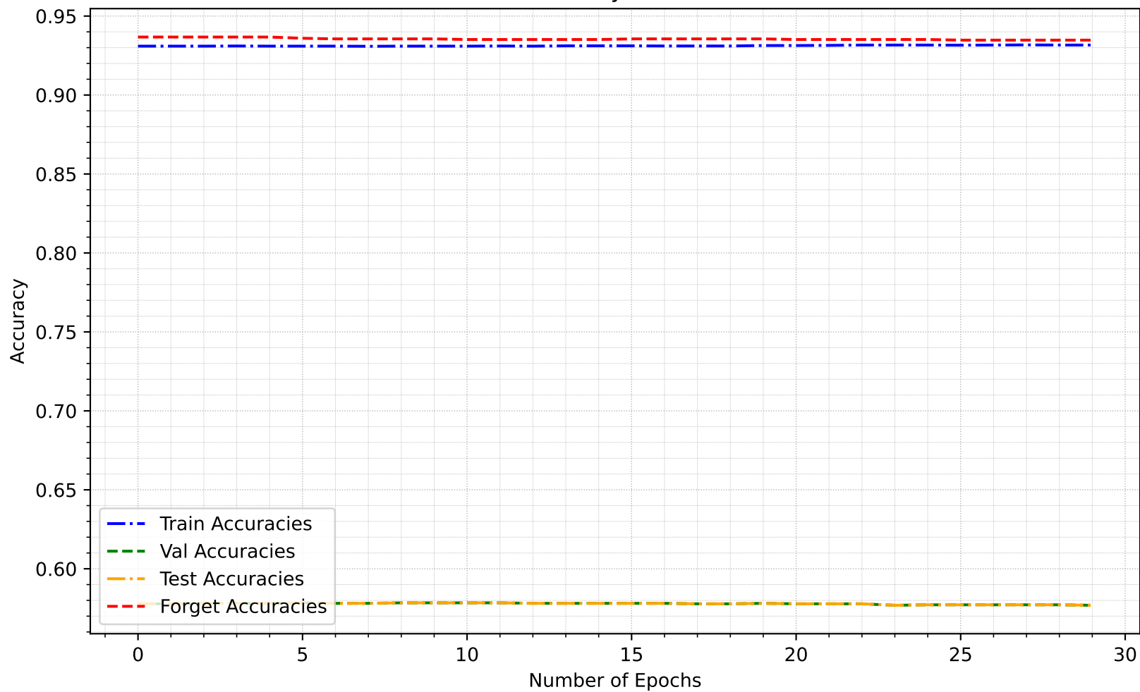
Accuracy Curves
