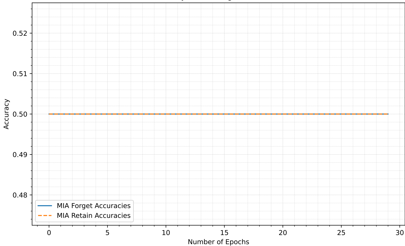
MIA Accuracy as the Target Model Unlearns
