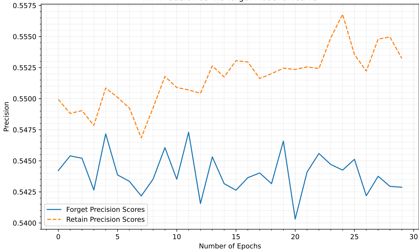
MIA Precision as the Target Model Unlearns
