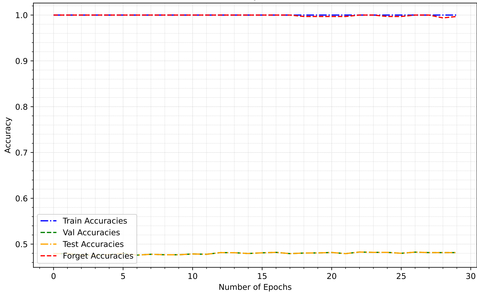
Accuracy Curves
