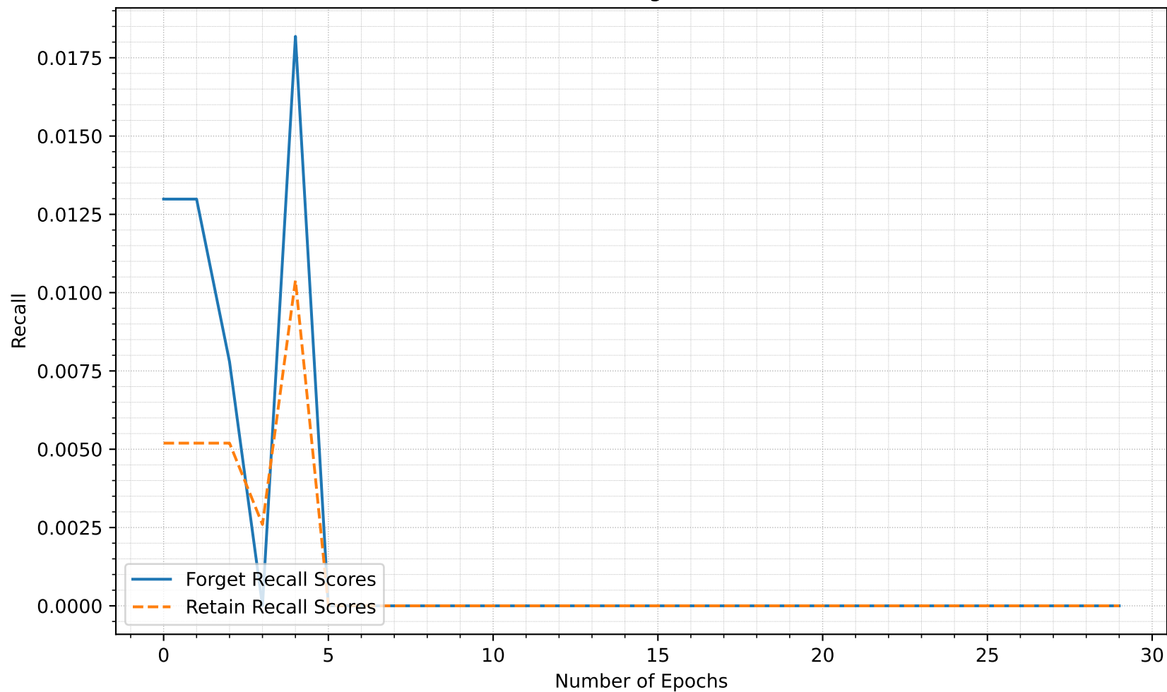
MIA Recall as the Target Model Unlearns
