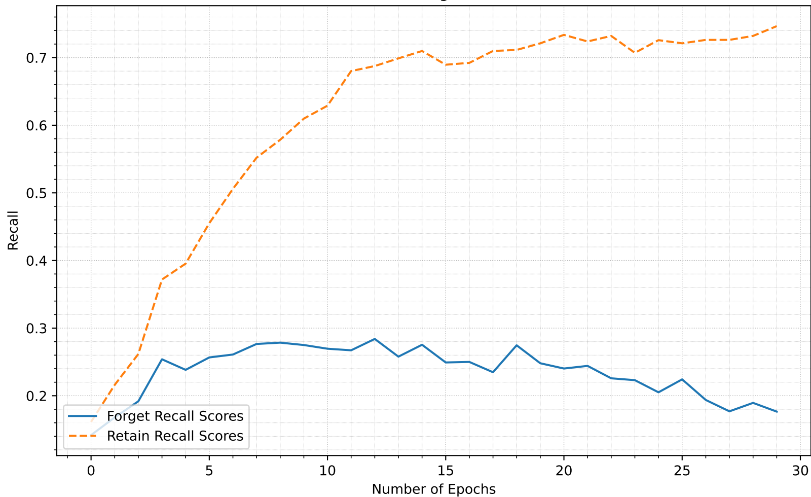
MIA Recall as the Target Model Unlearns
