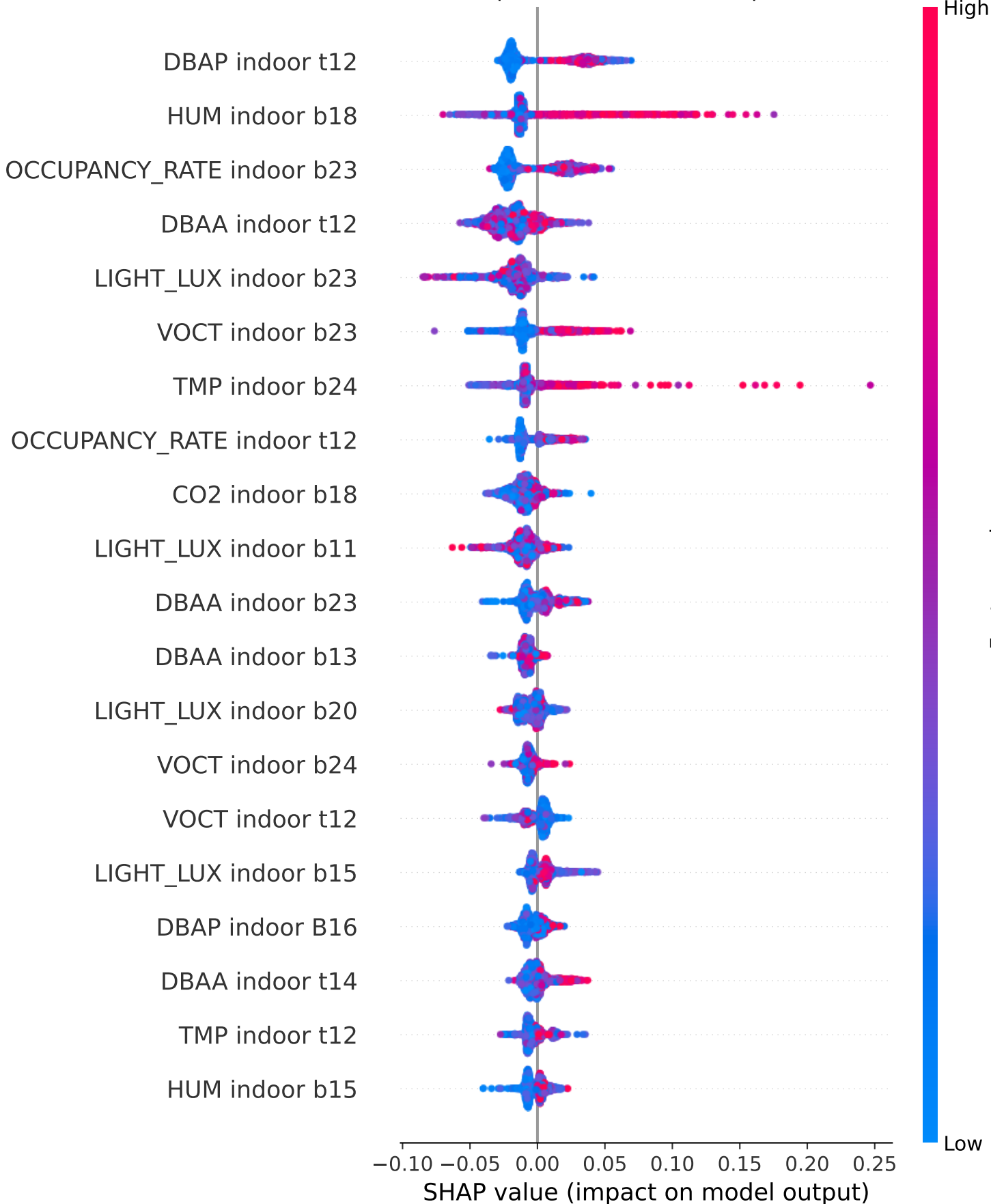
Owen / Grouped SHAP Values (Collapsed Over Time)
