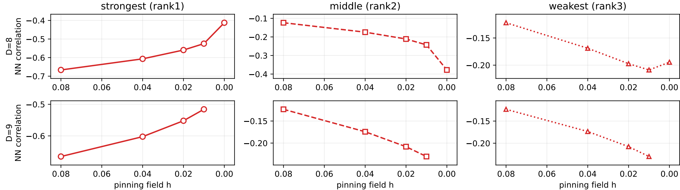
Izar replica 1, J_2=0.29 , dimer source: one rank per panel (independent vertical scales)
