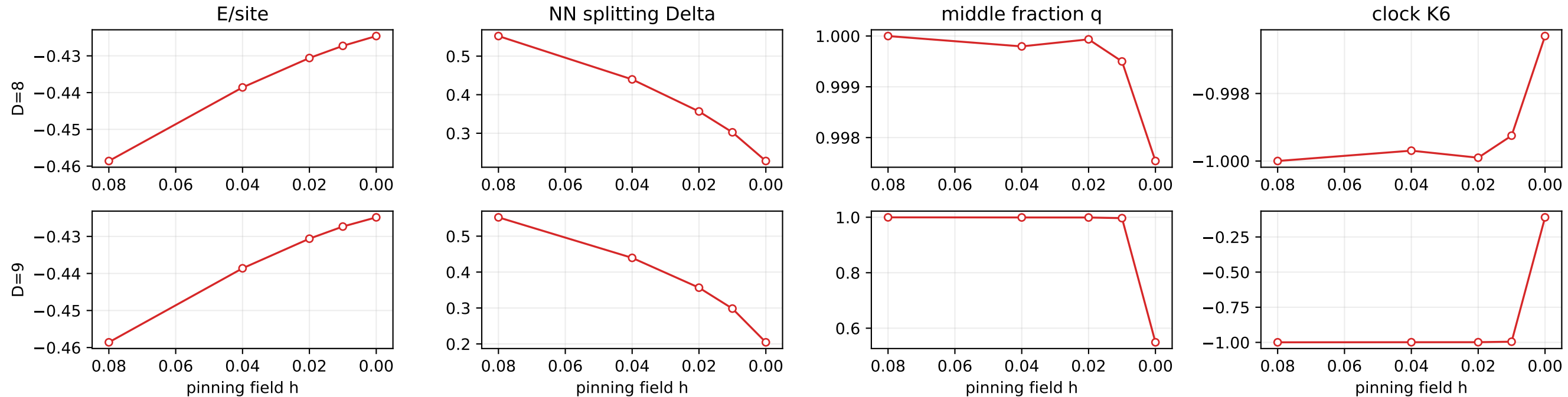
Izar replica 1, J_2=0.30 , dimer source: available optimization endpoints versus h
