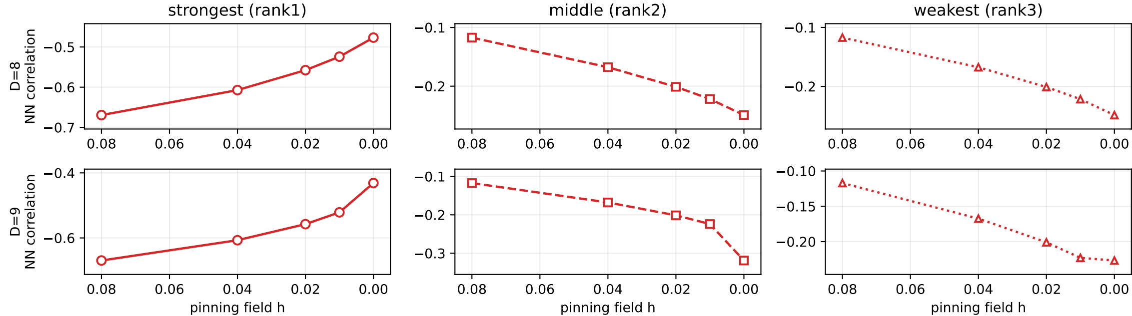
Izar replica 1, J_2=0.30 , dimer source: one rank per panel (independent vertical scales)
