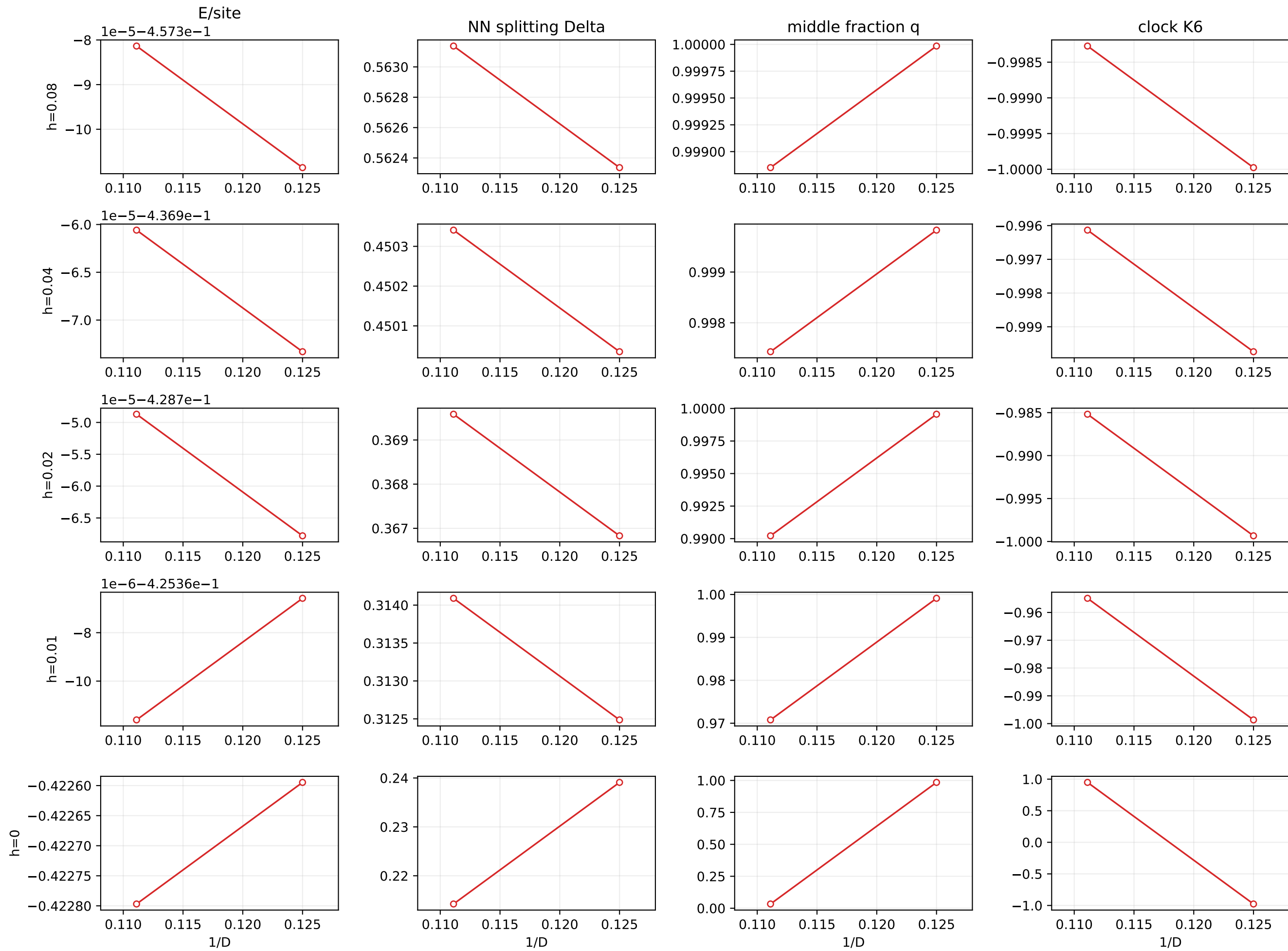
Izar replica 1, J2=0.31, dimer source: fixed-h trends; only h=0 energy is unbiased
