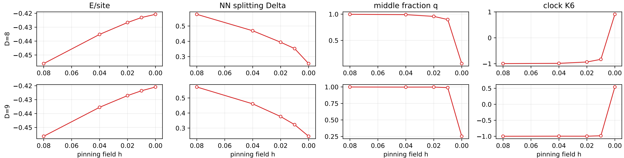
Izar replica 1, J_2=0.32 , dimer source: available optimization endpoints versus h
