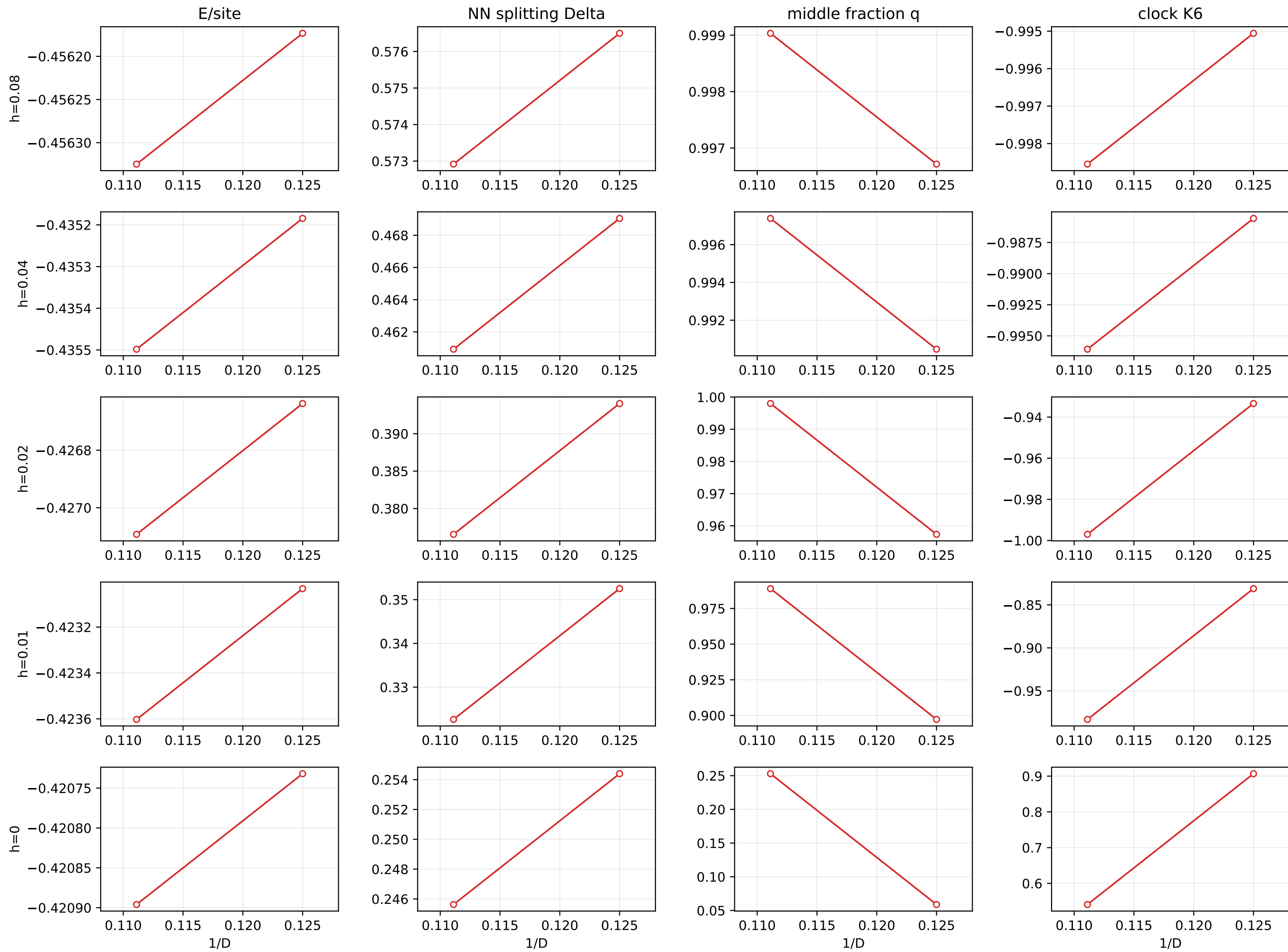
Izar replica 1, J2=0.32, dimer source: fixed-h trends; only h=0 energy is unbiased
