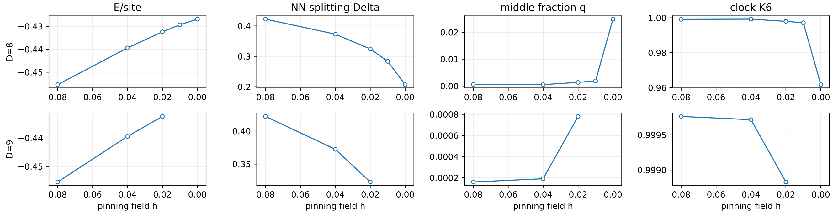
Izar replica 1, J_2=0.29 , plaquette source: available optimization endpoints versus h
