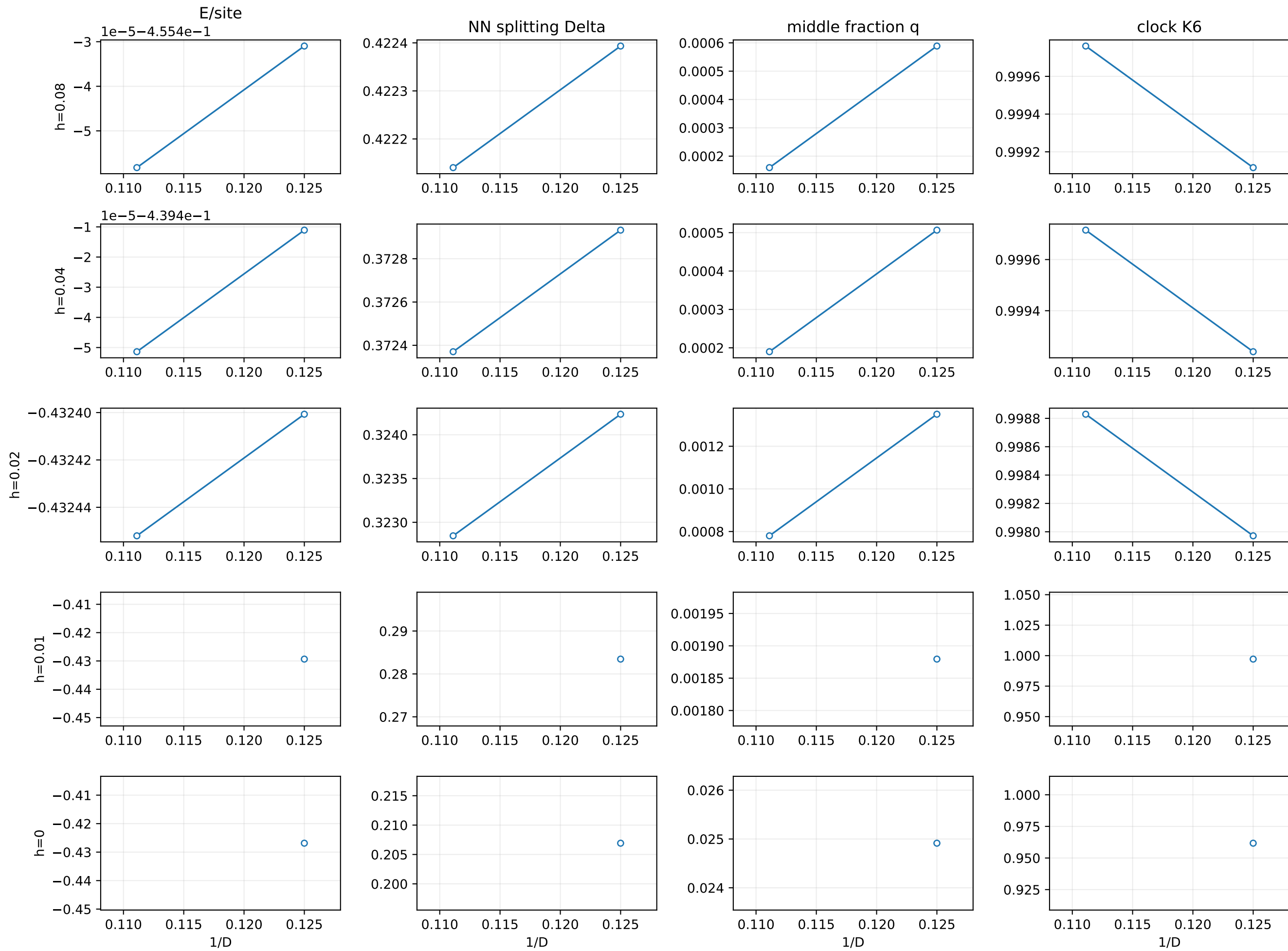
Izar replica 1, J2=0.29, plaquette source: fixed-h trends; only h=0 energy is unbiased
